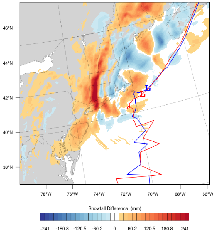
Figure 1: Storm total snowfall depth difference (mm) between two simulations of the 26–29 January 2015 Nor'easter using BL scheme variants that differ with respect to vertical moisture mixing. Bold "L"s represent cyclone center locations at 0600 UTC 28 January 2015 and solid lines denote cyclone tracks.
