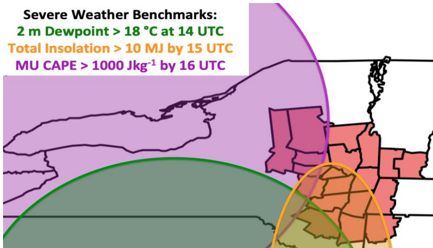
Figure 3: Potential data fusion product. In this hypothetical case, severe weather in the ALY WFO (highlighted in pink) would be most dependent on benchmark values of parameters available in the model guidance. The parameters, and their location- and time-dependence, would be unique to each forecast.
