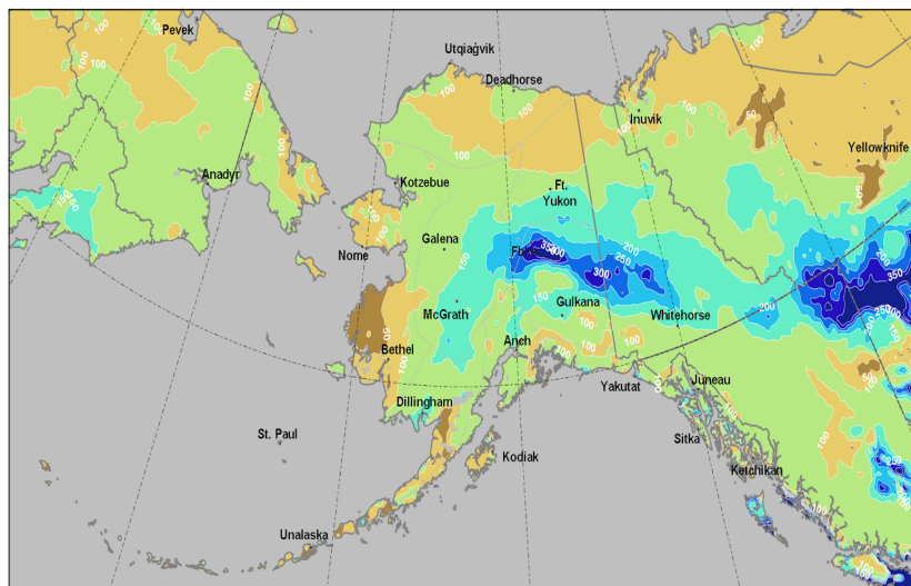
Snow Water Equivalent Percent of Median April 2022
