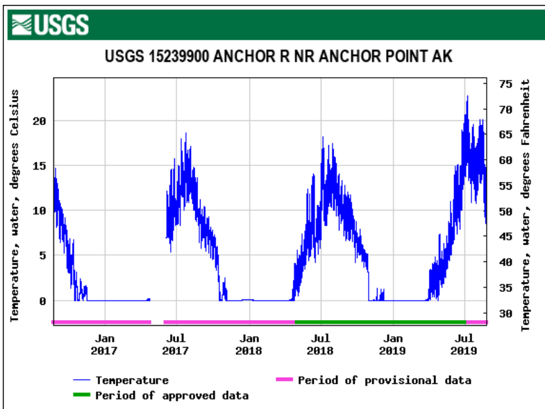
Figure 2: Water temperature data from Anchor River since 2016.
