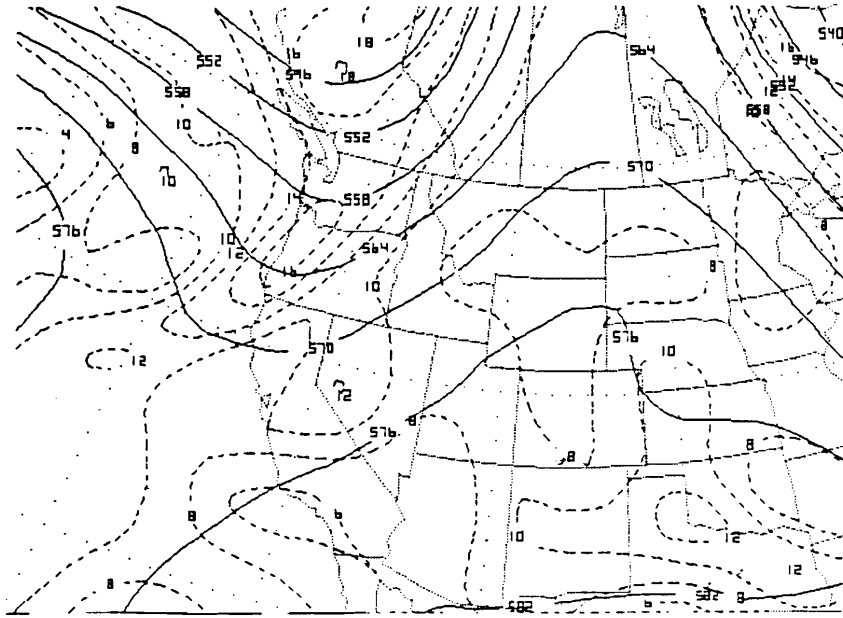
Figure 2. NGM 06 hour forecast of 500 mb geopotential height (solid) and absolute vorticity (dashed) valid at 1800 UTC 27 May 1994. Heights in dam at 60 m intervals. Vorticity at 2 \times 10^{-5} \text{ s}^{-1} .
