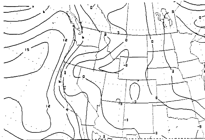
Figure 4. NGM 06 hour forecasted lifted indices valid at 1800 UTC 27 May 1994. Contoured in 3° intervals.
