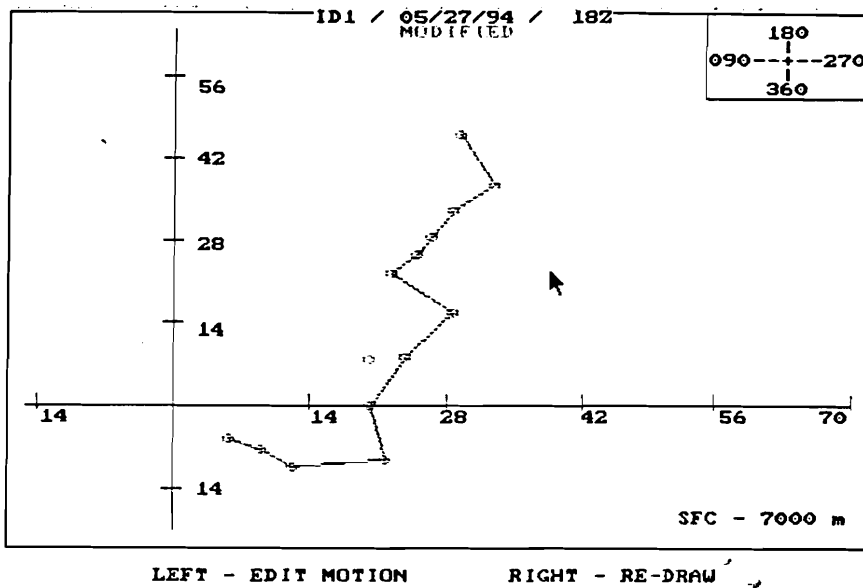
Figure 6. Hodograph at 1800 UTC 27 May 1994 for southwest corner of Idaho. Speeds are in knots. Vertical intervals (marked by open circles) are 0.5 Km apart starting at 0.8 Km at surface, then 1.0, 1.5, 2.0, etc. The first two levels can be ignored since surface is above these levels (Boise sounding was used as first guess).
