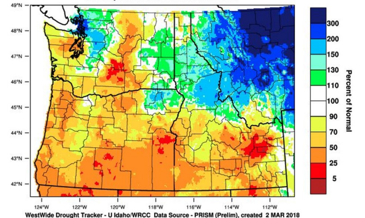
Pacific Northwest - Precipitation February 2018 Percent of 1981-2010 Normal
