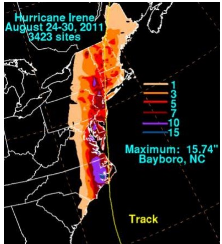
Irene's rainfall totals (inches)
