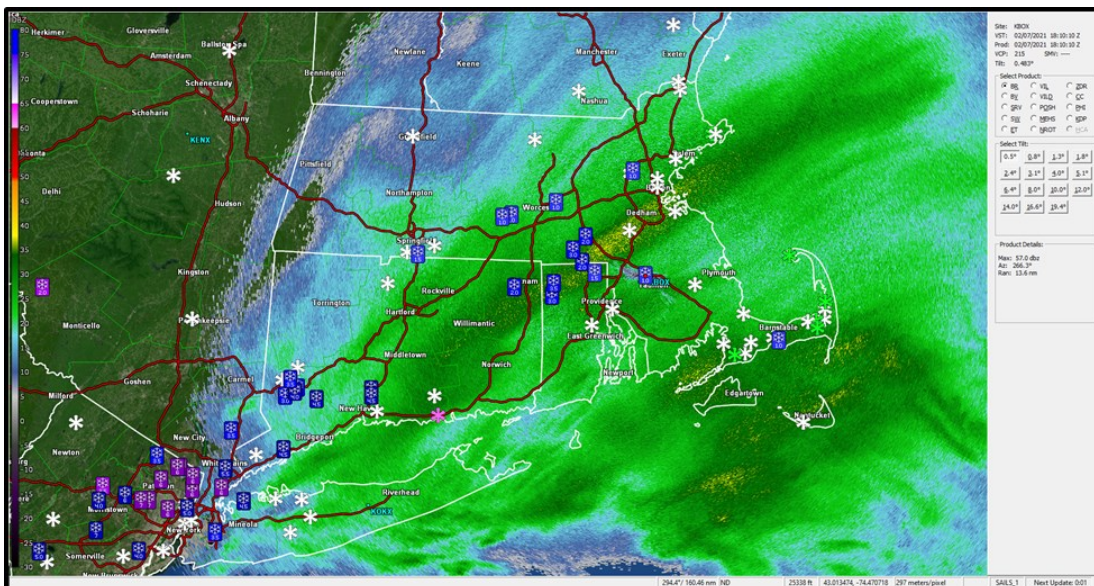
Radar image showing the band of heavy snow from CT into northern RI and eastern MA
