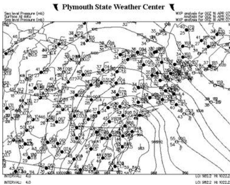
Figure 3. Surface analysis valid 00z April 16, 2007
