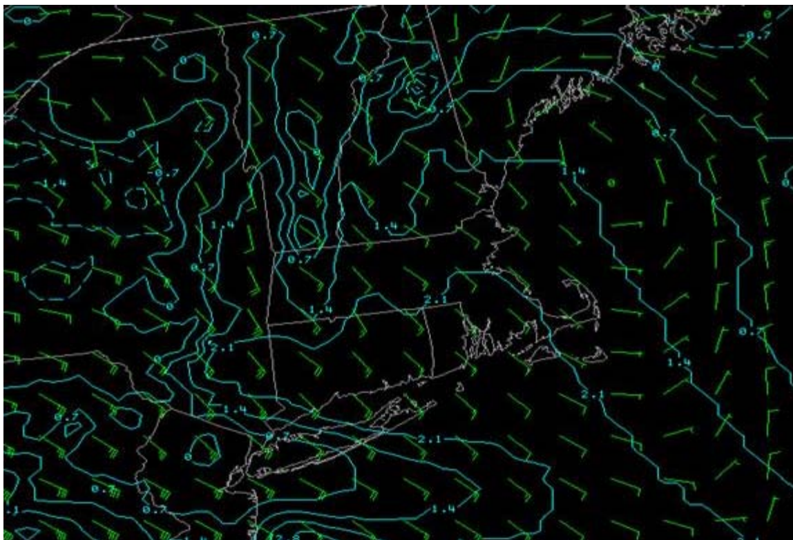
Figure 13. NAM forecast 925 mb
