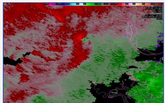
Storm relative velocity images of EF-1 tornadoes that occurred during an otherwise relatively uneventful 2016: the Fort Stewart GA tornado of Feb 3rd (top) and the Bloomingdale GA tornado of May 17th.
