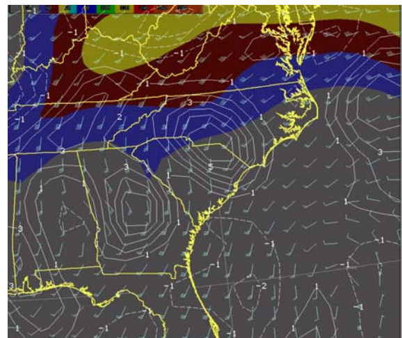
Fig 9. RUC 250 hPa 1500 UTC 27 September isotachs 2004 [shaded 30 kt (blue), 40 kt (red), 50 kt (yellow)], wind barbs and divergence (positive-solid white contour).
