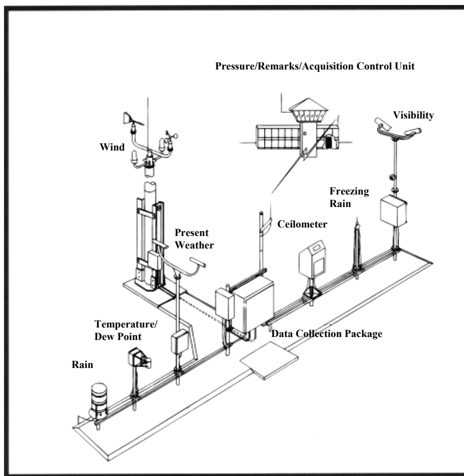
Figure 7. Standard Automated Surface Observing System (ASOS) (Adapted from: ASOS User's Guide 1998)
