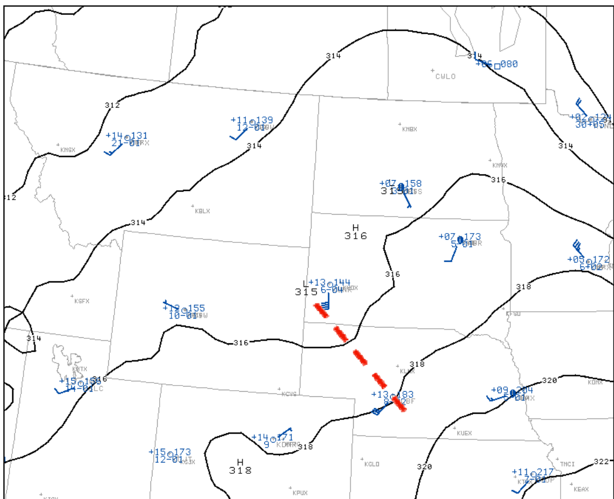
Figure 6. Same as Fig. 5, except analysis from 0000 UTC 18 August 2007.
