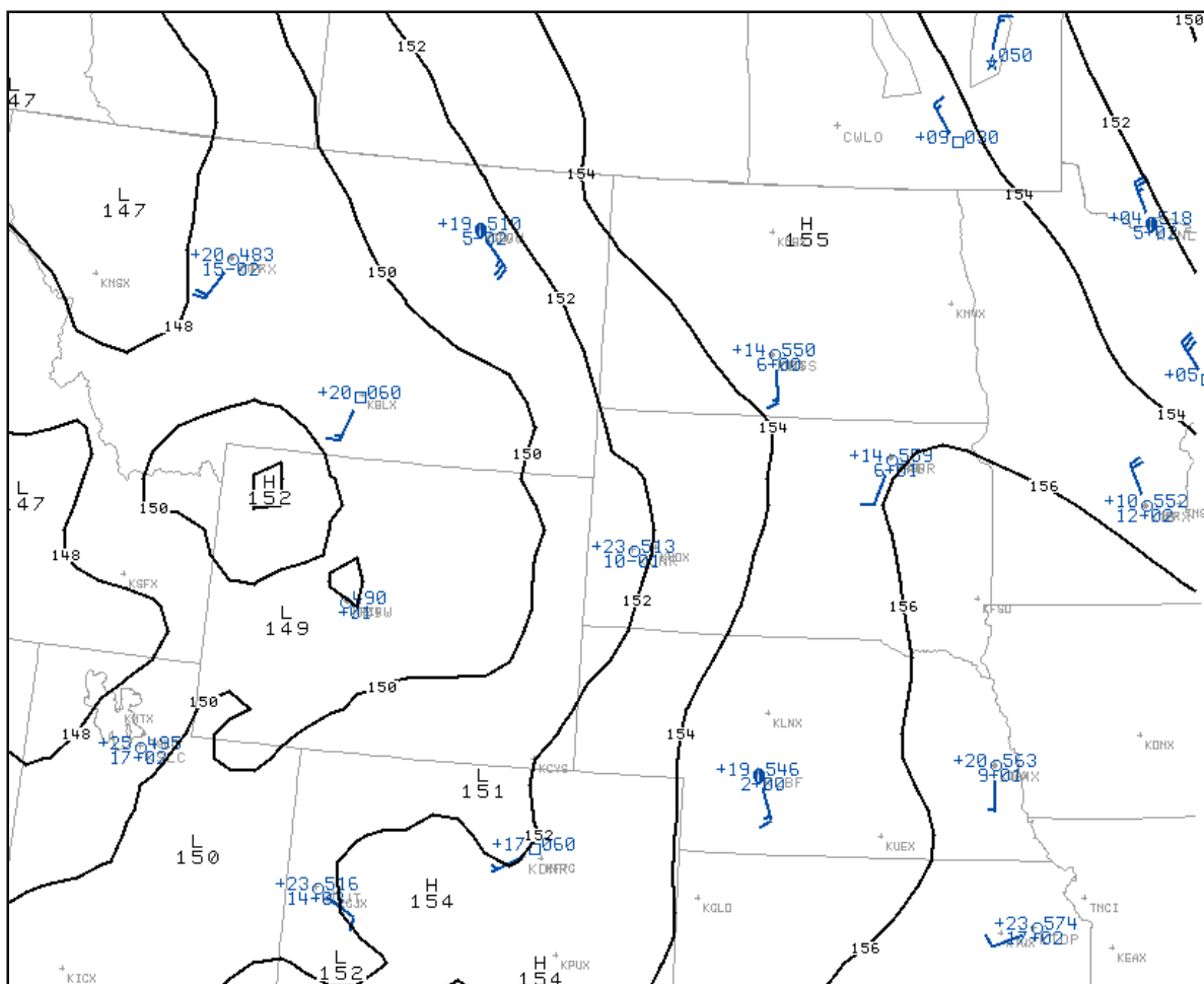
Figure 7. 850-mb analysis from 1200 UTC 17 August 2007. Height contours at 20-dam intervals with station plot in standard notation.
