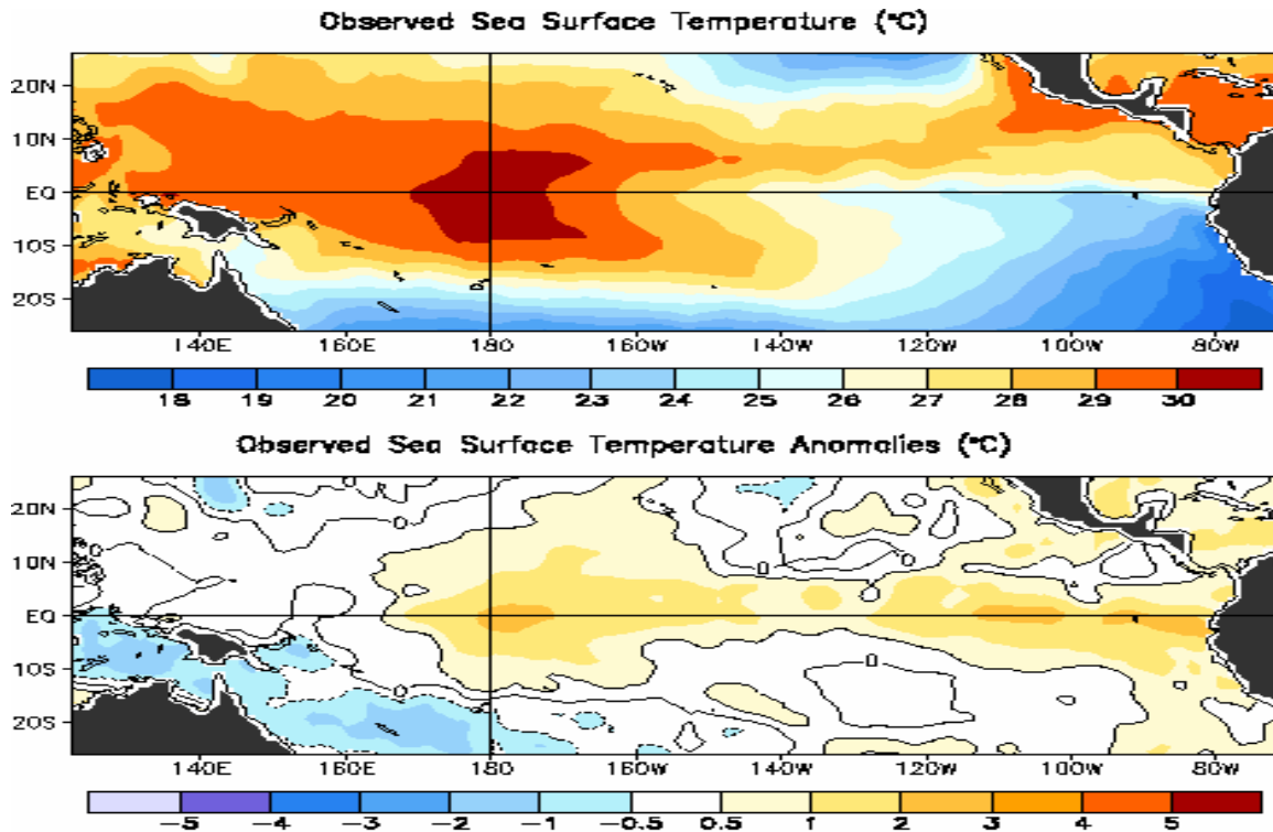
Figure 1. Observed Sea Surface Temperatures (top) and temperature departure from normal (bottom) across the Equatorial Pacific Ocean on 25 October 2006
