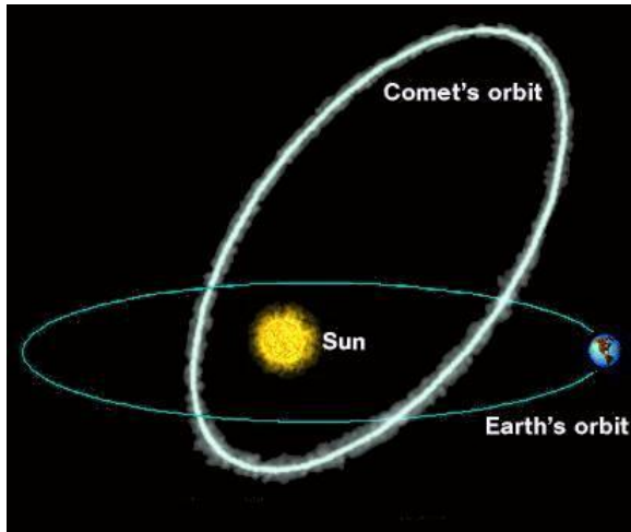
Figure 1 Earth's orbit intersecting the debris from a comet orbiting the sun, leading to a meteor shower
