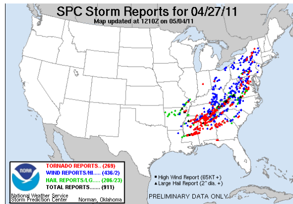
Figure 1 Preliminary SPC Storm Reports for April 27, 2011
