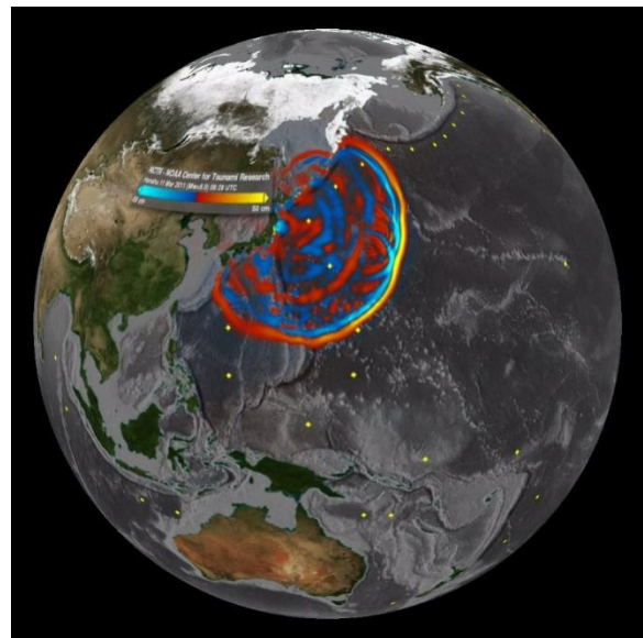
Figure 1 Wave propagation from the Japan Earthquake
