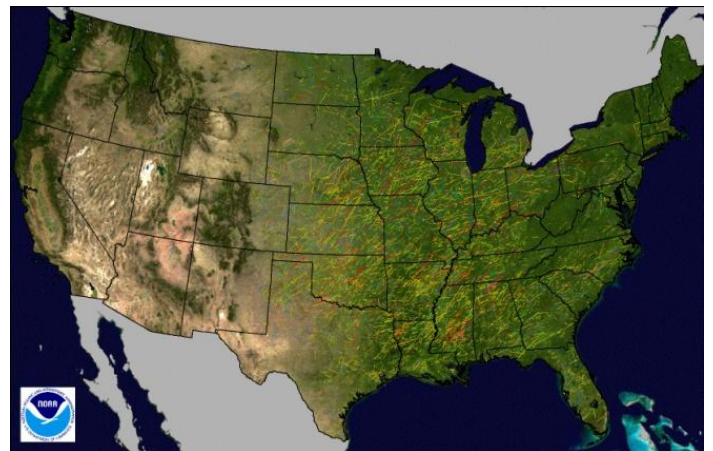
Figure 1 Tornado track and EF scale plots
