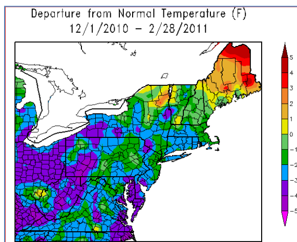
Figure 1 Temperature Departures Winter of 2010-11
