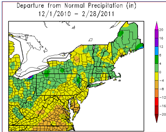
Figure 2 Precipitation Departures Winter 2010-11
