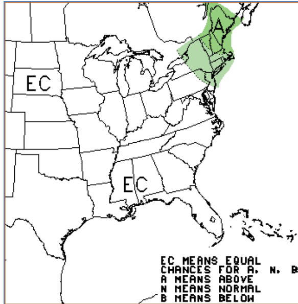
Figure 4. Summer Seasonal Precipitation
