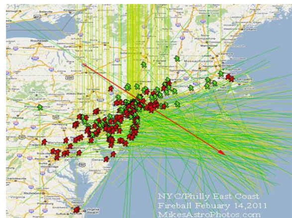
Figure 2 Plotted tracks of the meteor from observers in the Middle Atlantic Region and Southern new England
