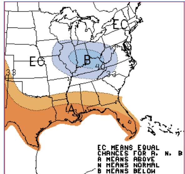
Figure 3. Summer Seasonal Temperature Outlook
