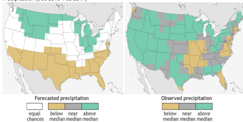
Figure 6. Precipitation Forecast/Verification
