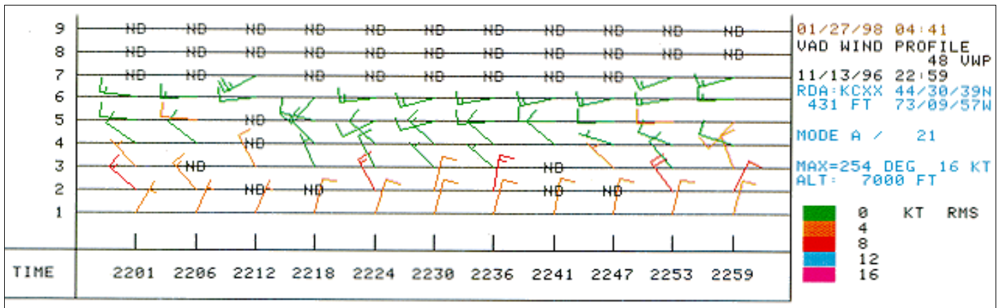
Figure 17. Same as Fig. 3, except it is for 13 November 1996 between 2201 and 2259 UTC. The north winds at 1,000-ft allowed for a long trajectory over Lake Champlain.
