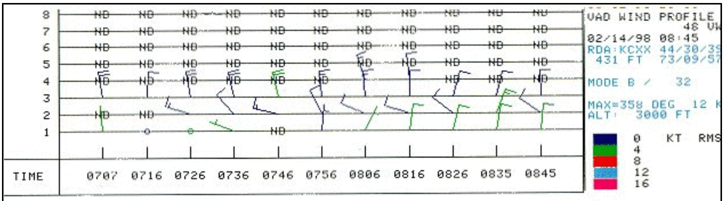
Figure 14. Same as Fig. 3, except it is for the period 0707 to 0845 UTC on 14 February 1998. It shows northerly winds in a 3,000-ft layer with an occasional westerly component at 2,000-ft.
