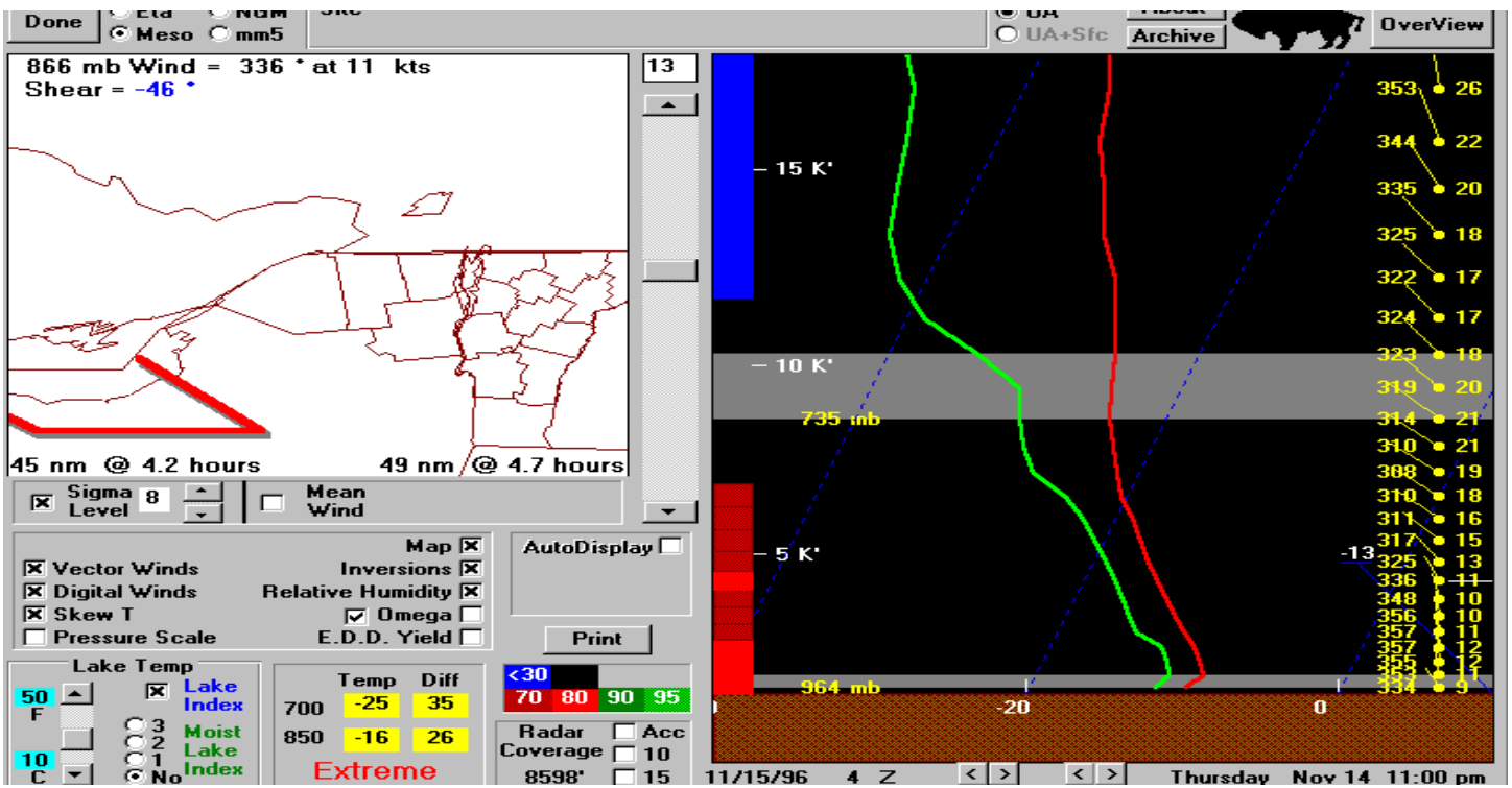
Figure 7. Meso-Eta forecast sounding for KBTV at 0400 UTC 15 November 1996 from the 1500 UTC 14 November run displayed with BUFKIT. The sounding shows extreme instability over Lake Champlain. Gray shaded areas on the sounding indicates an inversion layer. The left side of the display shows that a lake surface temperature of 10°C produced “extreme” instability.
