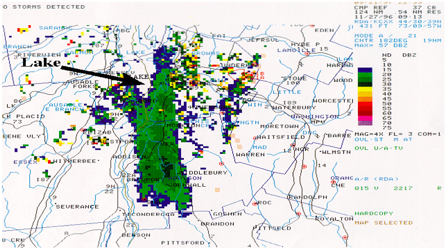
Figure 2. At 0913 UTC 27 November 1996 a large band of lake effect snow is depicted by a KCXX composite reflectivity image. Most notable is the area of 30 to 34 dBZ just north of Cornwall. The snow in this area may have been falling at a rate slightly over 2 inches per hour. The color table on the right depicts the intervals of maximum reflectivity in units of dBZ.
