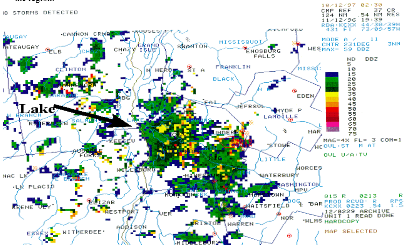
Figure 20. Composite reflectivity image at 1939 UTC from KCXX displays intense snow squalls (35-39 dBZ) that moved over Burlington on 12 November 1996. Numerous lighter snow showers are seen on the west side of Lake Champlain. The color table on the right depicts the intervals of maximum reflectivity in units of dBZ.
