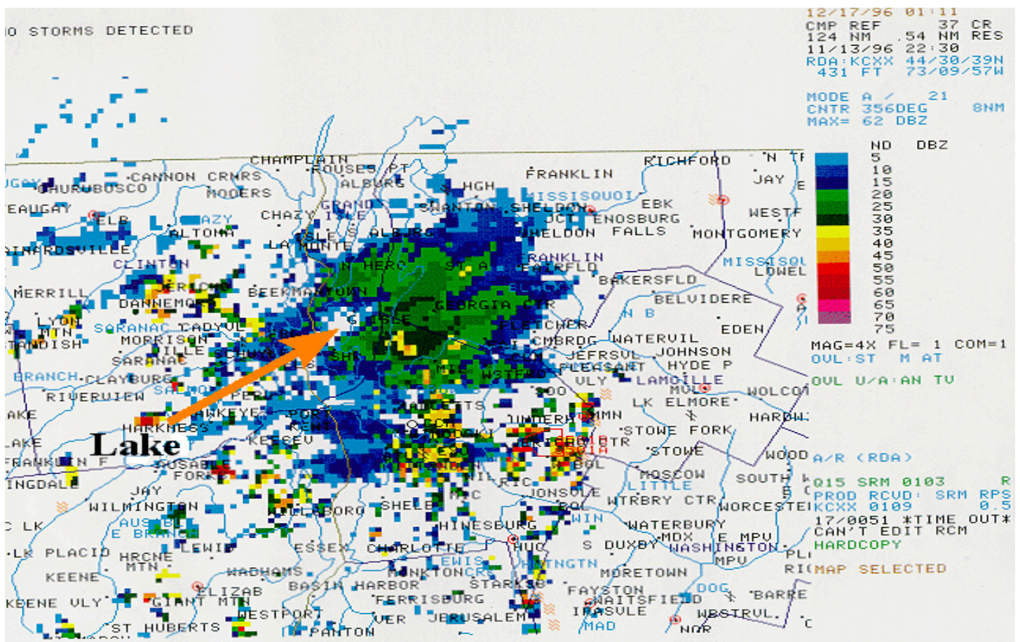
Figure 18. An intense lake enhanced snow squall depicted by the KCXX composite reflectivity image at 2230 UTC 13 November 1996. An impressive area of 30-40 dBZ is visible near the shore line of Lake Champlain. Lesser developed cells are seen north and south of this area over the open waters. A few light snow showers are seen on the windward side of the lake. The color table on the right depicts the intervals of maximum reflectivity in units of dBZ.
