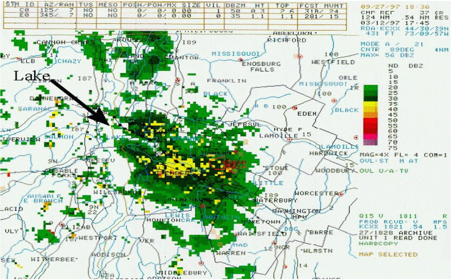
Figure 16. An example of lake enhanced snow squalls depicted by KCXX composite reflectivity at 1745 UTC on 12 March 1997. Burlington is located in the large area of 35-39 dBZ which was producing heavy snow. Other light snow showers are seen on the windward side of Lake Champlain. The WSR-88D SCIT algorithm identified this cell (black dots and line) and tracked it across the lake. The color table on the right depicts the intervals of maximum reflectivity in units of dBZ.
