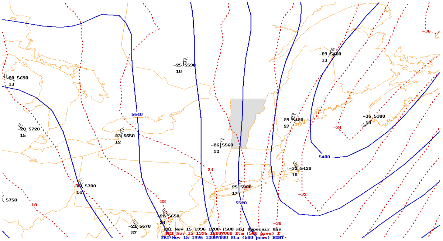
Figure 9. Eta model's 500-mb analysis at 1200 UTC 15 November 1996. Solid lines are geopotential heights (contoured every 60-m) and dash lines are isotherms (contoured every 2 °C). Upper air observations are shown.
