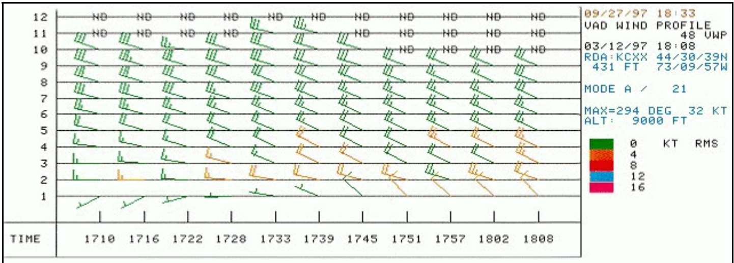
Figure 15. Same as Fig. 3, expect it is for 12 March 1997 between 1710 to 1808 UTC. It shows the passage of a surface trough around 1730 UTC.
