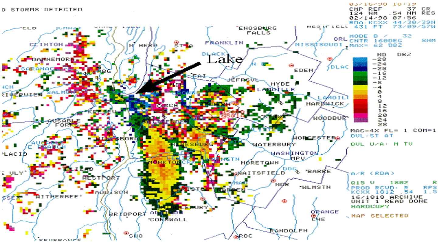
Figure 13. KCXX composite reflectivity image at 0756 UTC 14 February 1998. A weak band of snow is detected by radar on 14 February 1998. Reflectivity returns indicate that the band originates from the open waters just southeast of Plattsburgh (PBG) and then curves south with the northerly flow. The color table on the right depicts the intervals of maximum reflectivity in units of dBZ.
