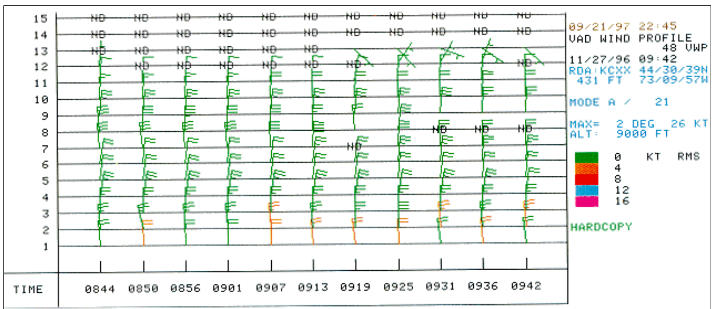
Figure 3. KCXX VWP from 0844 to 0942 UTC on 27 November 1996 depicting a deep layer of north winds at Burlington. Full wind bars are 5 \text{ ms}^{-1} and half bars are 2.5 \text{ ms}^{-1} . Vertical axis is altitude in thousand feet. "ND" indicates no data. Color table at the right depicts the root-mean-square error (knots) for each wind estimate.
