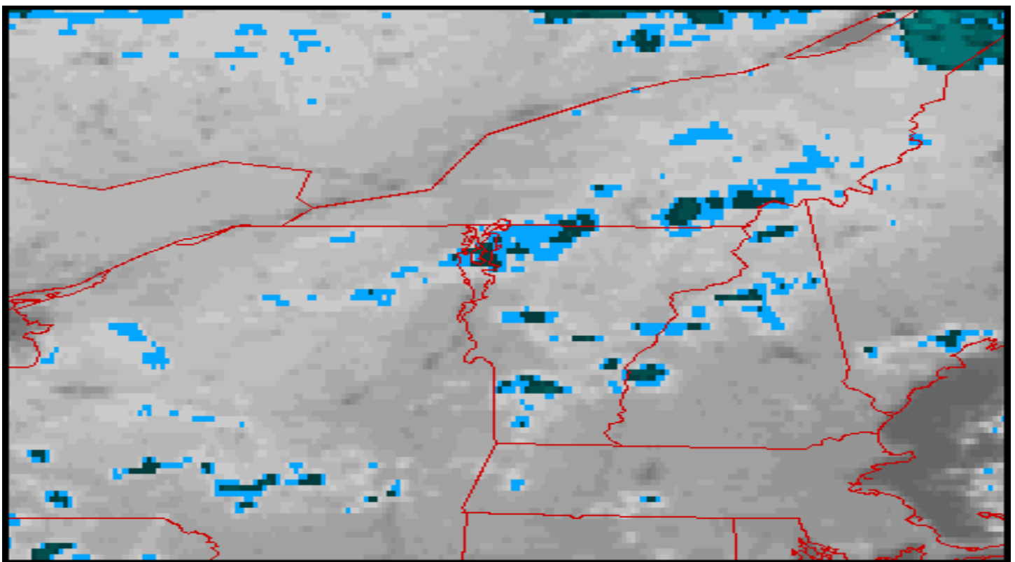
Figure 19. GOES-8 10.7 \mu\text{m} satellite image depicting enhanced clouds (dark blue is -21^{\circ}\text{C} ) over Lake Champlain at 2245 UTC on 13 November 1996. Other enhanced cold cloud tops indicate snow showers in the region.
