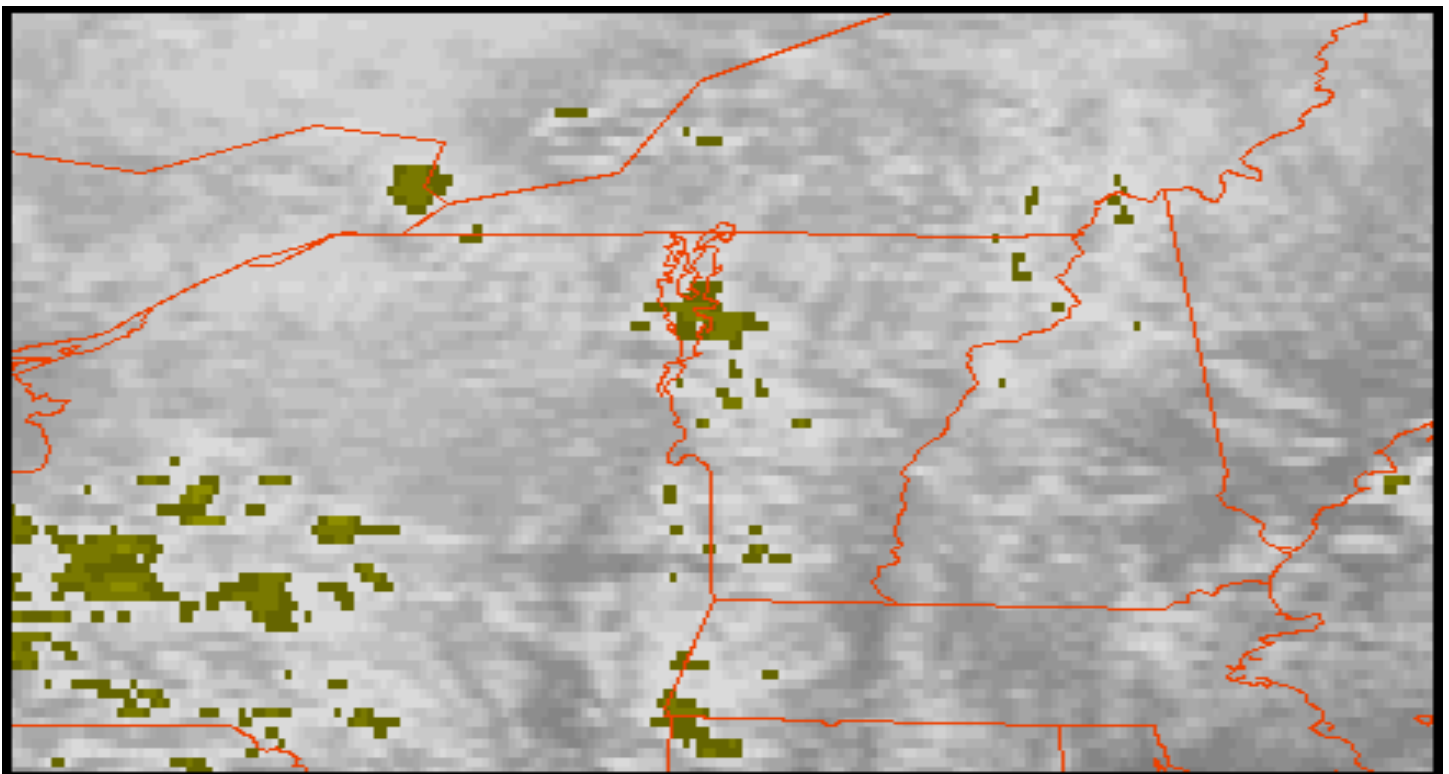
Figure 22. GOES-8 10.7 \mu\text{m} satellite image taken at 1745 UTC on 12 November 1996 depicting one of the heavy snow squalls that affected Burlington. Cloud top temperatures over Lake Champlain were between -20 and -25 ^{\circ}\text{C} indicated by the greenish-yellow enhancement.
