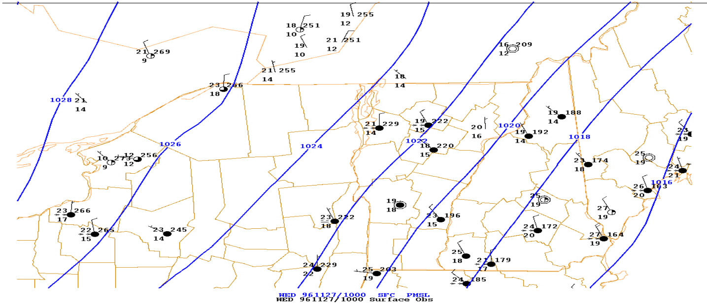
Figure 5. Surface analysis on 27 November 1996 at 1000 UTC. Solid lines are isobars contoured every 2-mb. Surface observations are shown on the map. Temperature and dew point temperature (°F) are on the left side of each observation. Present weather, if applicable, is located between the two temperatures. Full wind barbs at 5 ms -1 and half wind barbs are 2.5 ms -1 . Mean sea level pressure is located on the upper right of the observations in units of tenths of a millibar. Sky condition, if available, is indicated by the shading of the circle.
