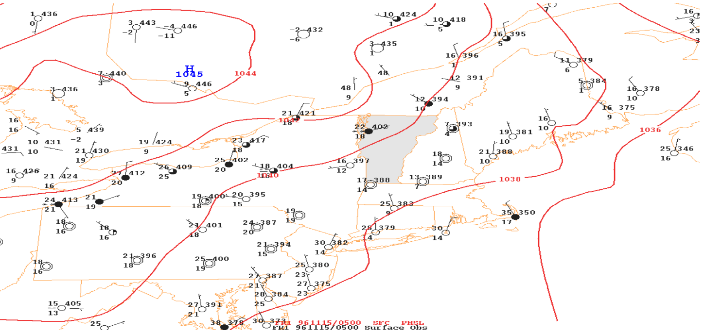
Figure 8. Same as Fig. 5, except it is from 0500 UTC on 15 November 1996.
