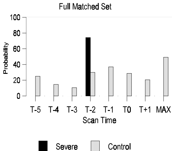
Figure 4. Probability of Hail from five volume scans prior to time of severe event or peak of storm to one volume scan after.
