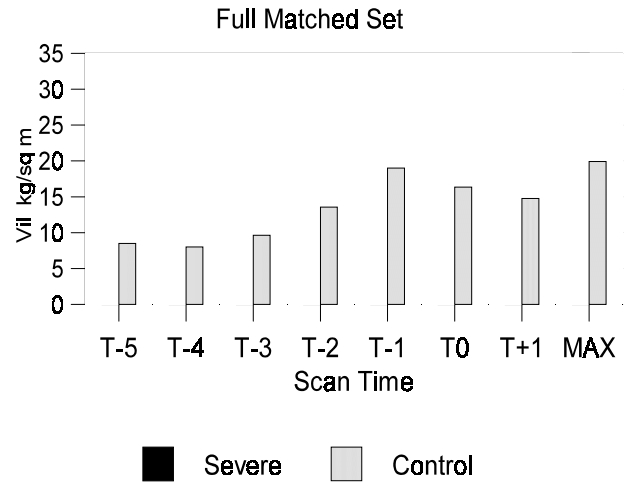
Figure 3. Cell VIL - Control and severe events matched by date for T-5 volume scans to T+1, and maximum value.
