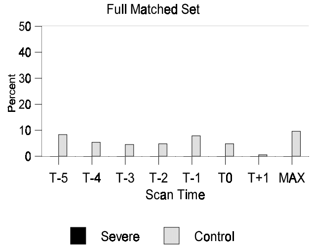
Figure 5. Probability of Severe Hail (POSH) from five volume scans prior to time of severe event or peak of storm to one volume scan after.
