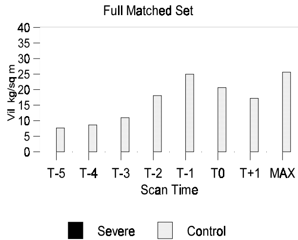
Figure 2. Grid VIL. Severe and control cases matched by date for T-5 volume scans to T+1 volume scans and max value.
