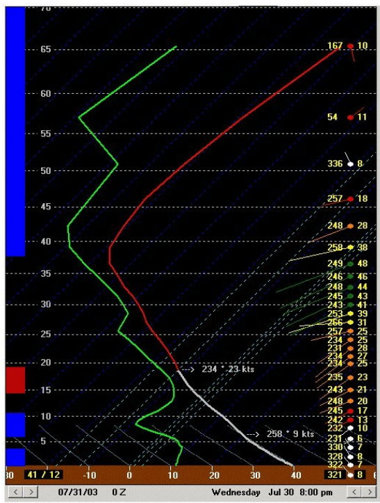
Figure 4 Sounding information for a) observed Medford, Oregon (MFR) sounding valid at 0000 UTC 31 July 2003 and b) BUFKIT display of Medford, Oregon (MFR) 12 hour Eta model forecast sounding valid at 0000 UTC 31 July 2003.
