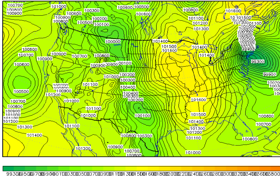
PRMSL at 18Z Tue 19apr1983
