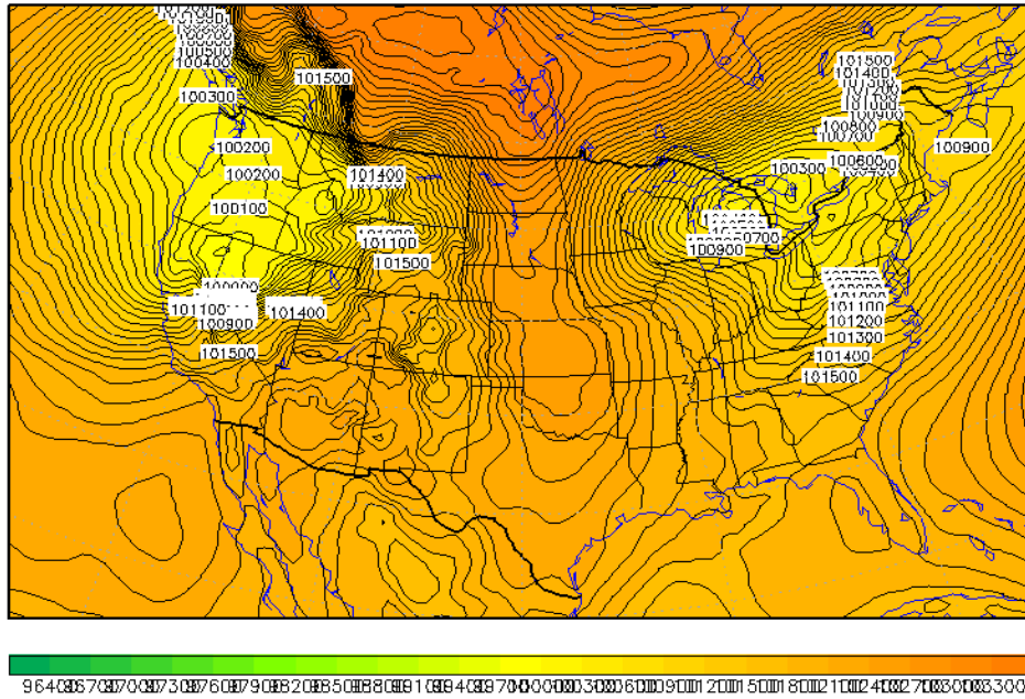
PRMSL at 21Z Fri 16feb1990
