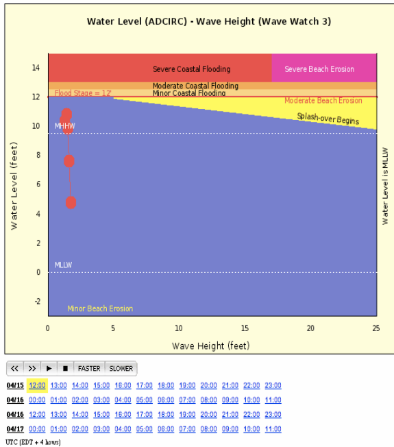
Figure 2. An example of a coastal flood nomogram recreated for the 16 April, 2007 (Patriot’s Day) nor’easter. The nomogram animates predicted hourly water levels for Portland Harbor versus forecast wave heights at near-shore buoys. The red line represents the benchmark for coastal flooding, while the yellow shading depicts the onset of splash-over. Click on the image to view animation.
