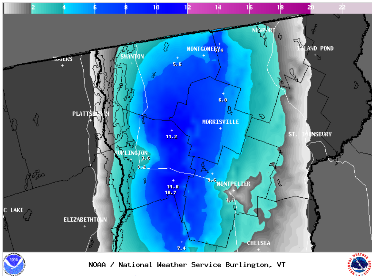
Figure 32. As in Fig. 31, except for cases with a Froude Number between 0.5 and 1.
