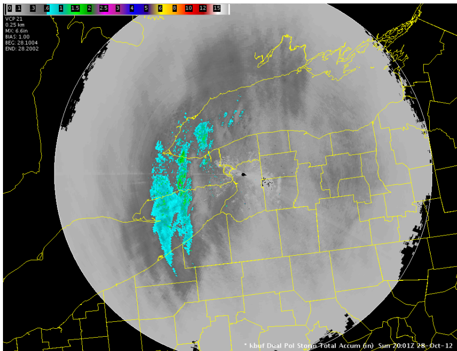
Figure 5. DP Storm Total Precipitation QPE from the Buffalo radar on October 28 th , 2012 between 1004Z and 2002Z. This is the same event but using a multiplier of 1.5 for snow and ice crystals. Note the reduction of the melting layer discontinuity ring.
