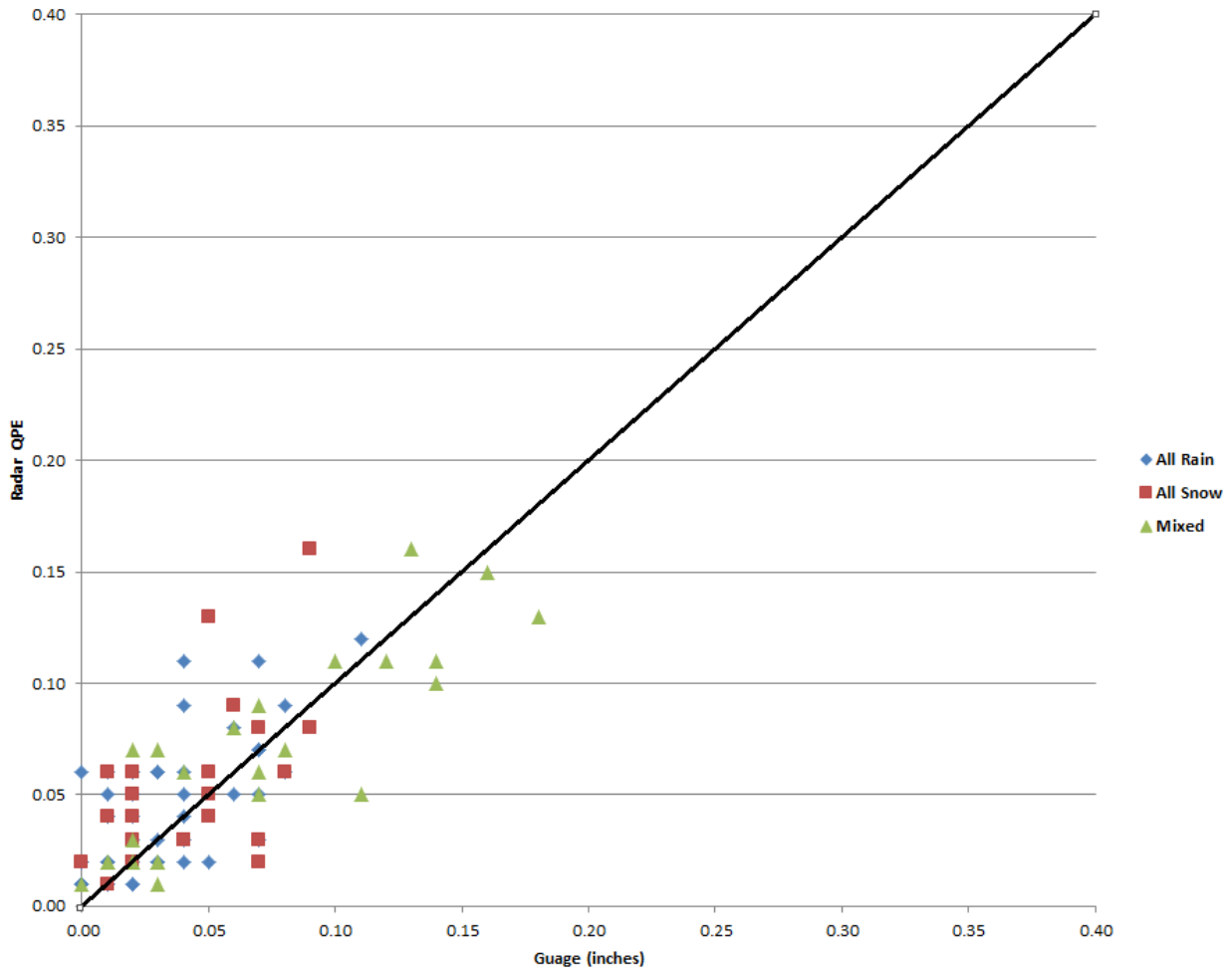
Figure 3. A scatterplot graph which compares DP QPE to gauge measured precipitation for 102 hourly cases with a 1.4 coefficient categorized by precipitation type at ground level.
