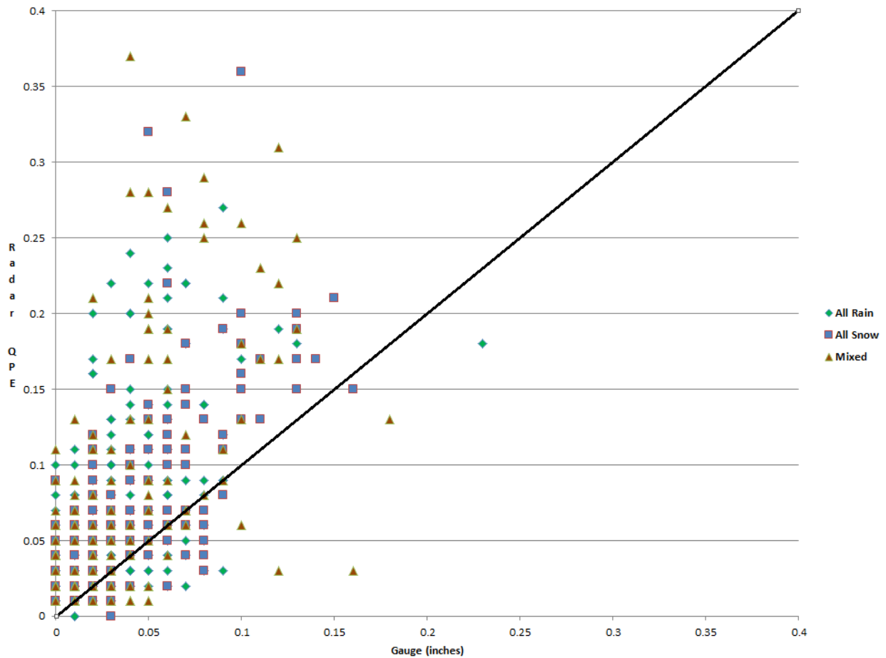
Figure 2. A scatterplot graph which compares DP QPE to gauge measured precipitation for 620 hourly cases with a 2.8 coefficient categorized by precipitation type at ground level.
