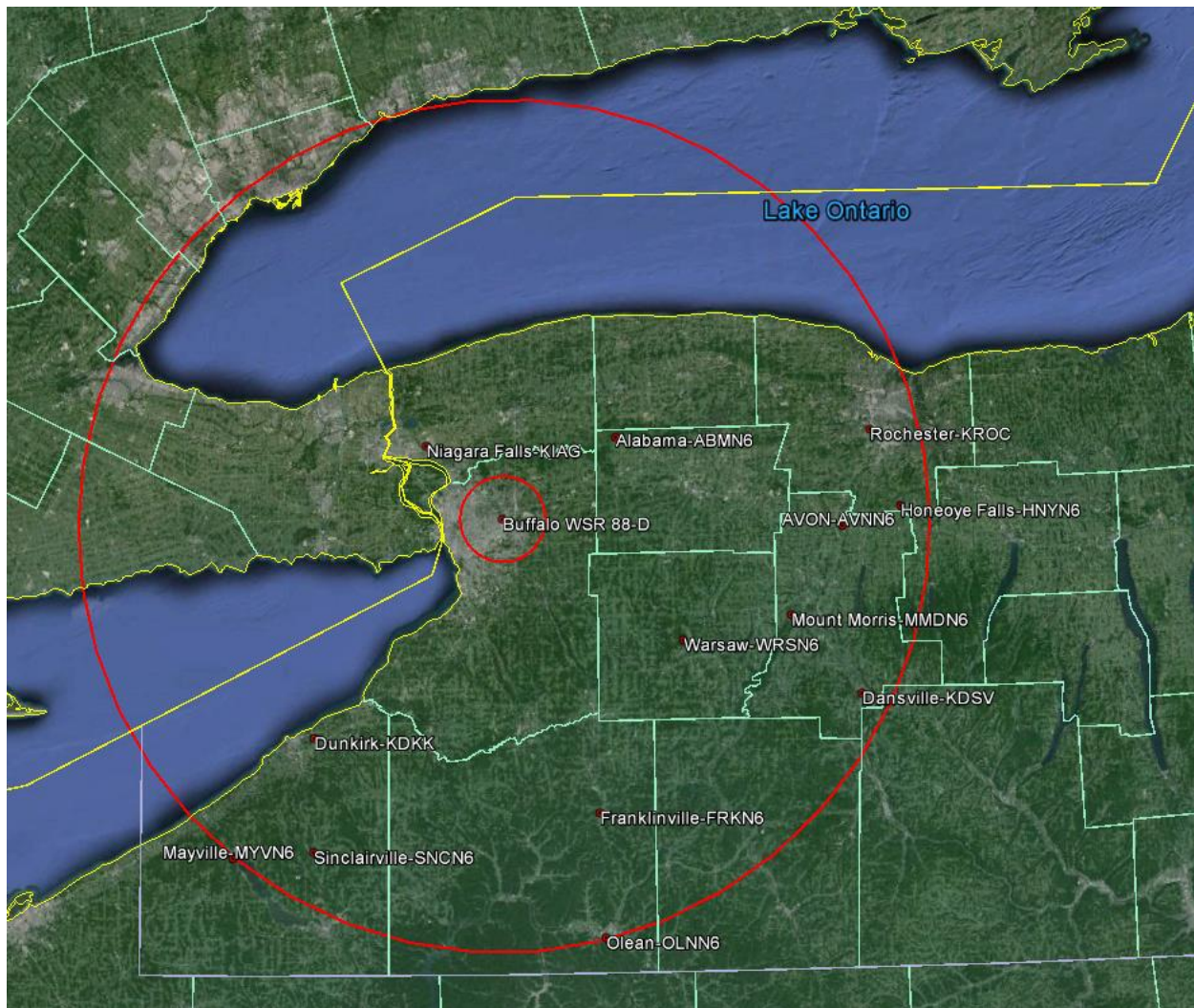
Figure 1. A map showing the location of the 13 precipitation gauges used for this study and range rings at a distance of 10 km and 100 km from the Buffalo WSR-88D.
