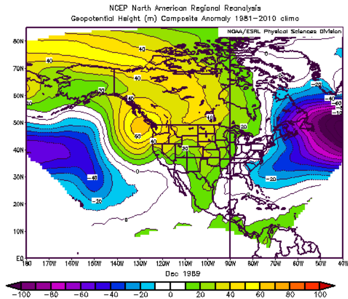
Figure 14a. 500 hPa geopotential height composite anomaly (m), from the 1981-2010 climatology, during December 1989. Figure from NOAA's Earth System Research Laboratory.
