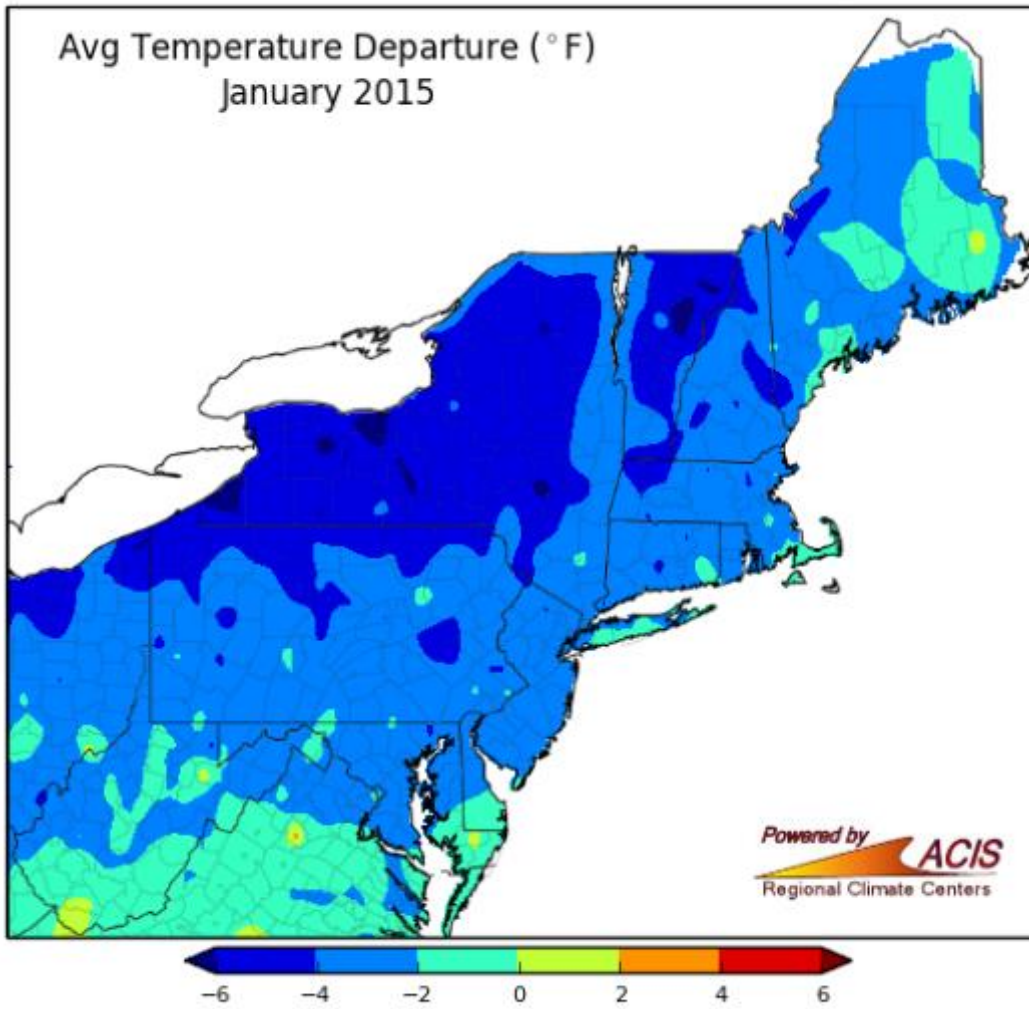
Figure 2. January 2015 departure from normal temperature (°F). Figure from the Northeast Regional Climate Center .
