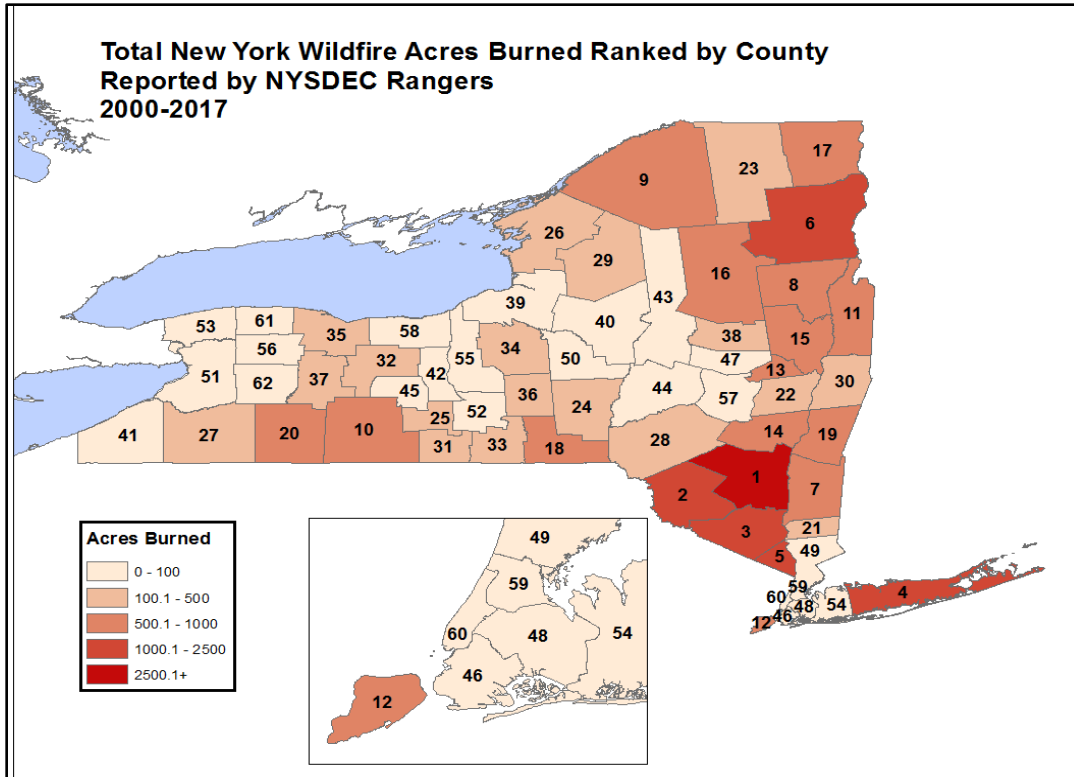
Figure 9. Total wildfire-acres burned ranked by county and color-filled from 2000-2017.
