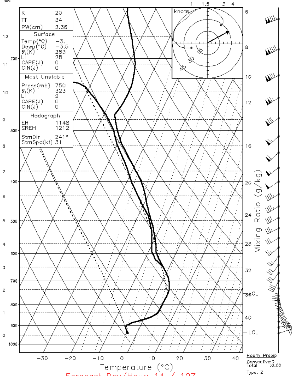
Figure 11. Vertical profile or sounding taken at UNV valid at 1000 UTC 14 November 1997. Data are from the 1500 UTC 29 km Eta profile data base.
