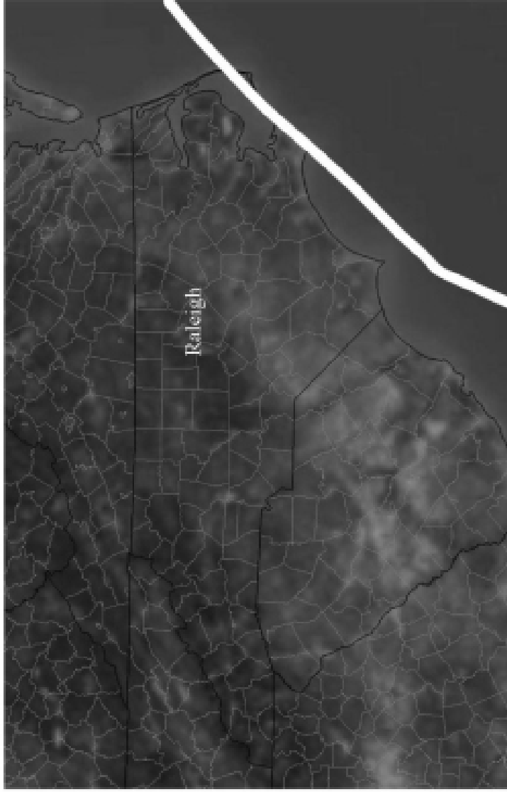
Figure 11. As in Fig. 5, except for Arthur (June 1996).
