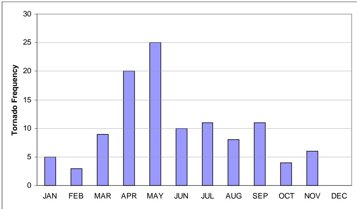
Figure 5. Monthly distribution of all tornado segments reported within the Charleston CWA from 1950 to 1993. Total tornado segments is 112.
