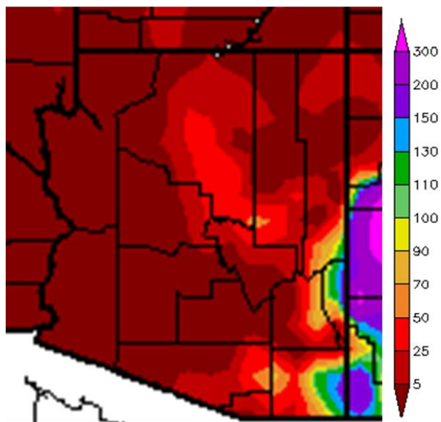
Percent of Normal Precipitation June 2017
