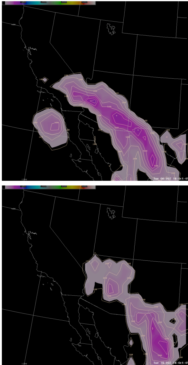
Figure 5. CAPE at (a) 0600 UTC and (b) 1800 UTC. Contours every 100 \text{ J kg}^{-1} .
