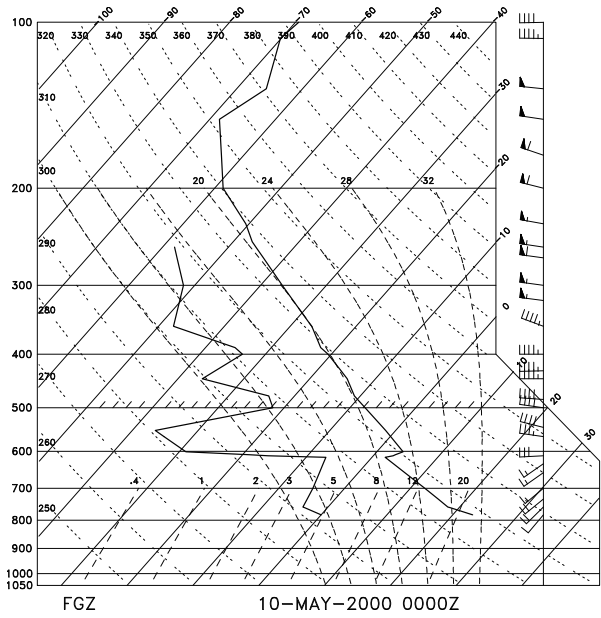
Figure 4: As in Figure 2, except for 0000 UTC 10 May 2000.
