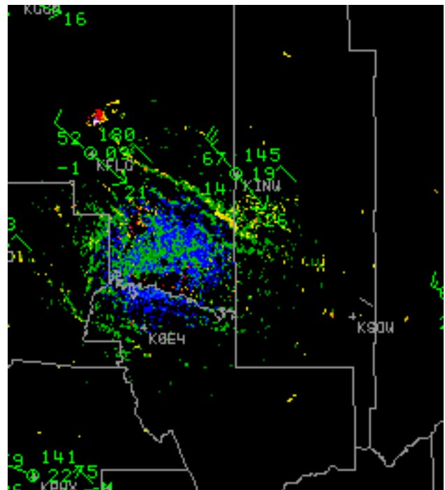
Figure 3: WSR-88D image taken at 2117 UTC 17 March 2000. The convergence zone can be clearly seen lying between Flagstaff (KFLG) and Winslow (KINW). Station plot uses standard notation.
