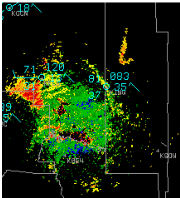
Figure 5: As in Fig. 3, except for 2106 UTC 09 May 2000.
