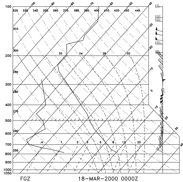
Figure 2: Skew T\text{-ln } p plot from Flagstaff, Arizona (FGZ) taken at 0000 UTC 18 March 2000.
