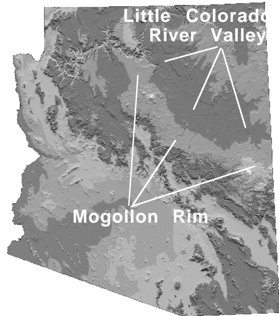
Figure 1: Image showing terrain and elevation over the state of Arizona. The Mogollon Rim and Little Colorado River Valley are noted.
