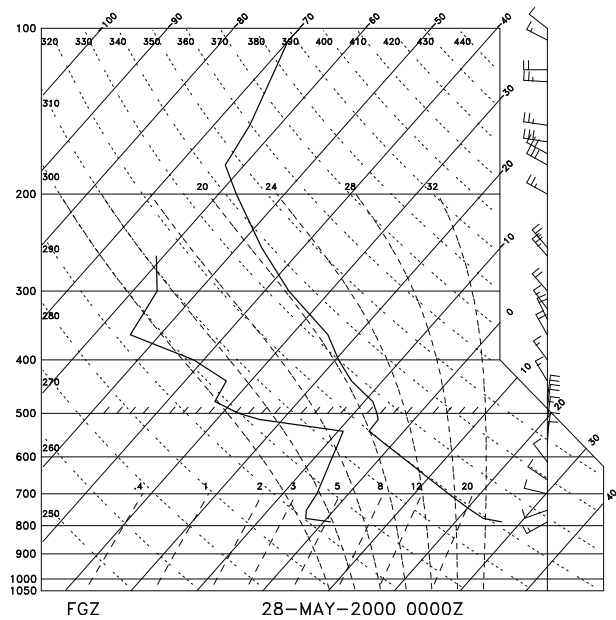
Figure 6: As in Fig. 2, except for 0000 UTC 28 May 2000.
