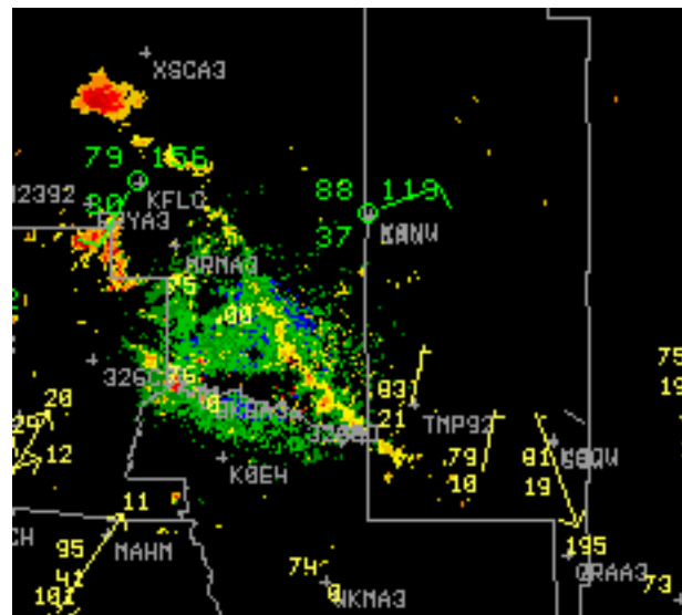
Figure 7: As in Fig. 3, except for 0126 UTC 28 May 2000.
