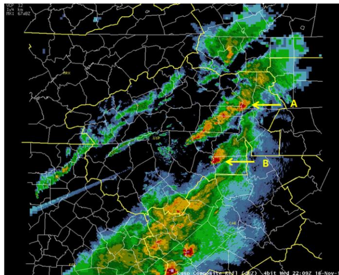
Fig. 13. KGSP WSR-88D 2119 UTC (top) and 2209 UTC (bottom) on 16 November 2011 composite reflectivity images showing the storm associated with the Cleveland County tornado (A) and the storm associated with the tornadoes in Union, Chester, and York counties (B).
