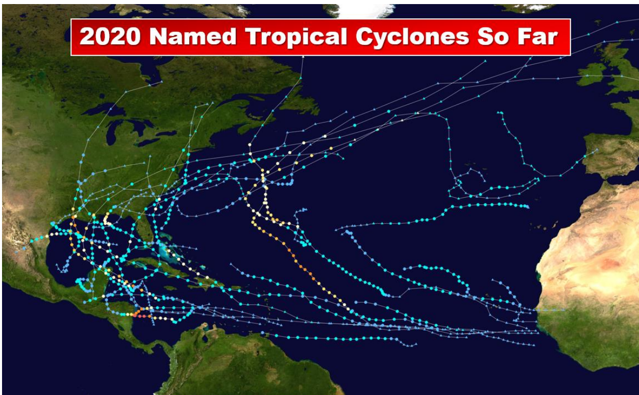
Figure 1: 2020 tracks of named Atlantic tropical cyclones so far. Image adapted from https://upload.wikimedia.org/wikipedia/commons/3/3c/2020_Atlantic_hurricane_season_summary_map.png .
