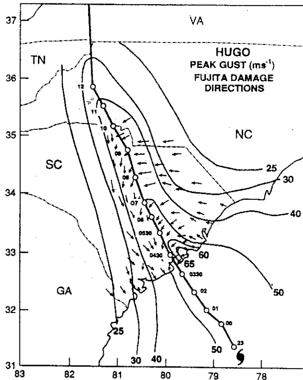
FIG. 13. Envelope of peak gusts relative to the track of Hugo's wind center. Superimposed are (first) damage vector directions as determined by aerial surveys supplied by Ted Fujita of the University of Chicago.
