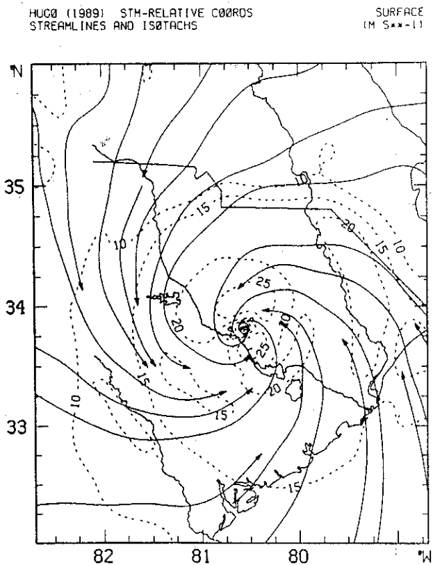
FIG. 10. As in Fig. 8, but for 0700 UTC on 22 September 1989. Data collection input is 0500–0900 UTC.
