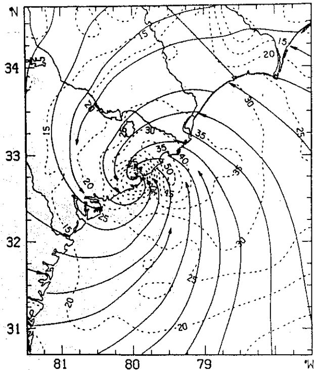
FIG. 8. As in Fig. 4, but for surface winds measured by oceanic, land-based, and adjusted aircraft platforms for 0400 UTC for 22 September 1989.
