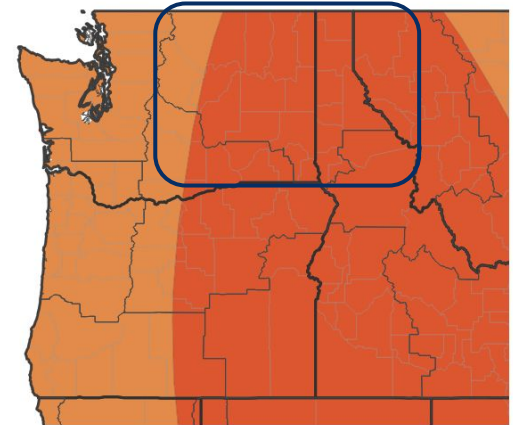
Seasonal (3-Month) Temperature Outlook
