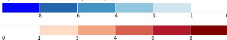
Departure from Normal Max Temperature (°F)
