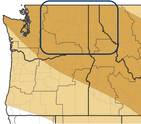
Seasonal (3-Month) Precipitation Outlook
