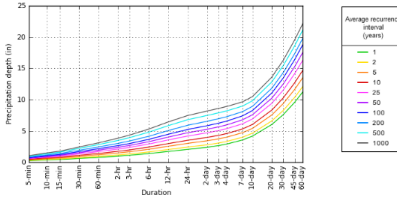
PDS-based depth-duration-frequency (DDF) curves Latitude: 42.9278°, Longitude: -75.1563°
