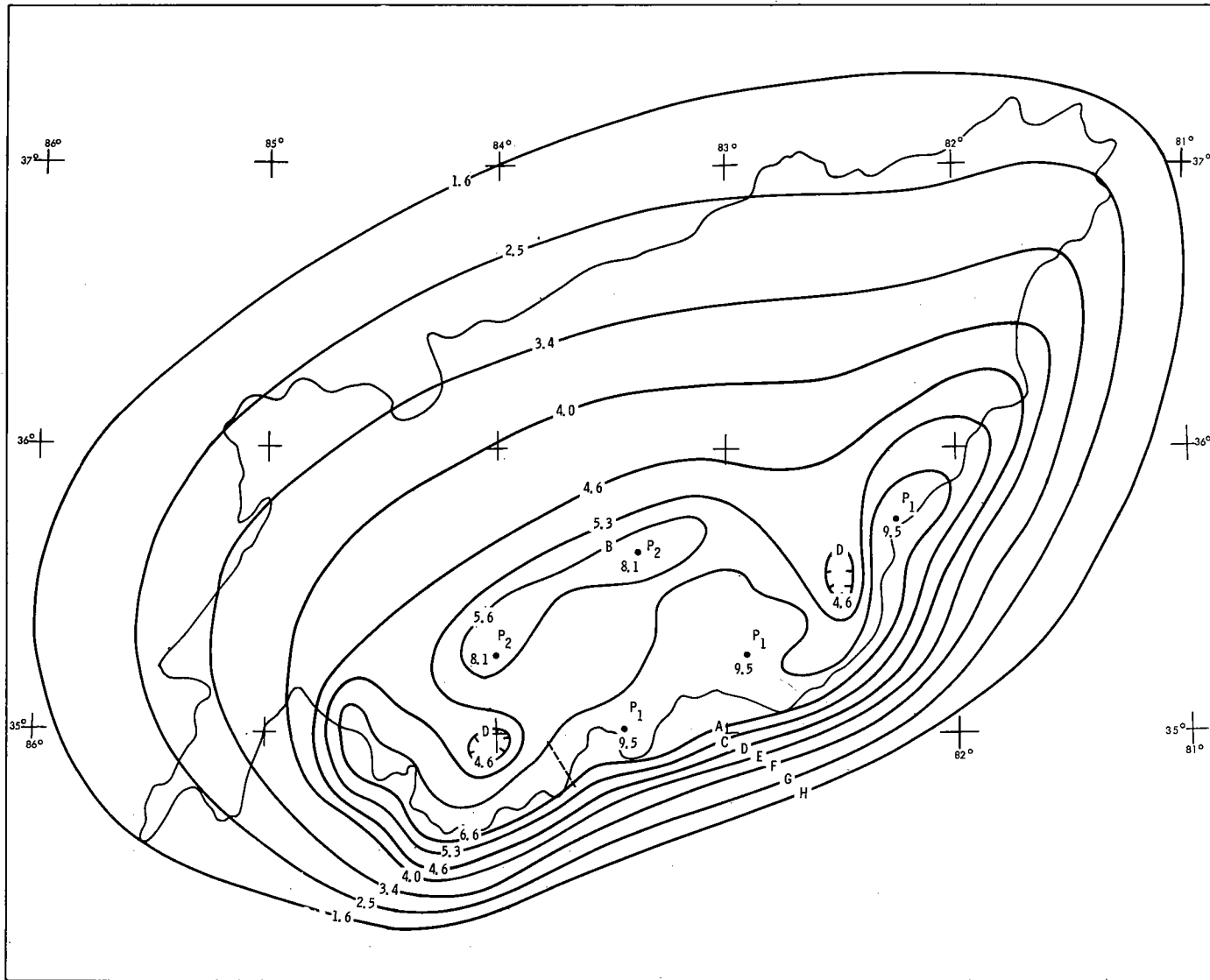
Figure 7-6. Probable maximum March isohyets (21,400-sq. mi. upstream), 1st 6 hours
