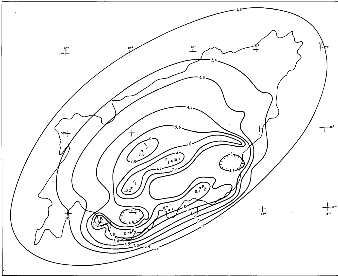
Figure 7-4. Probable maximum March isohyets (21,400-sq. mi. downstream), 1st 6 hours
