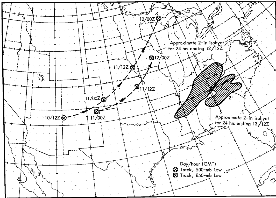
Figure 3-15. Low tracks and rain pattern - March 11-12, 1963
