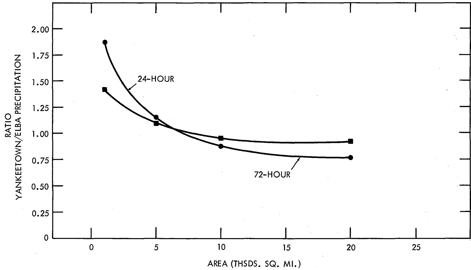
Figure 5-10. Seasonal variation of precipitation related to area
