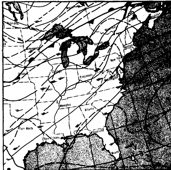
(700 mb) January 20, 1954
