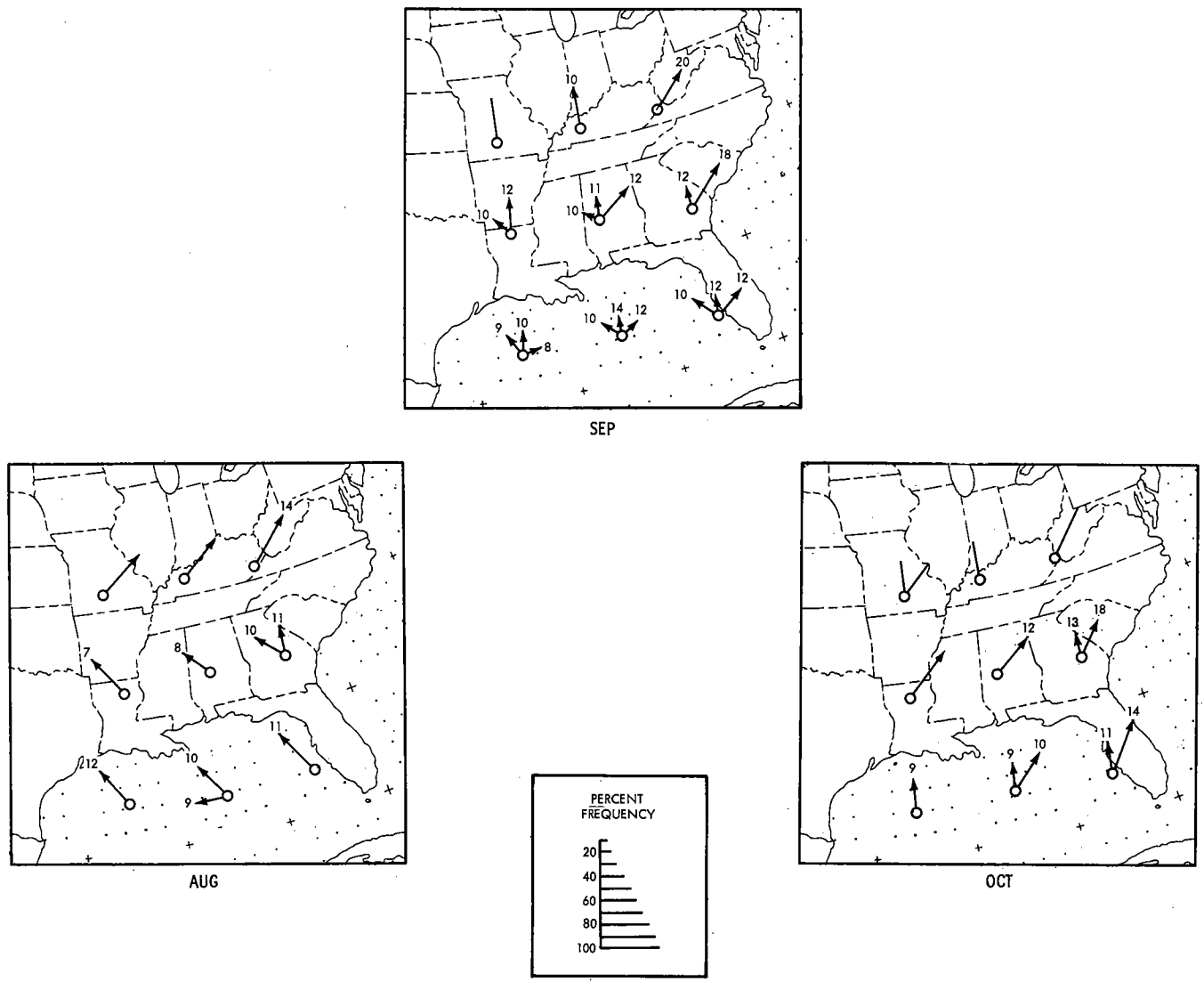
Figure 3-19a. Most frequent directions and median speed (kt.) of tropical storm movements (after Ref. 3-17)
