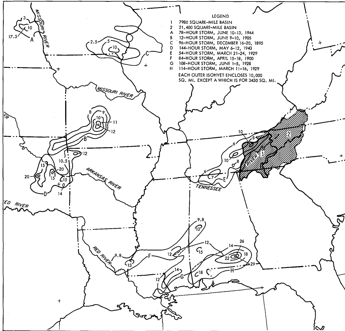
Figure 5-1. Isohyetal patterns of important storms
