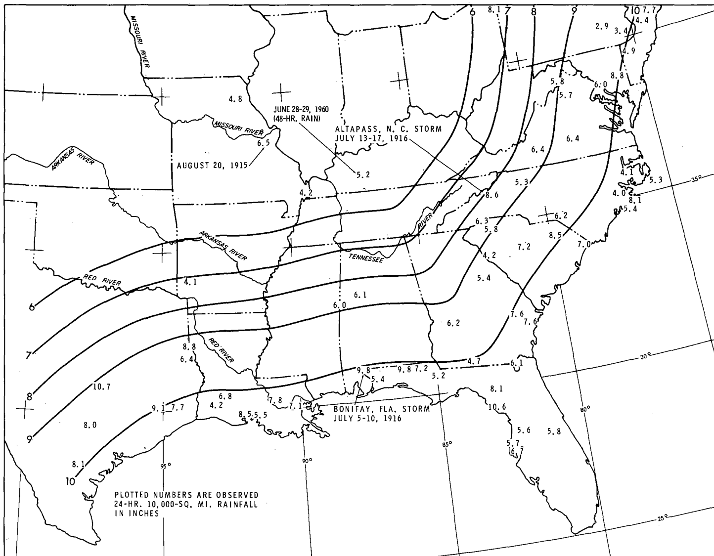
Figure 5-4. Distance-from-coast variation of summer TVA precipitation (non-orographic)
