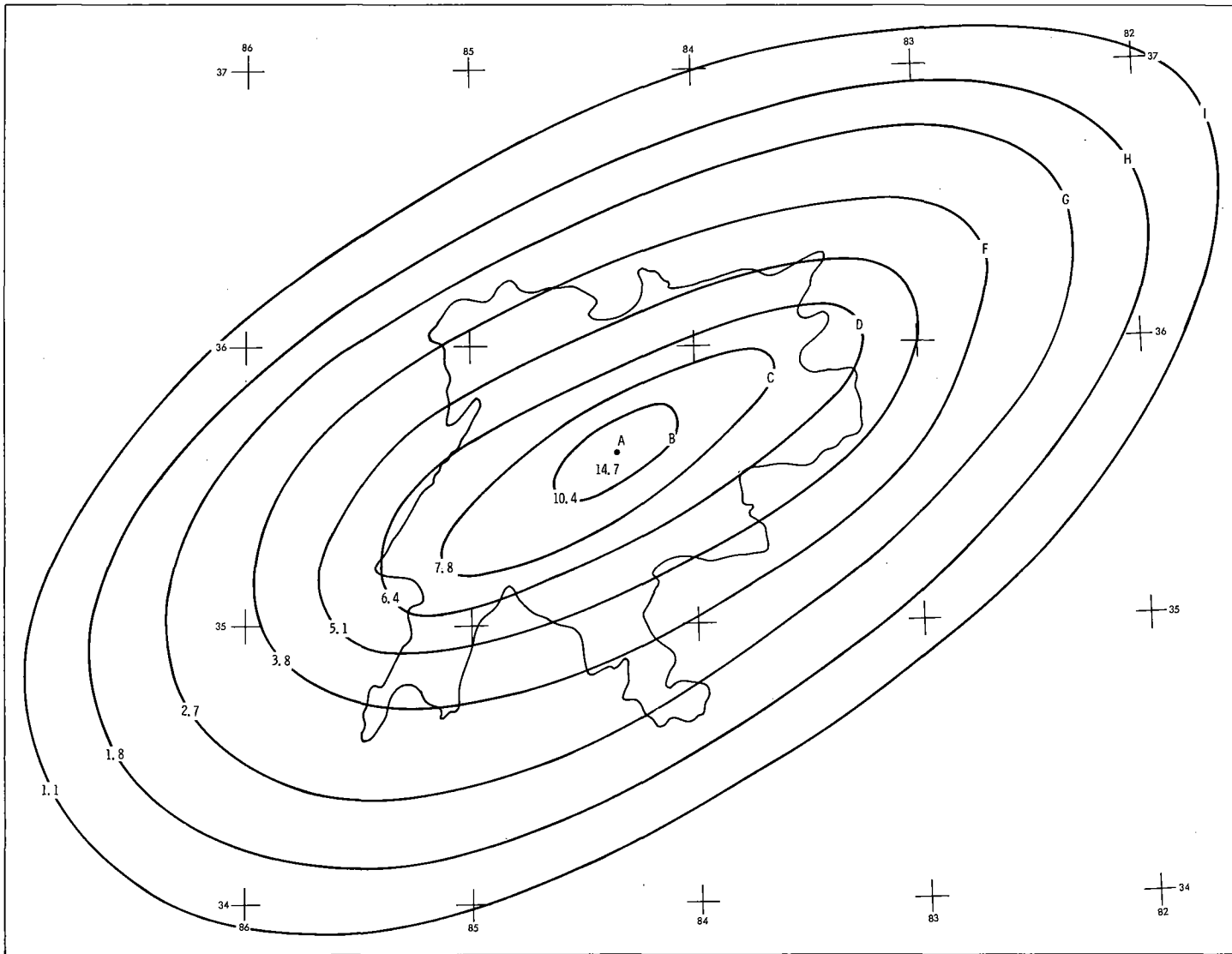
Figure 7-2. Probable maximum March isohyets (7980 sq. mi.), 1st 6 hours
