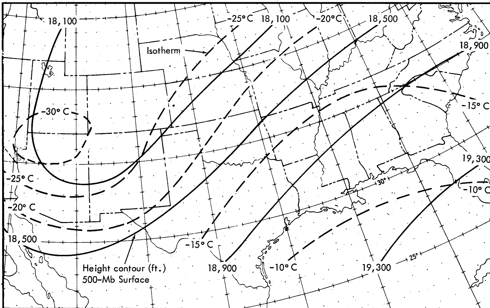
Figure 3-12. Mean 500-mb flow for March 4-5, 1963
