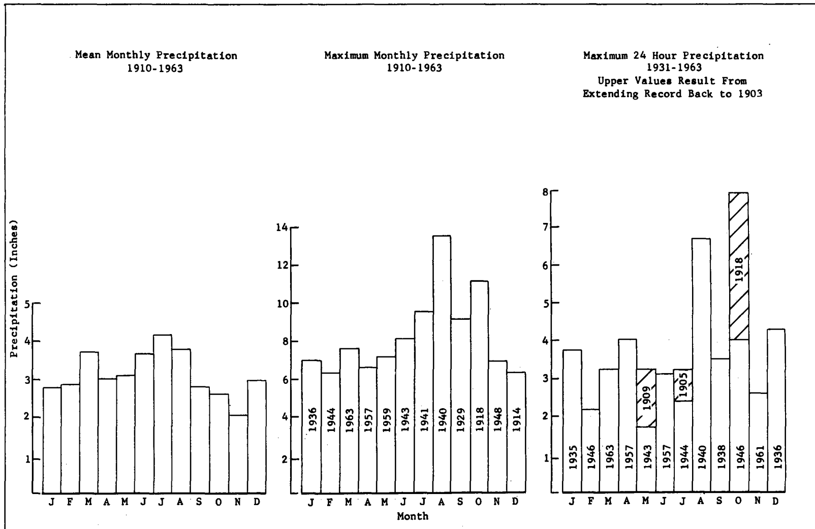
Figure 3-3. Mean and extreme rainfall - Asheville
