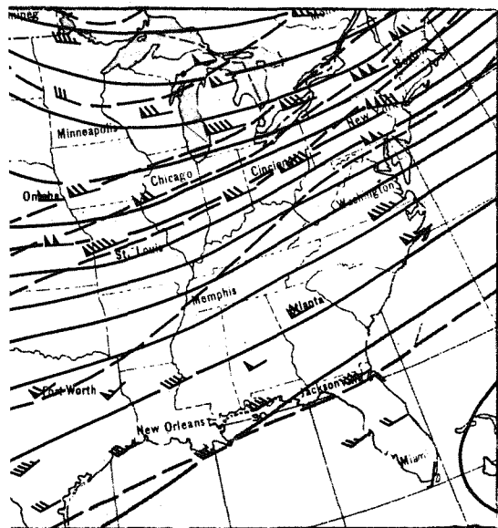
(500 mb) January 29, 1957
