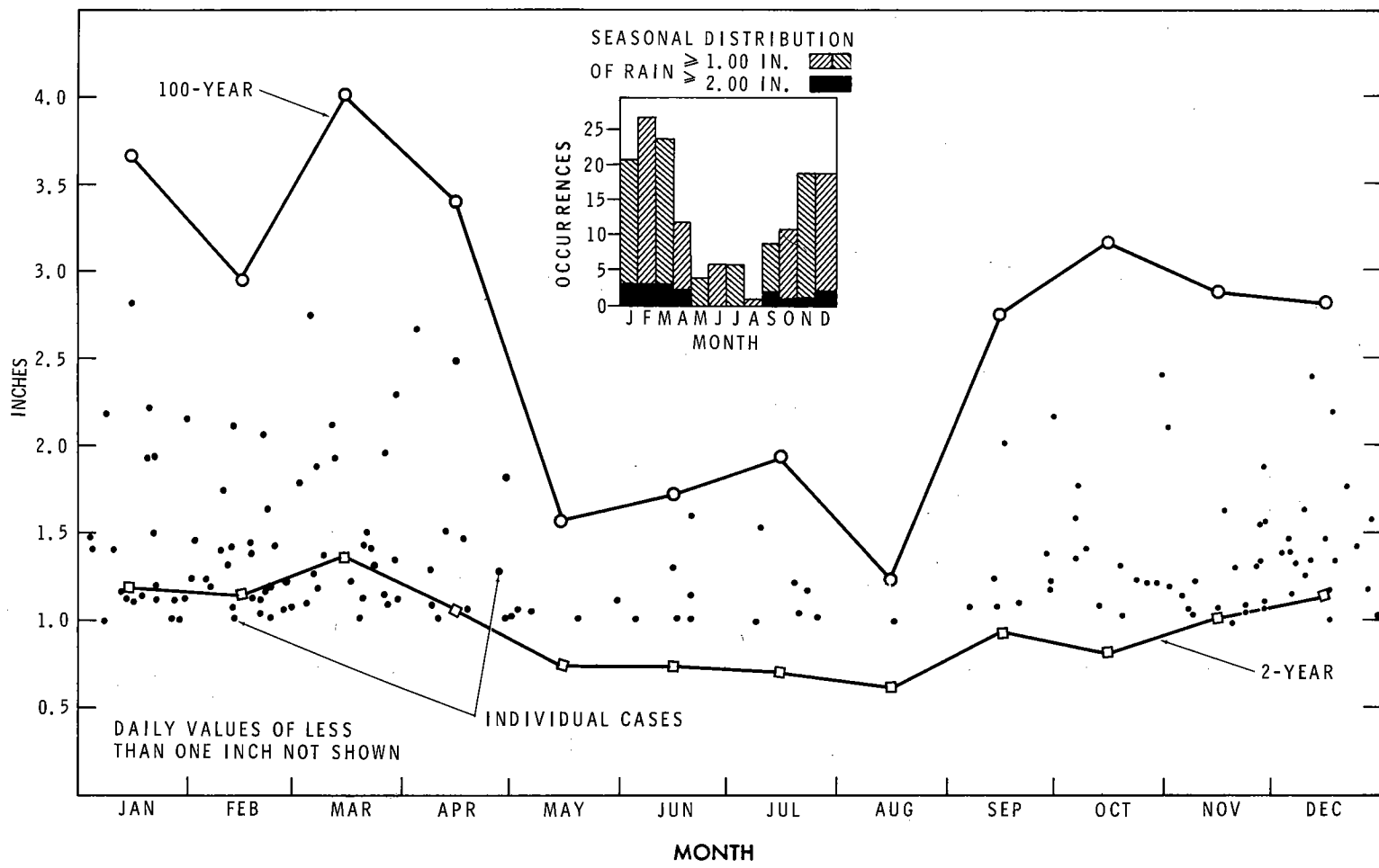
Figure 5-7. Daily rains of one inch or more above Chattanooga (1944-1963)
