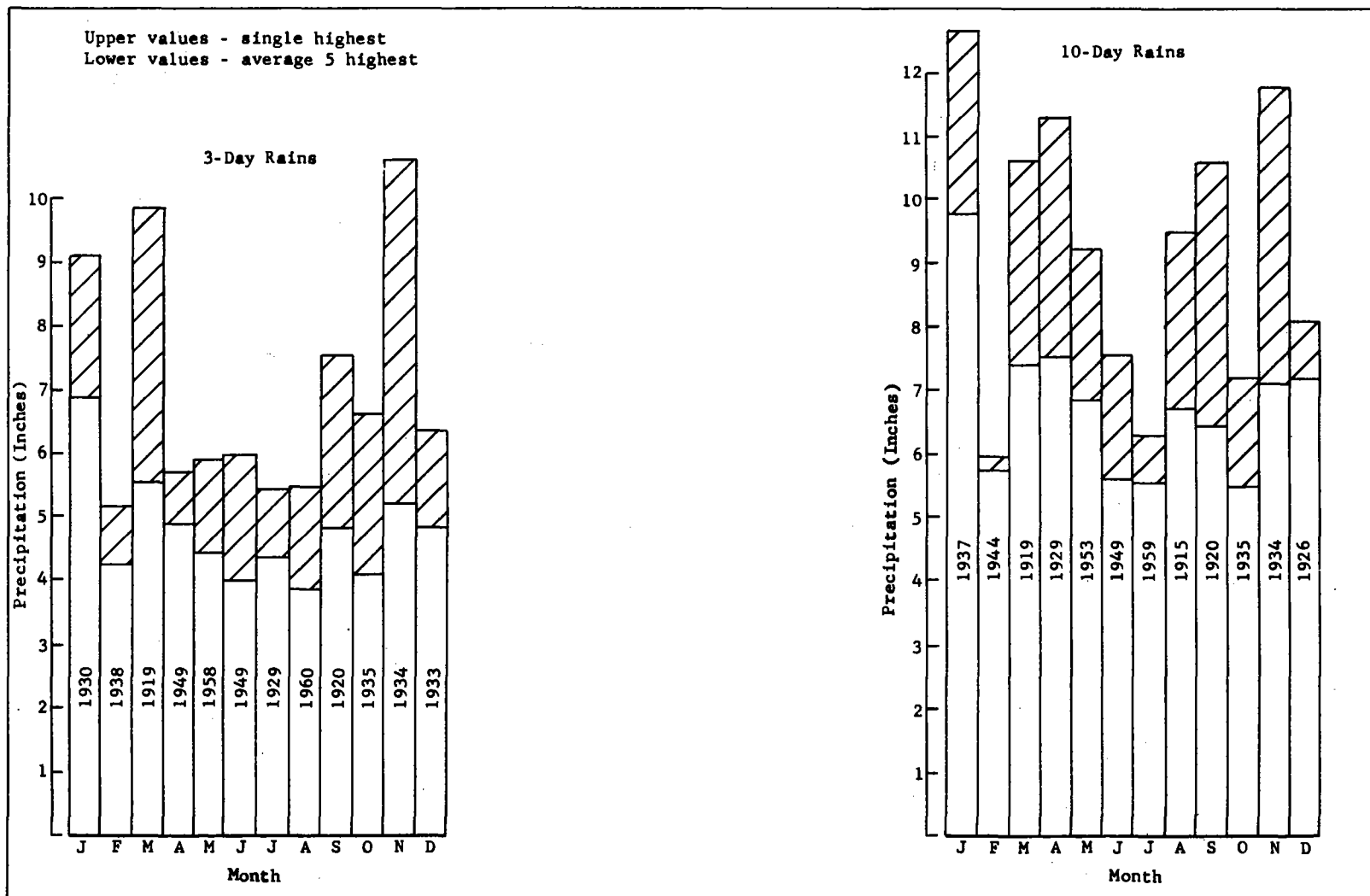
Figure 3-7. Extreme 3- and 10-day rains - Memphis (1912-1961)
