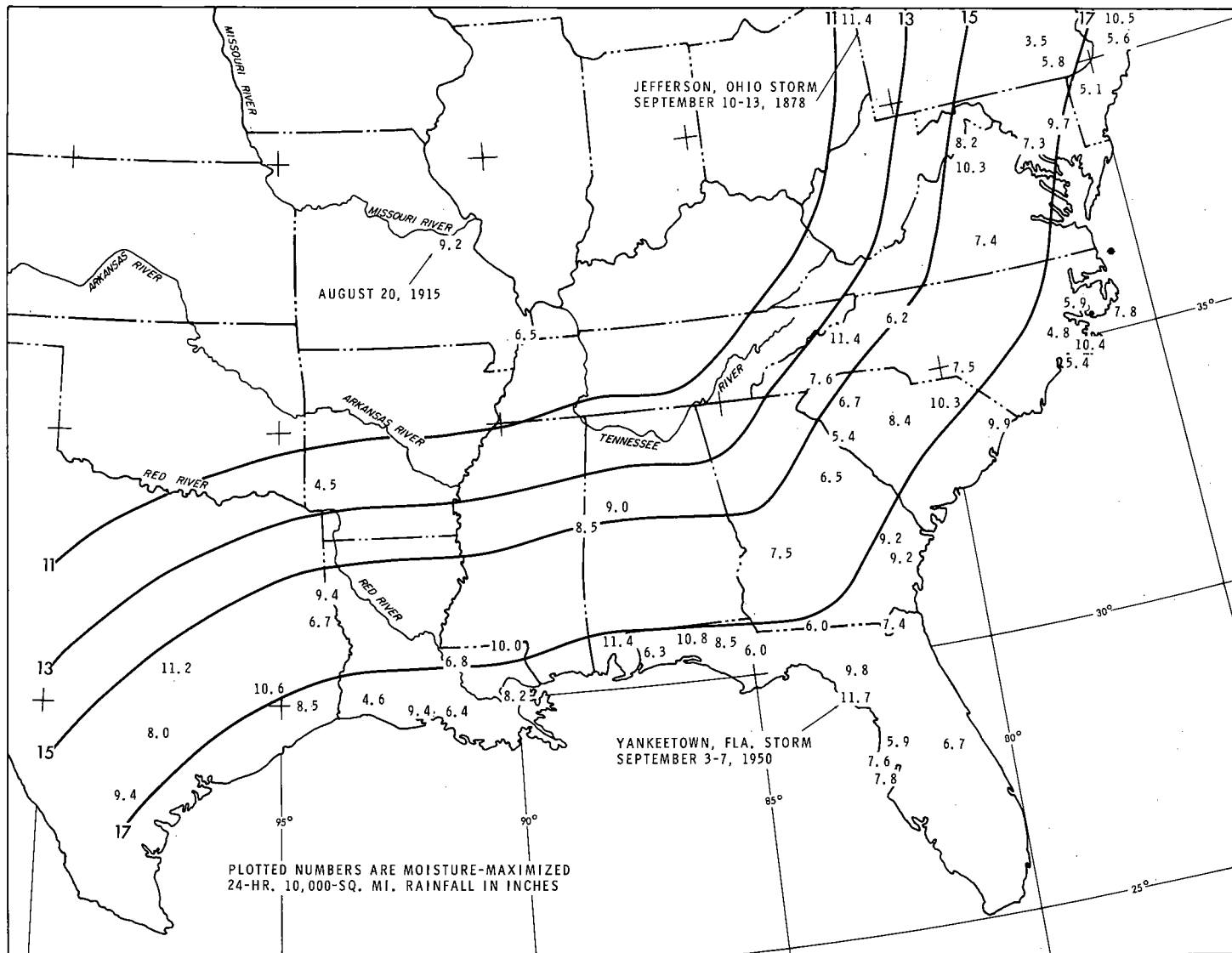
Figure 5-5. Distance-from-coast variation of summer PMP (non-orographic)
