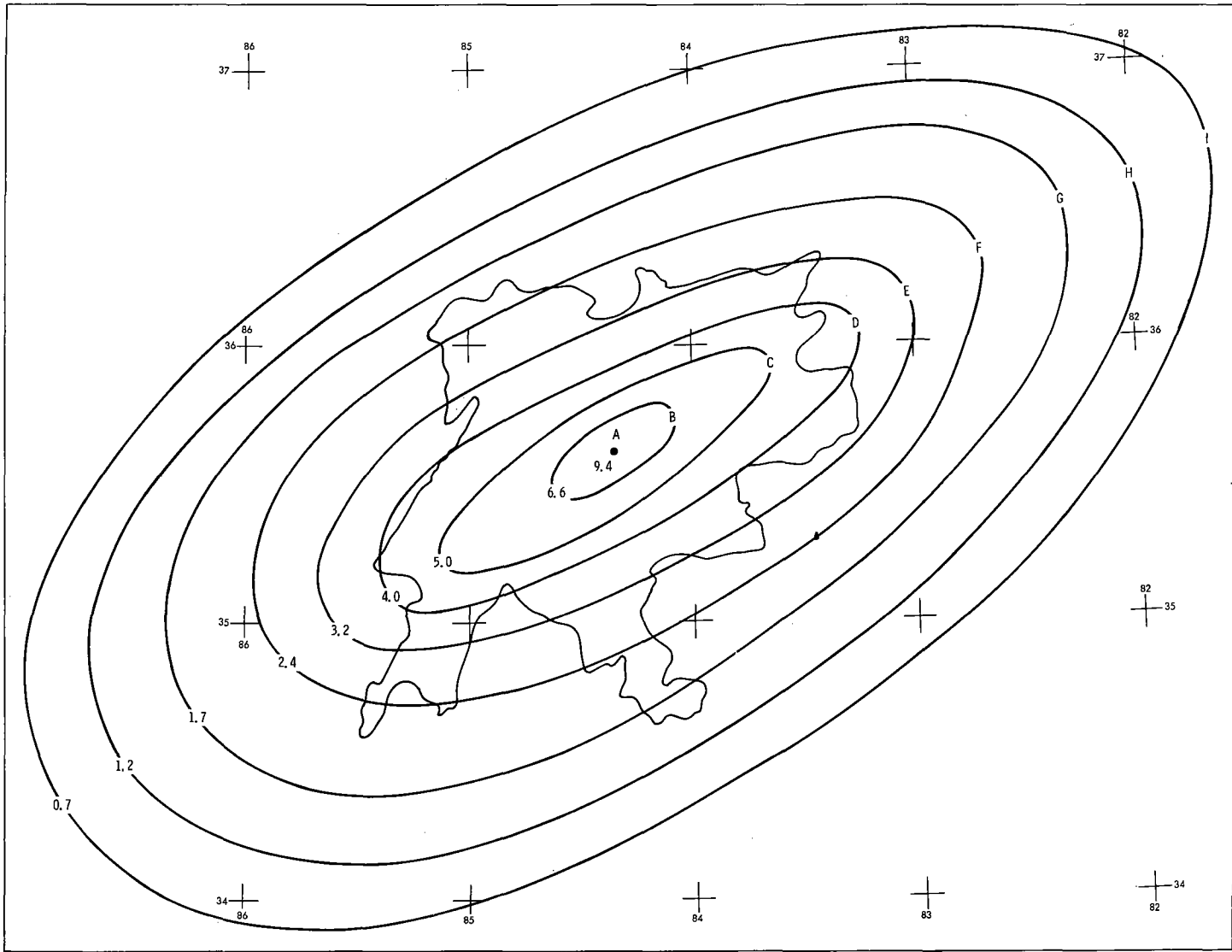
Figure 7-1. TVA March isohyets (7980 sq. mi.), 1st 6 hours
