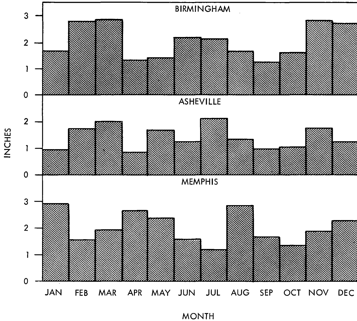
Figure 6-3. Exceedance of 10-day over 3-day rain (mean of 5 highest rains, 1912-1961)
