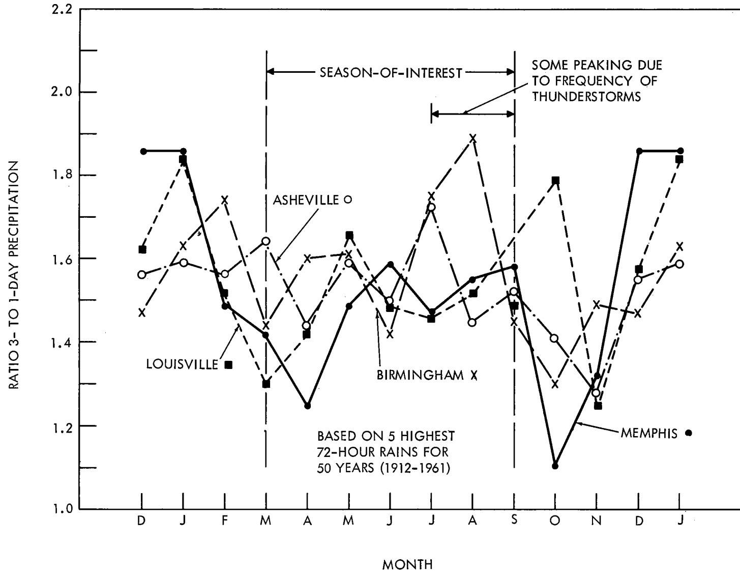
Figure 5-17. Seasonal variation of point 72/24-hr. ratios
