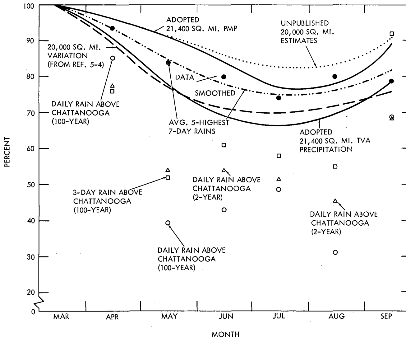
Figure 5-6. Seasonal variation of rainfall over the upper Tennessee River Basin (in percent of March)
