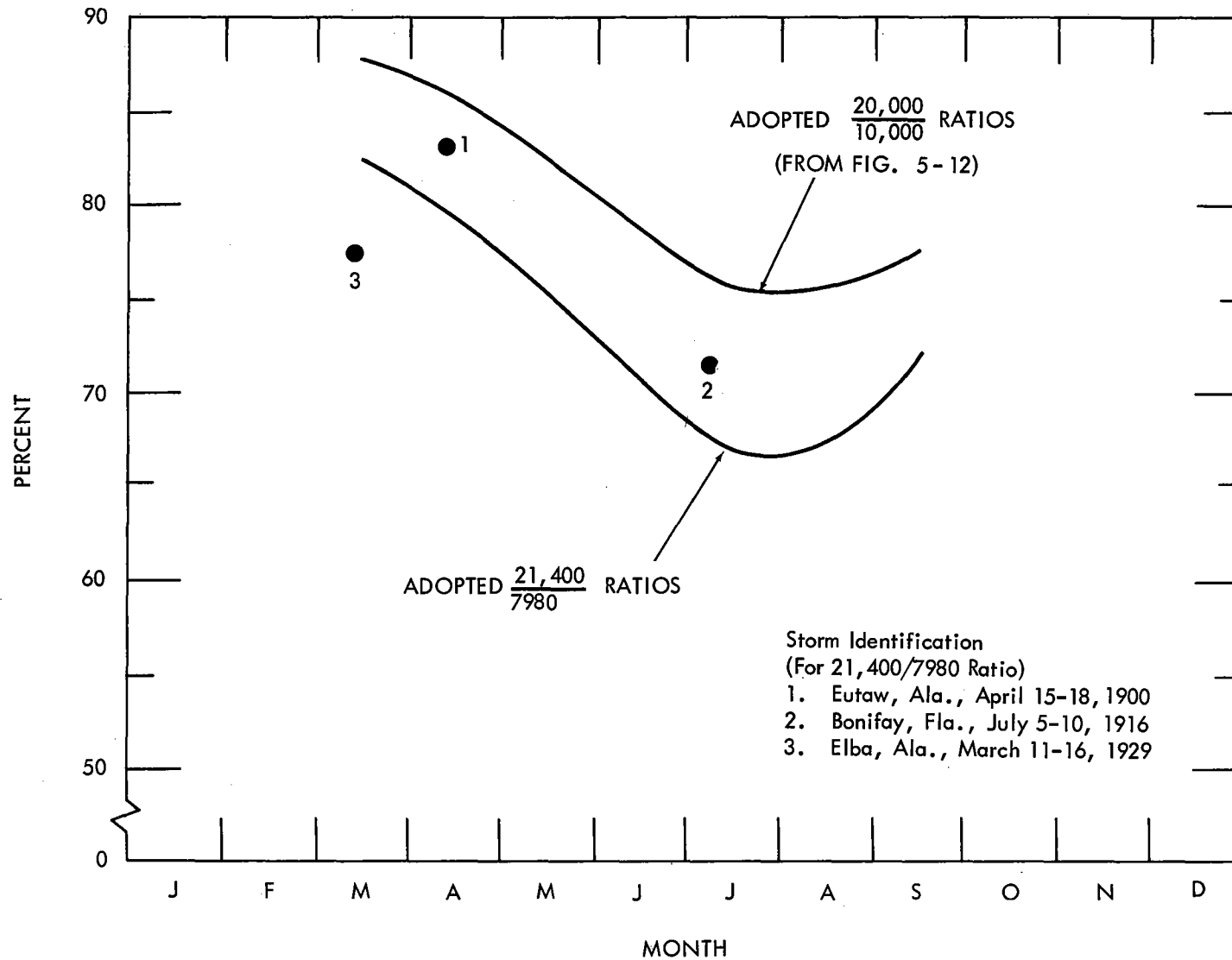
Figure 5-13. Depth-area ratios (21,400/7980-sq. mi.) for 24-hr. rainfall
