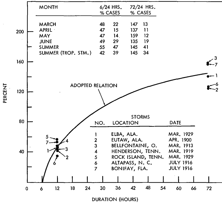
Figure 5-14. Depth-duration in percent of 24 hours (10,000 sq. mi.)
