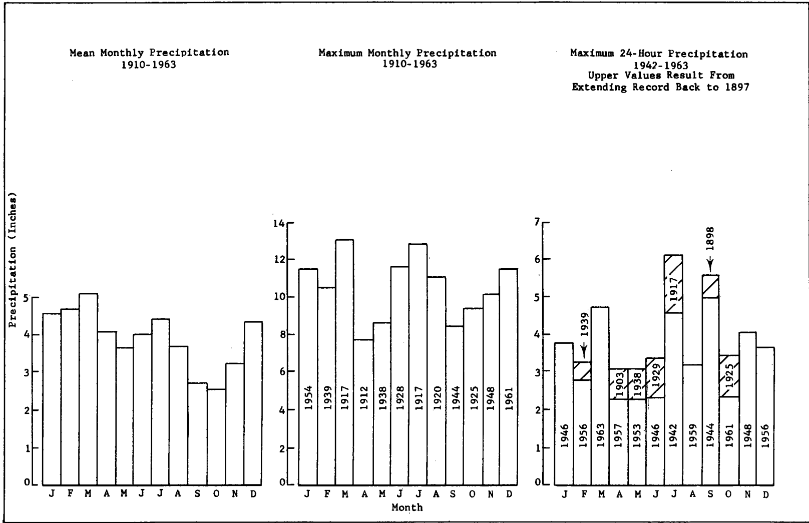
Figure 3-2. Mean and extreme rainfall - Knoxville
