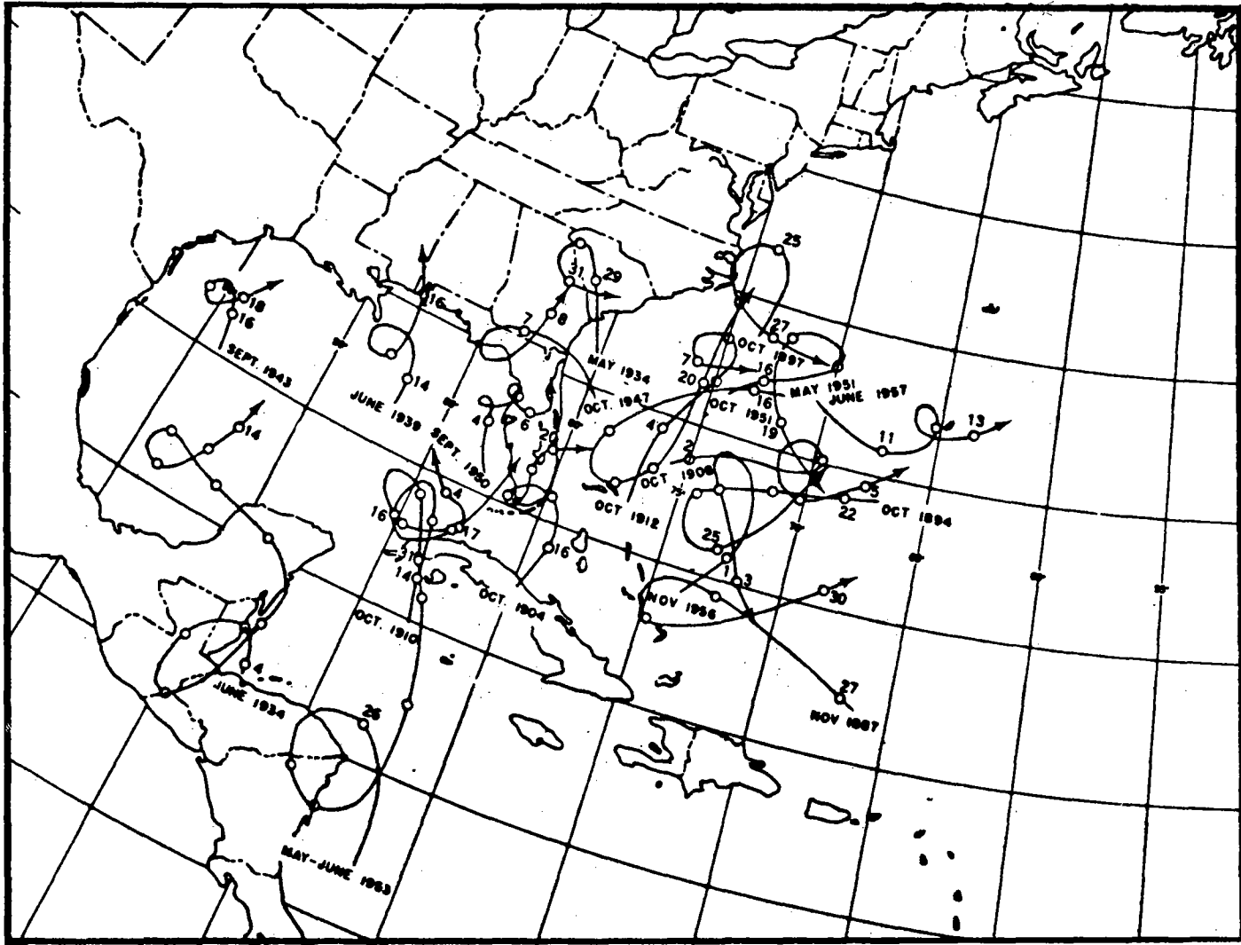
Figure 3-24. Tropical cyclone tracks with counterclockwise loops (from Ref. 3-18)
