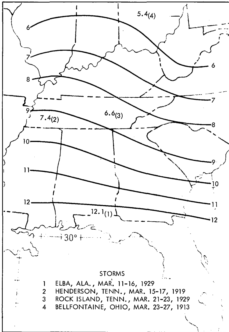
Figure 5-2. March 24-hr. 10,000-sq.mi. TVA precipitation (in.)
