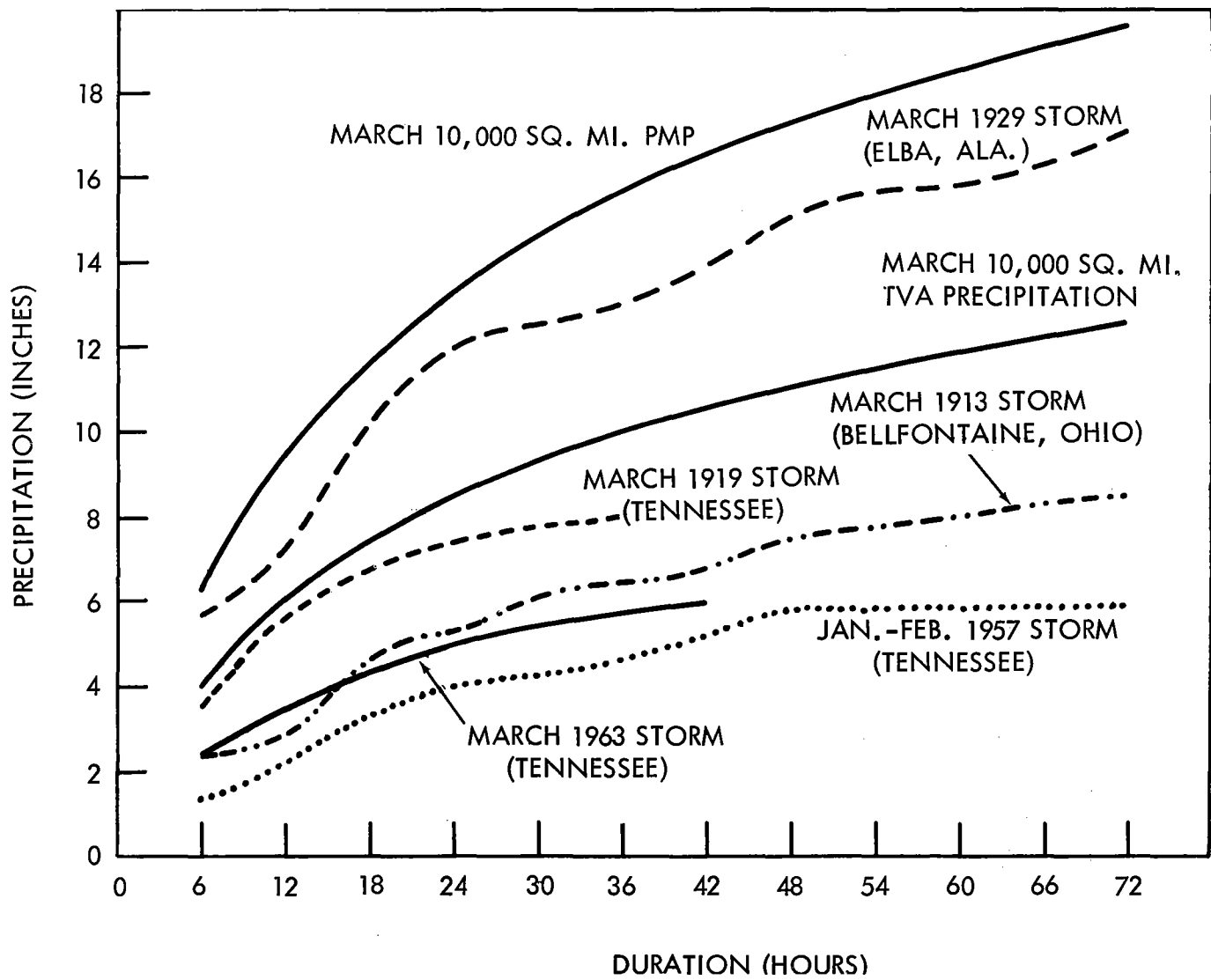
Figure 5-18. Depth-duration rainfall comparisons
