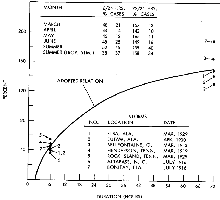
Figure 5-15. Depth-duration in percent of 24 hours (20,000 sq. mi.)
