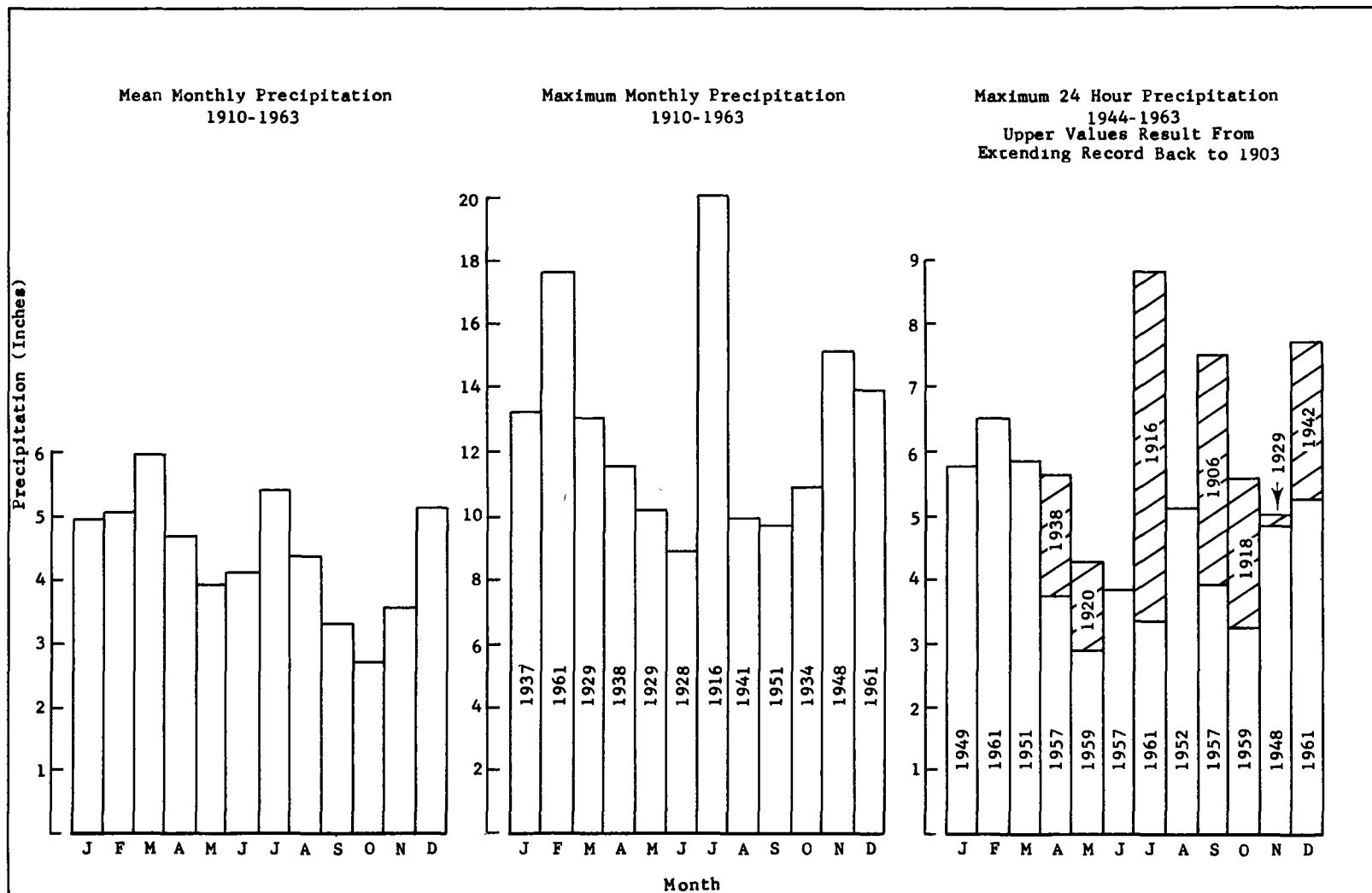
Figure 3-5. Mean and extreme rainfall - Birmingham
