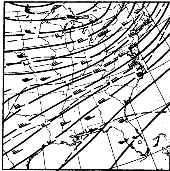
(500 mb) February 22, 1962
