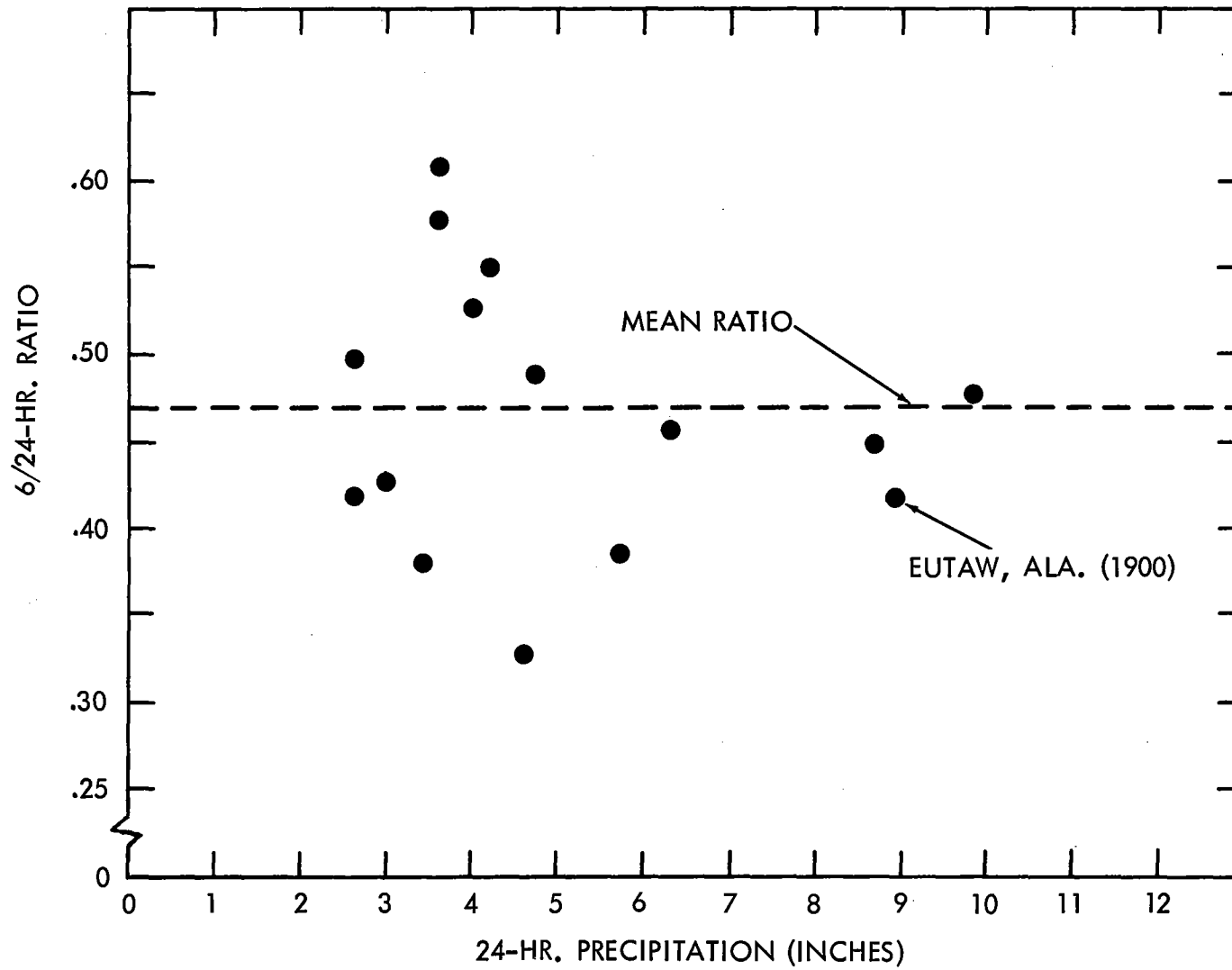
Figure 5-16. 10,000-sq. mi. 24-hr. 6/24-hr. ratio (April)
