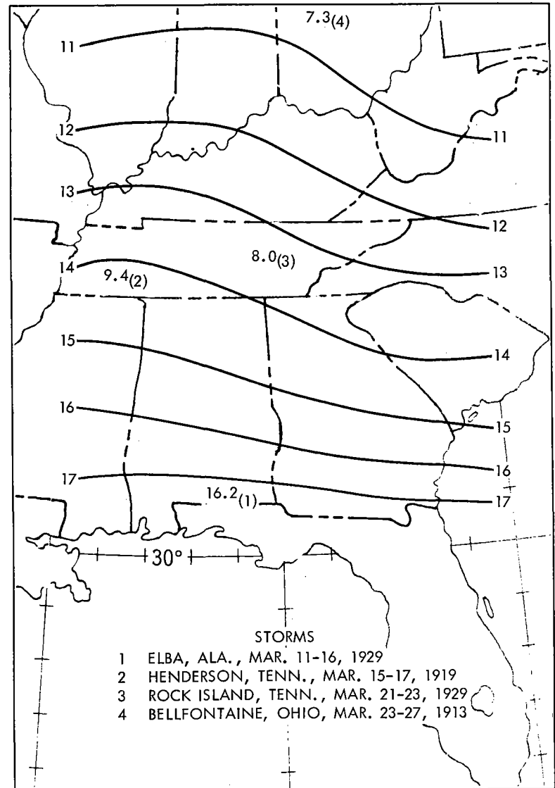
Figure 5-3. March 24-hr. 10,000-sq. mi. PMP (in.)
