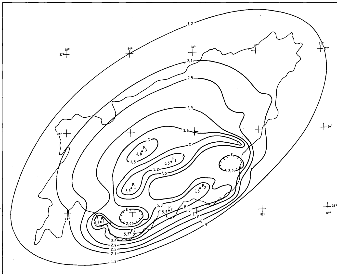
Figure 7-3. TVA March isohyets (21,400-sq. mi. downstream), 1st 6 hours
