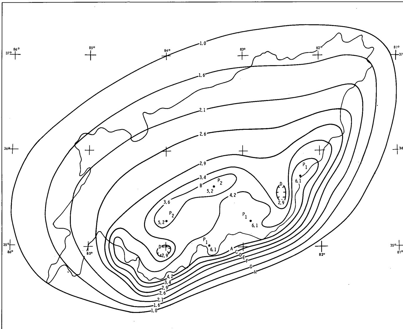
Figure 7-5. TVA March isohyets (21,400-sq. mi. upstream), lst 6 hours
