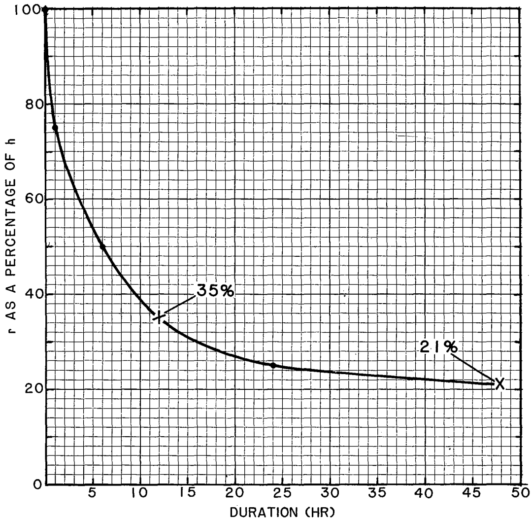
Figure 12.--Relation of length of core event (r) to a duration of greater or equal length (h) for the Upper Deerfield River basin. The "X's" indicate the interpolated and extrapolated values.
