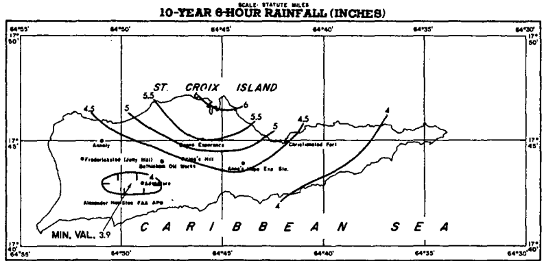
FIGURE 4-87.—10-yr. 6-hr. rainfall for Virgin Islands (in.).
