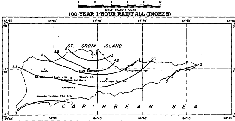
FIGURE 4-69.—100-yr. 1-hr. rainfall for Virgin Islands (in.).
