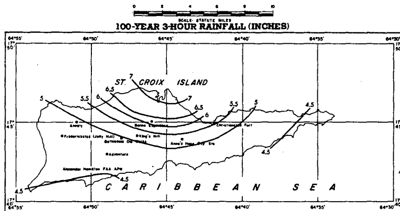
FIGURE 4-83.—100-yr. 3-hr. rainfall for Virgin Islands (in.).
