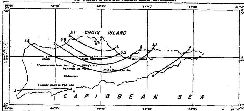
FIGURE 4-82.—50-yr. 3-hr. rainfall for Virgin Islands (in.).
