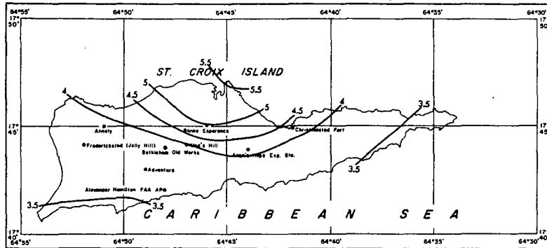
FIGURE 4-81.—25-yr. 3-hr. rainfall for Virgin Islands (in.).
