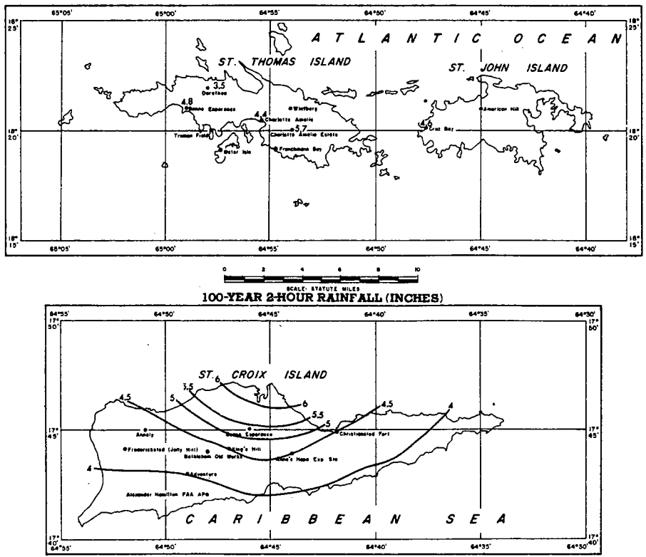
FIGURE 4-76.—100-yr. 2-hr. rainfall for Virgin Islands (in.).
