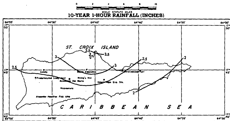
FIGURE 4-66.—10-yr. 1-hr. rainfall for Virgin Islands (in.).
