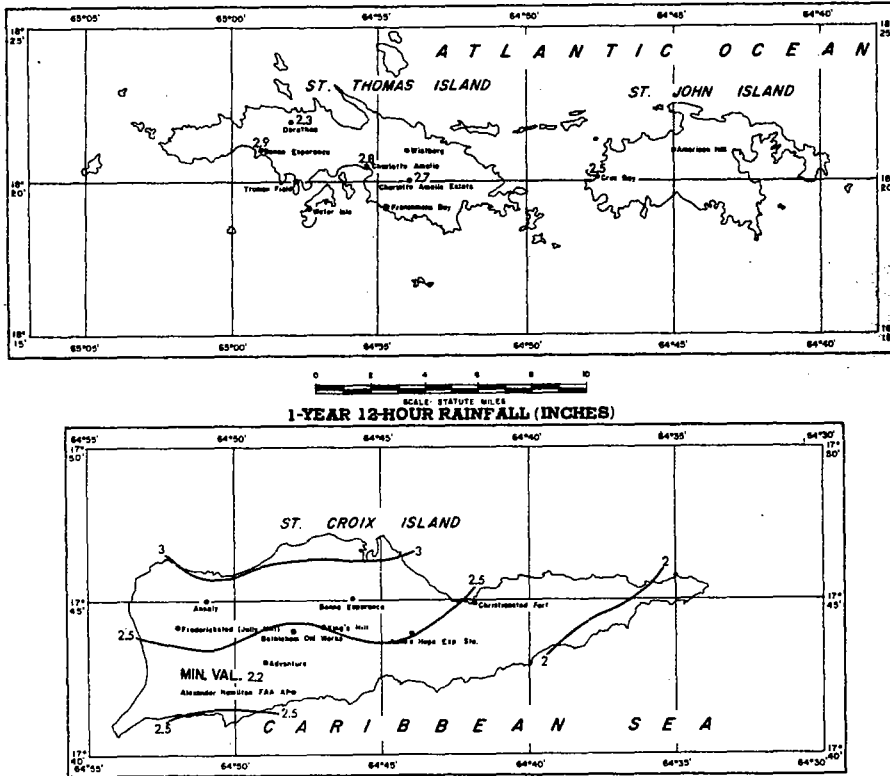
FIGURE 4-91.—1-yr. 12-hr. rainfall for Virgin Islands (in.).
