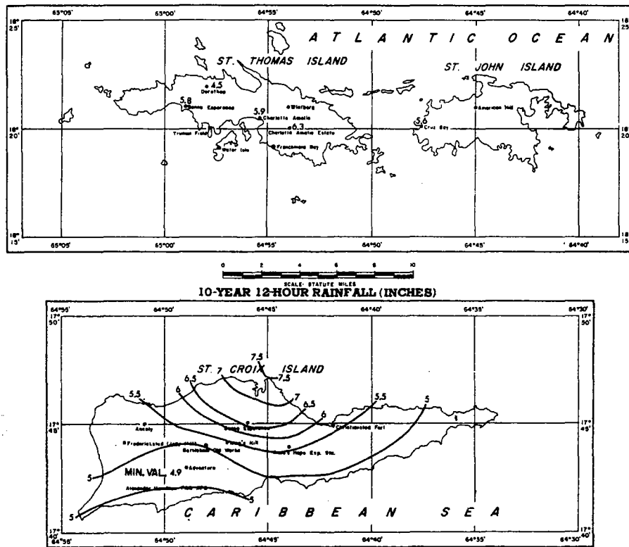
FIGURE 4-94.—10-yr. 12-hr. rainfall for Virgin Islands (in.).
