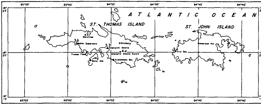
SCALE: STATUTE MILES 50-YEAR 1-HOUR RAINFALL (INCHES)
