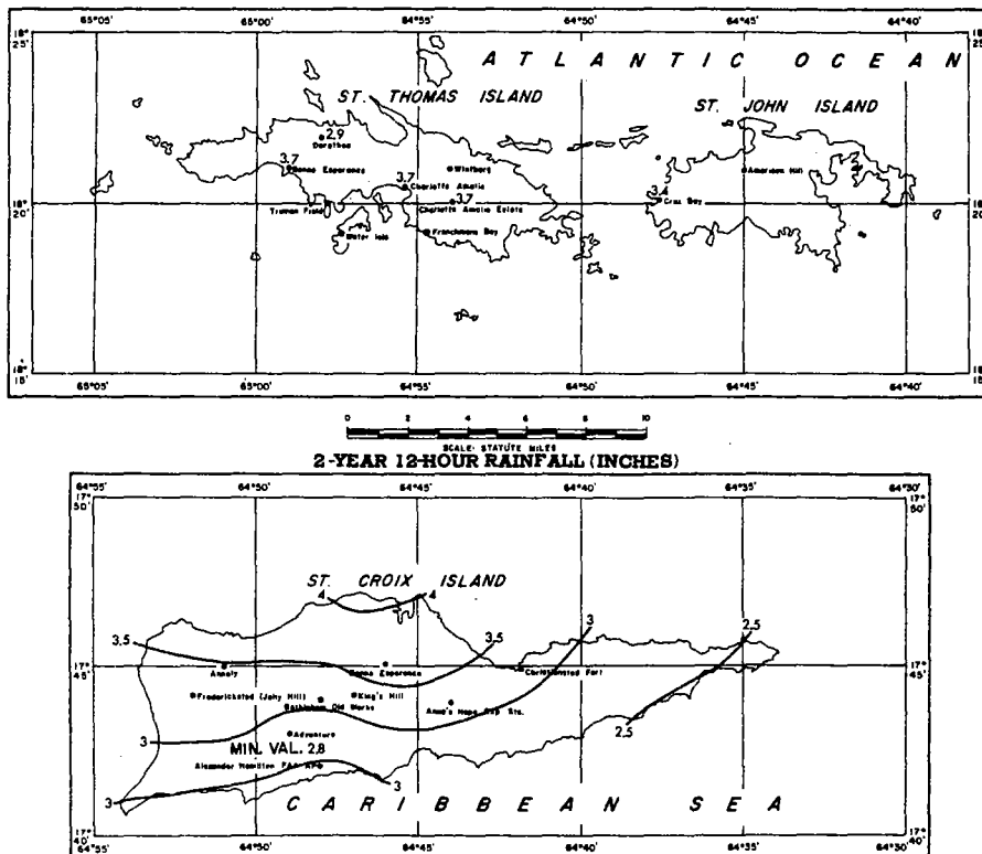
FIGURE 4-92.—2-yr. 12-hr. rainfall for Virgin Islands (in.).
