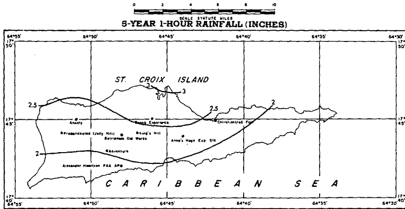
FIGURE 4-65.—5-yr. 1-hr. rainfall for Virgin Islands (in.).
