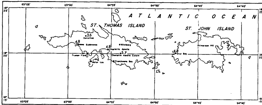
SCALE: STATUTE MILES 50-YEAR 3-HOUR RAINFALL (INCHES)
