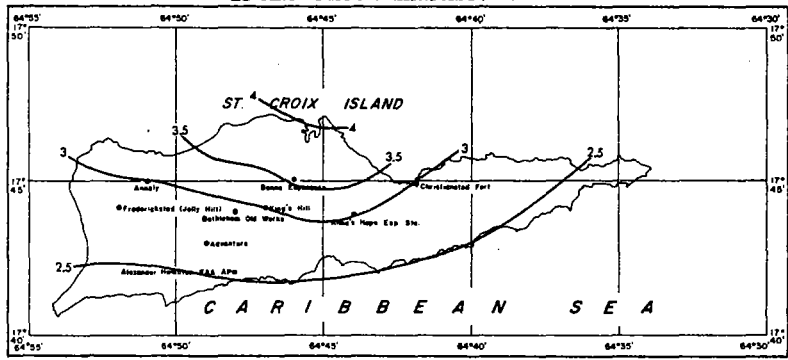
FIGURE 4-67.—25-yr. 1-hr. rainfall for Virgin Islands (in.).
