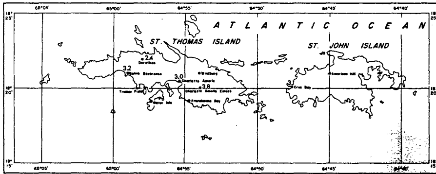
SCALE: STATUTE MILES 25-YEAR 1-HOUR RAINFALL (INCHES)
