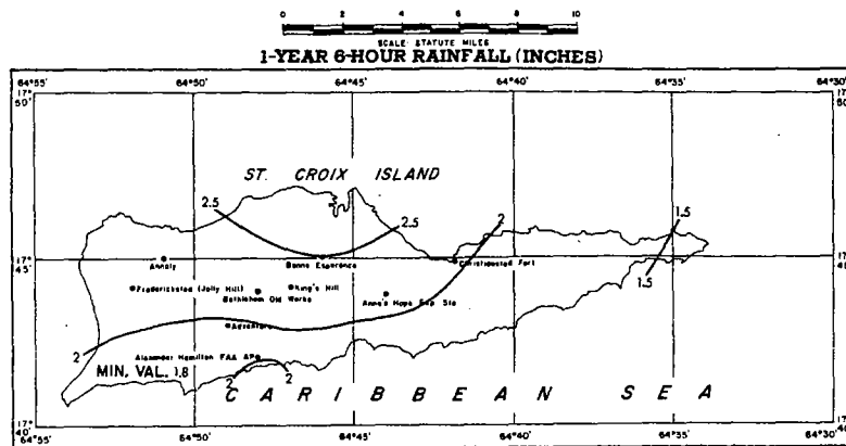
FIGURE 4-84.—1-yr. 6-hr. rainfall for Virgin Islands (in.).
