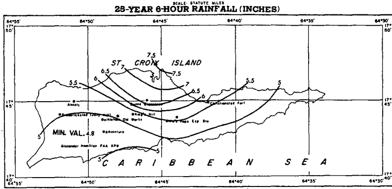
FIGURE 4-88.—25-yr. 6-hr. rainfall for Virgin Islands (in.)
