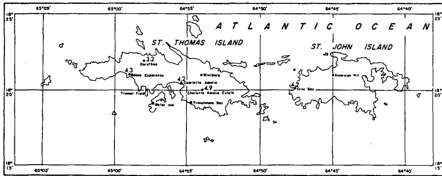
SCALE: STATUTE MILES 25-YEAR 3-HOUR RAINFALL (INCHES)
