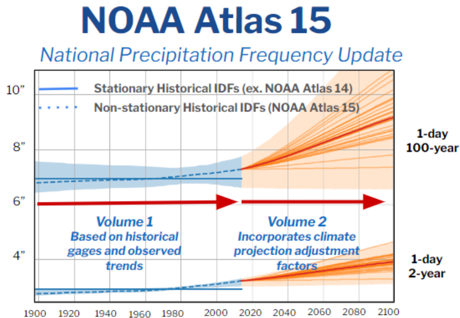
Figure 6. Envision Atlas 15 historical and future intensity-duration-frequency curves (IDFs).
