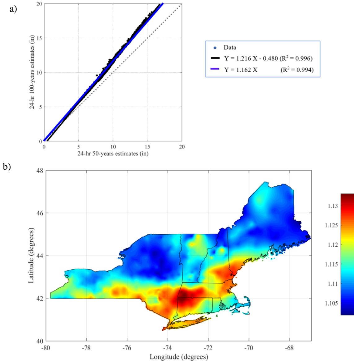
Figure 4.8.1. a) Scatter plot of 100-year versus 50-year 24-hour precipitation frequency estimates. Linear model and zero-intercept linear model regression lines are also shown. b) Spatially interpolated ratios used to calculate 24-hour 100-year precipitation frequency grid from the 24-hour 50-year grid.
