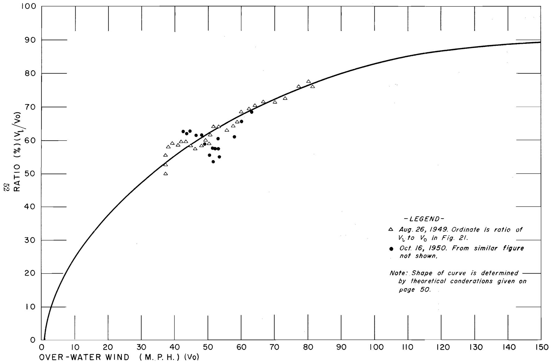
FIG. 30 RATIO OF AVERAGE OFF-LAND WIND TO AVERAGE OVER-WATER WIND
