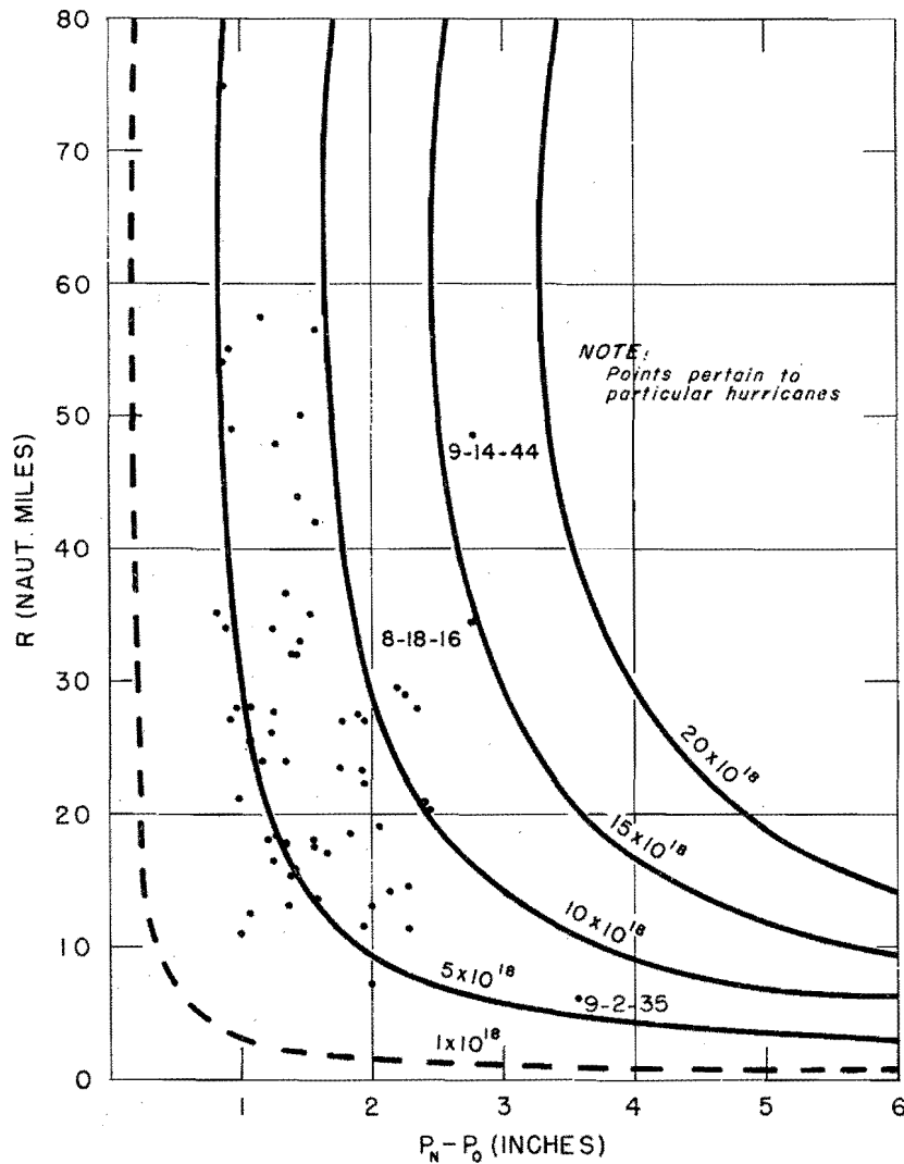
KINETIC ENERGY (ERGS) IN A CIRCULAR LAYER OF 100-NAUTICAL-MILE RADIUS, 1 CM DEEP, AS FUNCTION OF R AND P_N - P_0 .
