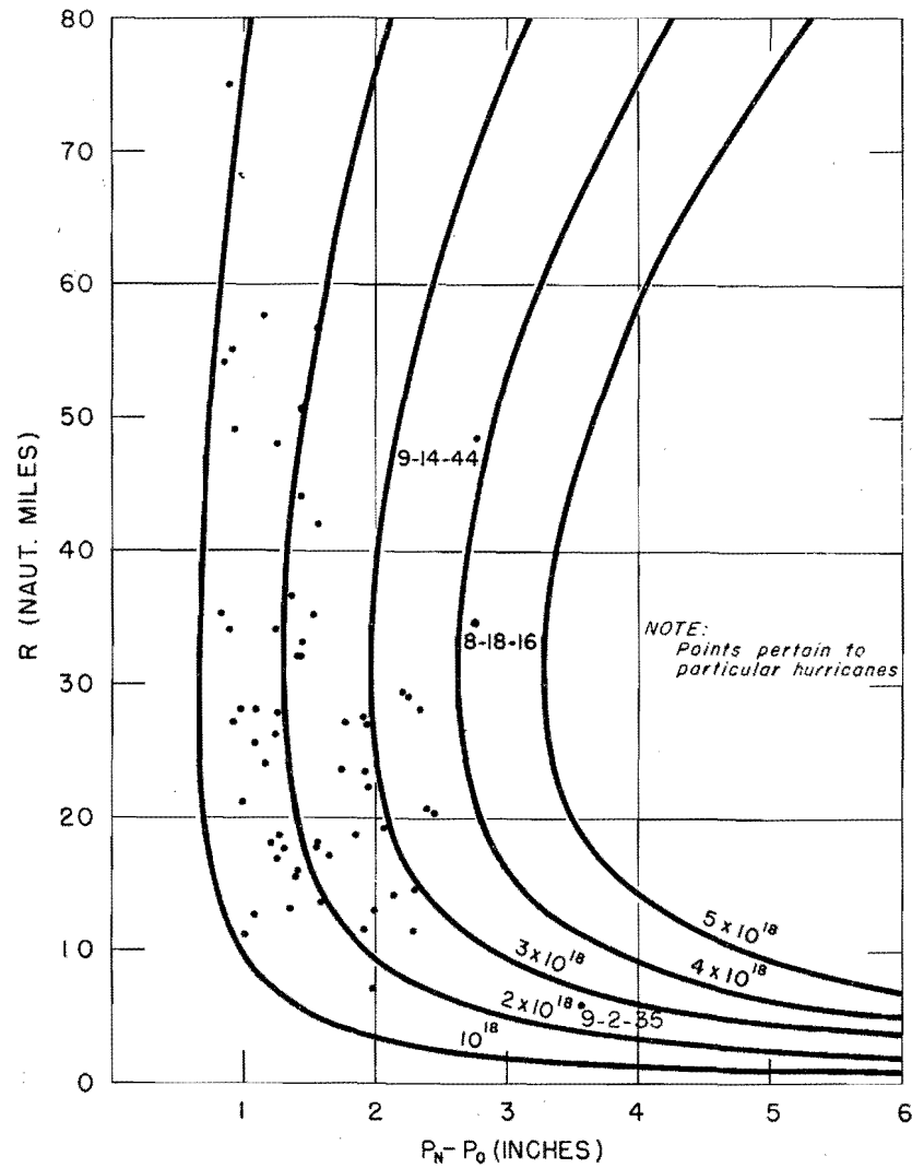
KINETIC ENERGY (ERGS) IN A CIRCULAR LAYER OF 50-NAUTICAL-MILE RADIUS, 1 CM DEEP, AS A FUNCTION OF R AND P_N - P_0 .
