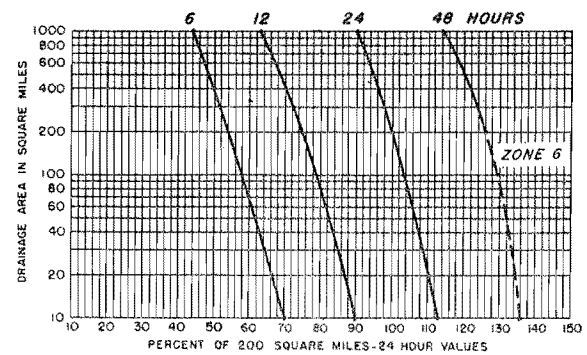
FIGURE B SEASONAL VARIATION DEPTH-AREA-DURATION RELATIONSHIPS
