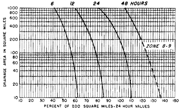
FIGURE 26 SEASONAL VARIATION DEPTH-AREA-DURATION RELATIONSHIPS Percentage to be applied to 200 square miles 24 hour probable maximum precipitation values for: DECEMBER
