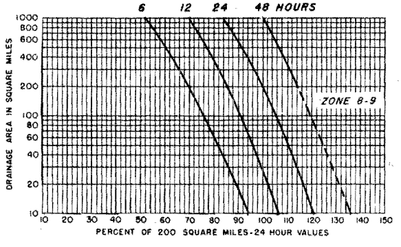
FIGURE 20 SEASONAL VARIATION DEPTH-AREA-DURATION RELATIONSHIPS Percentage to be applied to 200 square miles 24 hour probable maximum precipitation values for: SEPTEMBER
