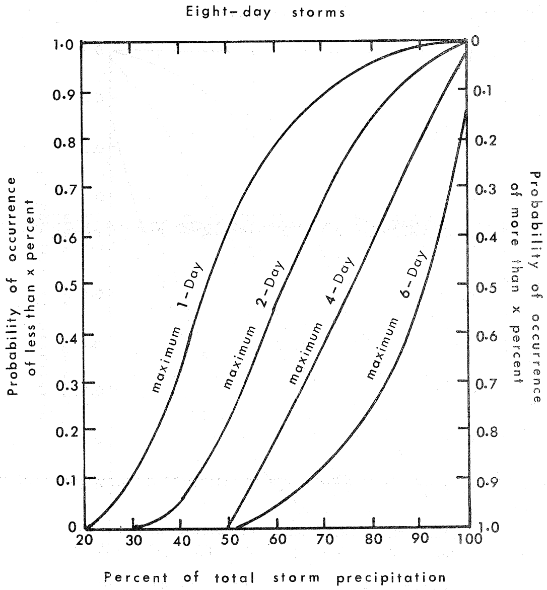
Figure 7. Percent of precipitation observed on maximum M-days within 8-day storm.
