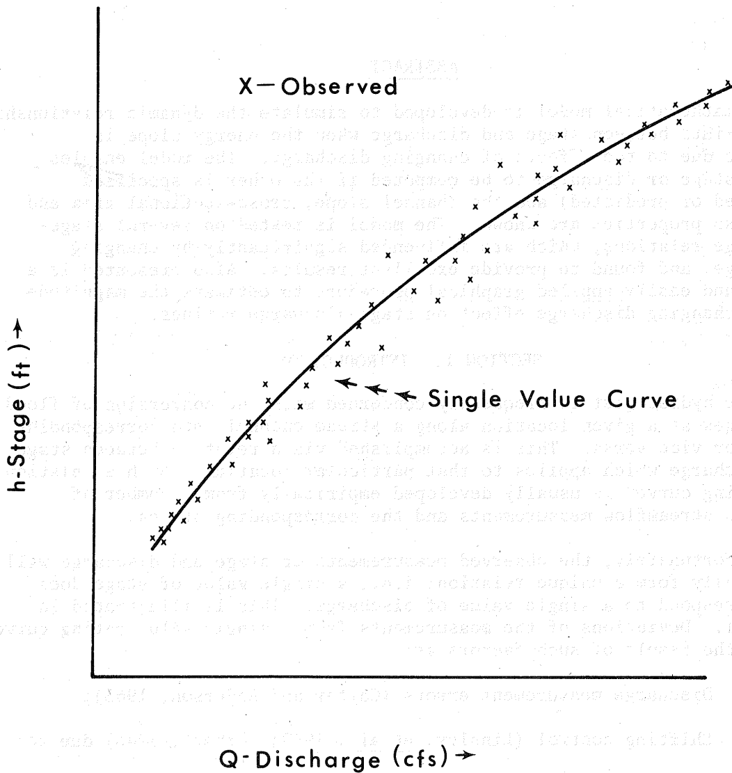
Figure 1. Stage-Discharge Relation.
