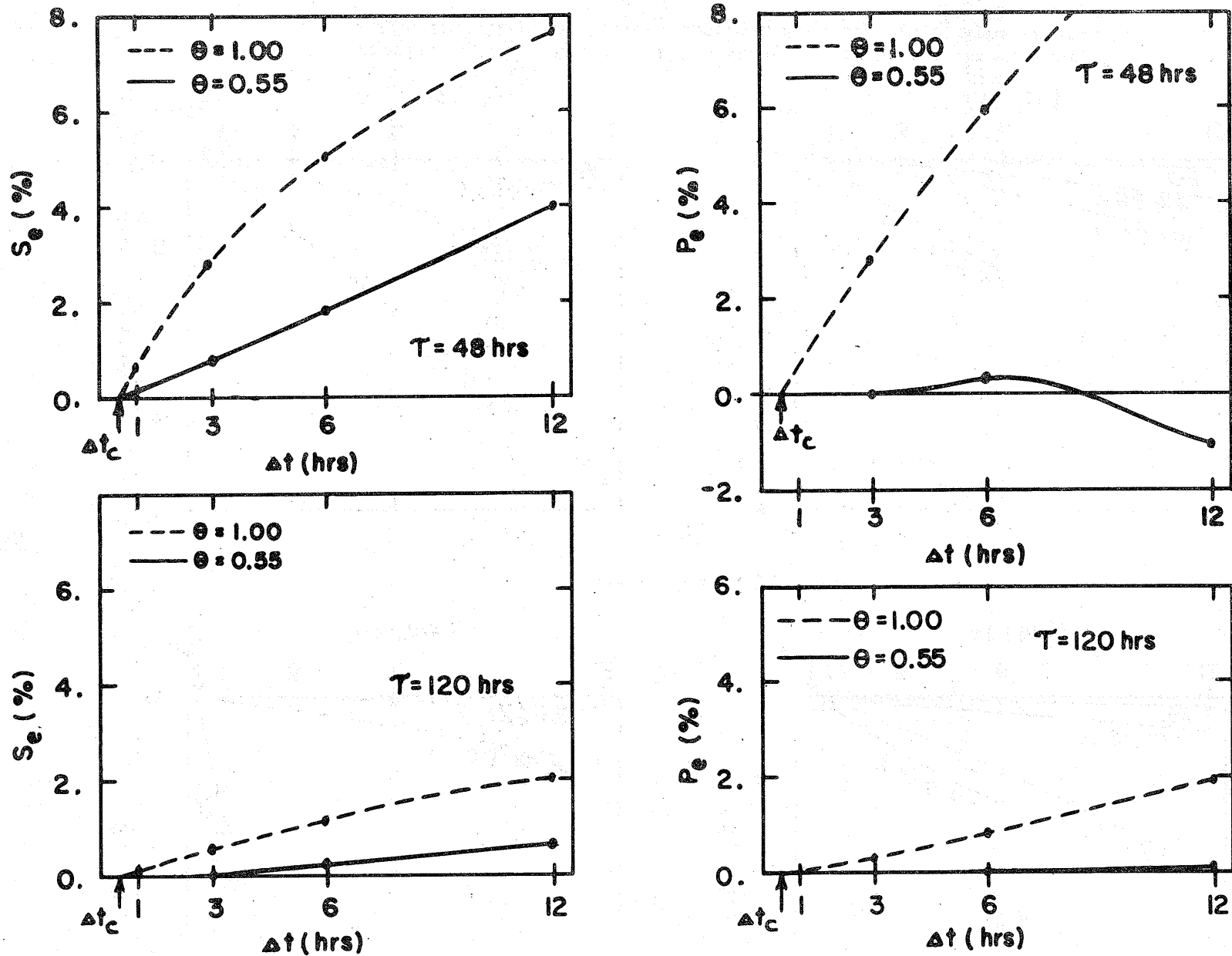
Fig. 8. Effect of \theta and \tau on the Distortion of the Computed Stage Hydrograph at the Downstream Boundary for Various \Delta t Time Steps Having \rho=20 and \gamma=1.2
