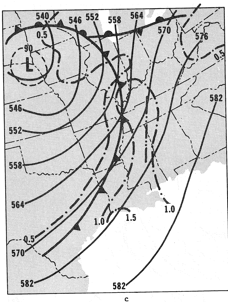
Figures 3c - d--Maps showing 500-mb contours superposed on surface Low(s) and fronts for: (c) 0600 CST April 12, 1974; (d) 1800 CST April 12, 1974. 500-mb heights (solid lines) are given in decameters, precipitable water in the layer from the surface to 500-mb (dashed-dot lines) are in inches; and the closed isobar (dashed line) about the surface Low in mb with the first digit of 9 omitted. Dashed-dot-dot-dashed line denotes squall line.
