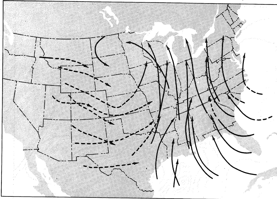
Figure 7a--850-mb 24-hr air parcel trajectory for period ending at 1800 CST April 12, 1974. Dashed arrows indicate descending motion and solid arrows indicate rising motion.
