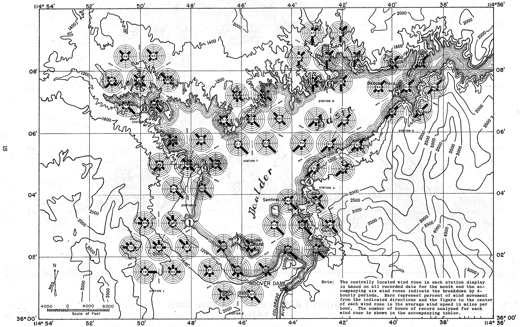
Figure 12 WIND PATTERN OVER LOWER LAKE MEAD MARCH, 1951
