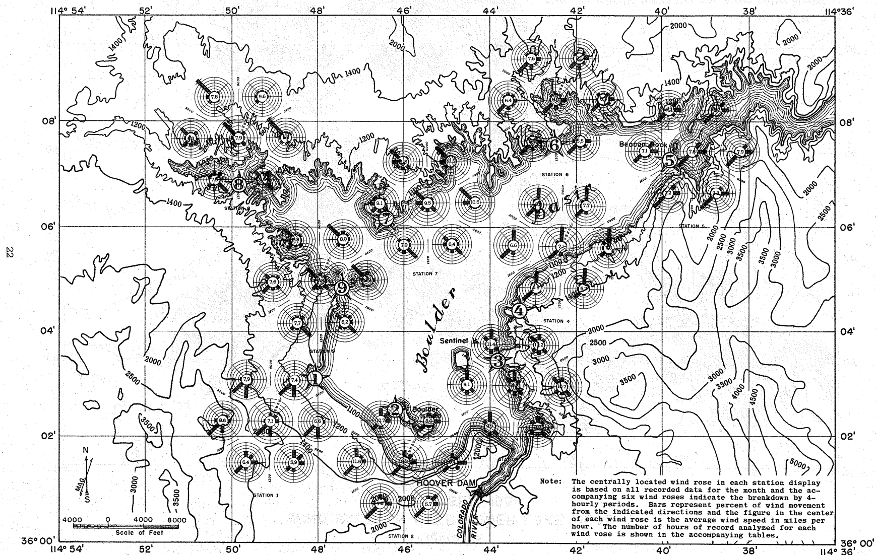
Figure 19 WIND PATTERN OVER LOWER LAKE MEAD OCTOBER, 1951
