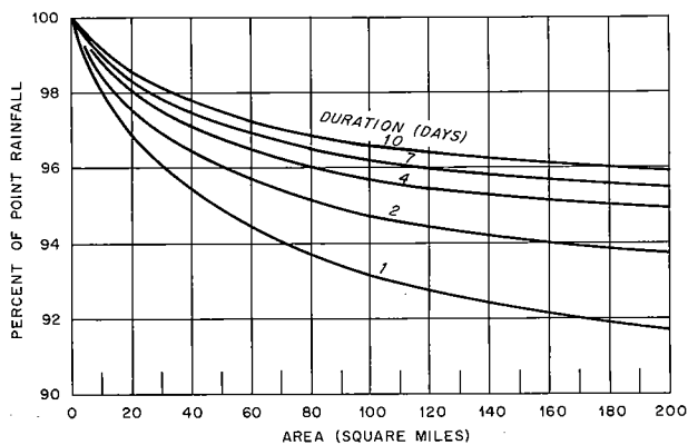
FIGURE 10.—Depth-area curves.
