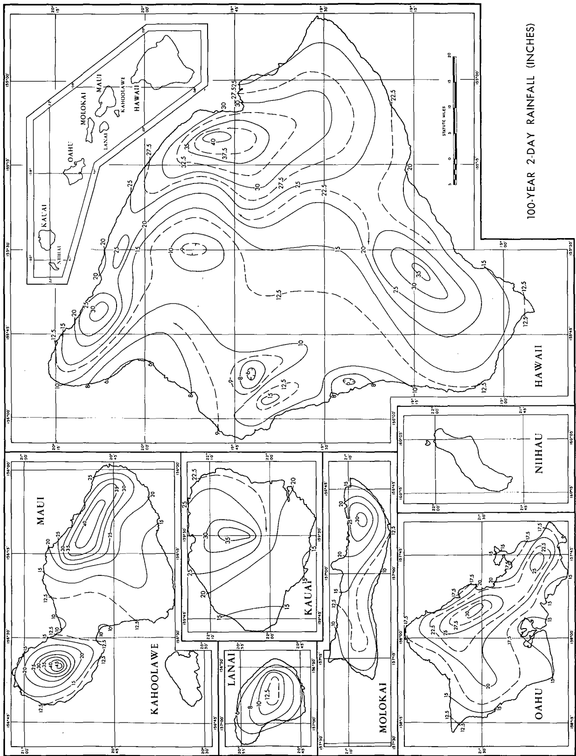
FIGURE 16.—100-year 2-day rainfall (in.).
