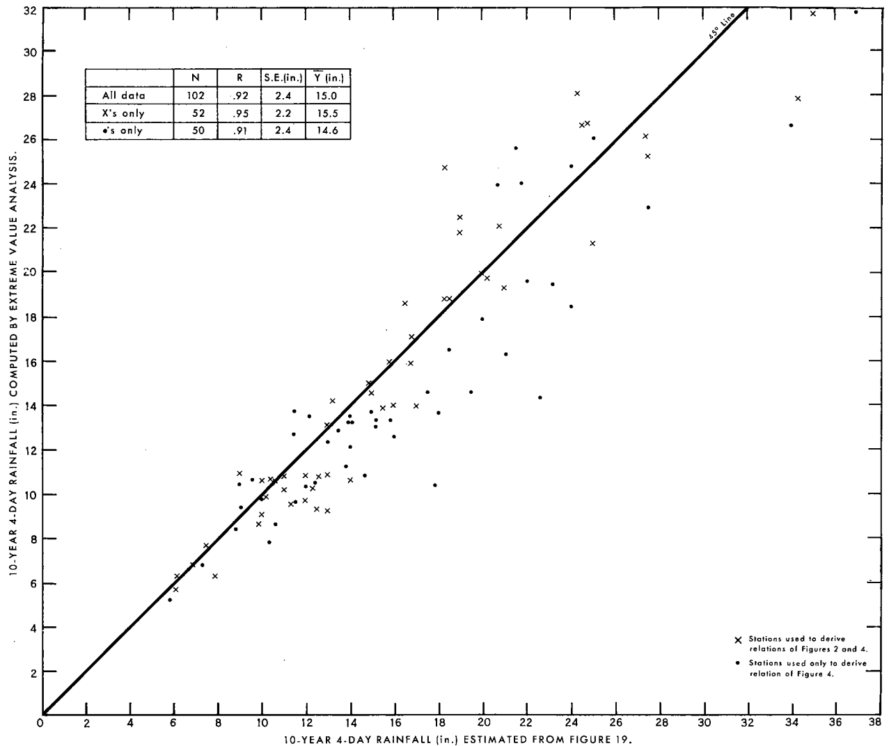
FIGURE 8.—Comparison of estimated vs. computed 10-year 4-day rainfall.
