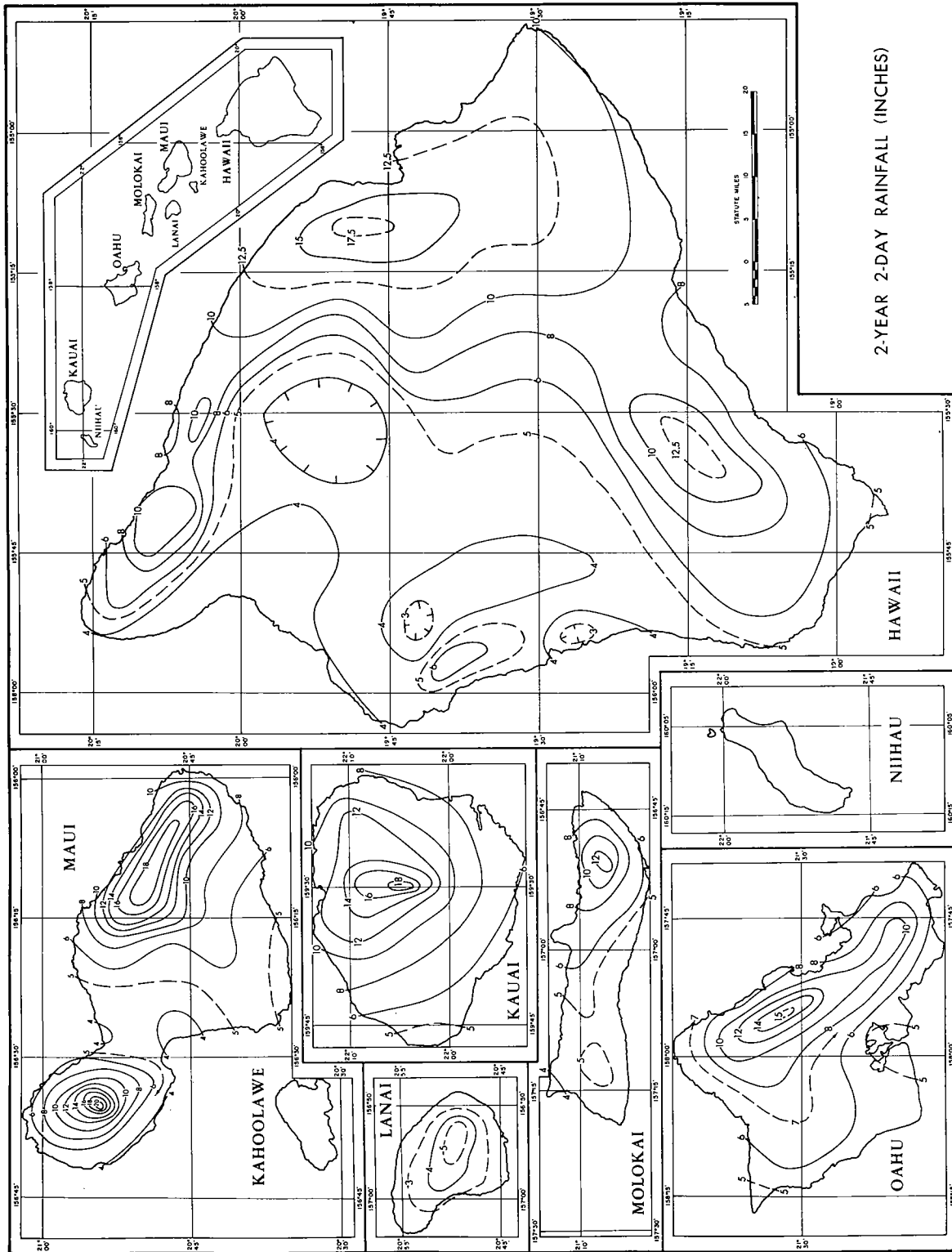
Figure 11.—2-year 2-day rainfall (in.).
