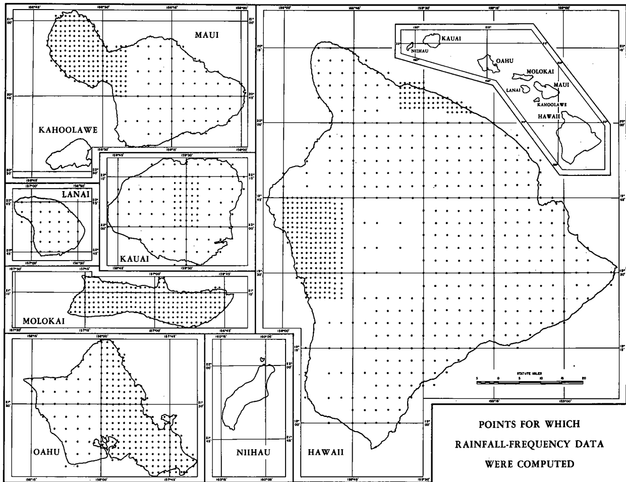
FIGURE 6.—Points for which rainfall-frequency data were computed.
