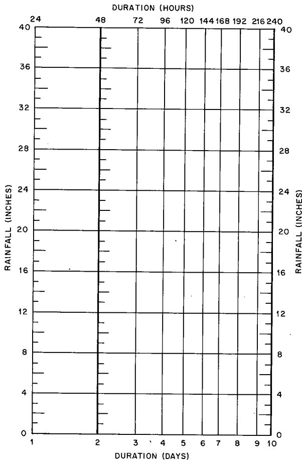
FIGURE 2.—Duration-interpolation diagram.
