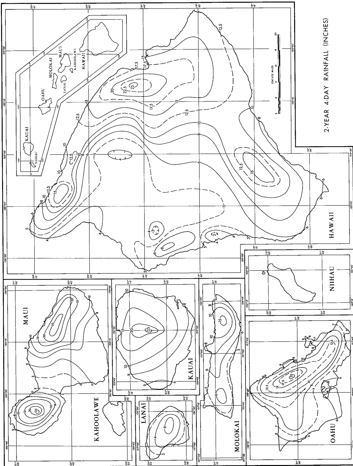
FIGURE 17.—2-year 4-day rainfall (in.).
