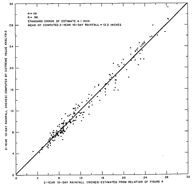
FIGURE 5.—Test of relation of figure 4.
