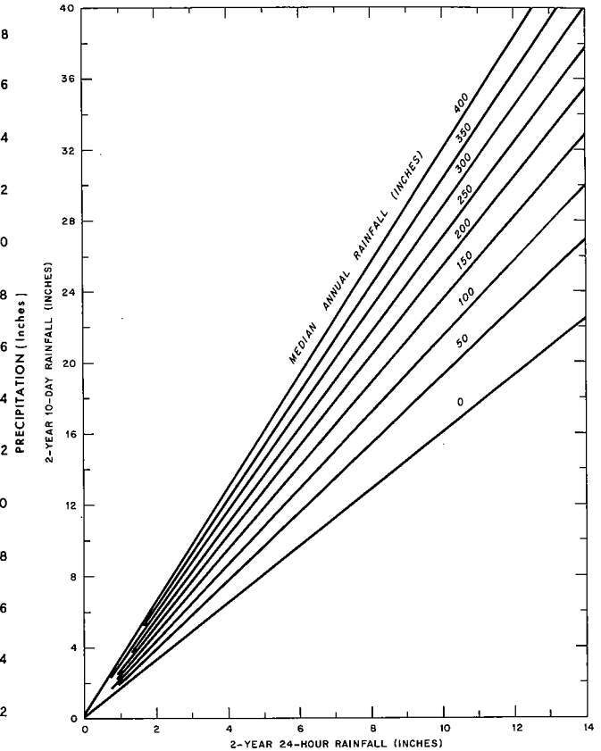
FIGURE 4.—Relation for estimating 2-year 10-day rainfall.
