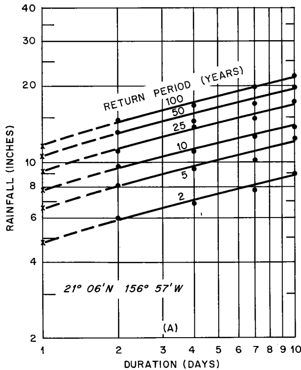
FIGURE 9.—Smoothing values read from isopluvial maps.
