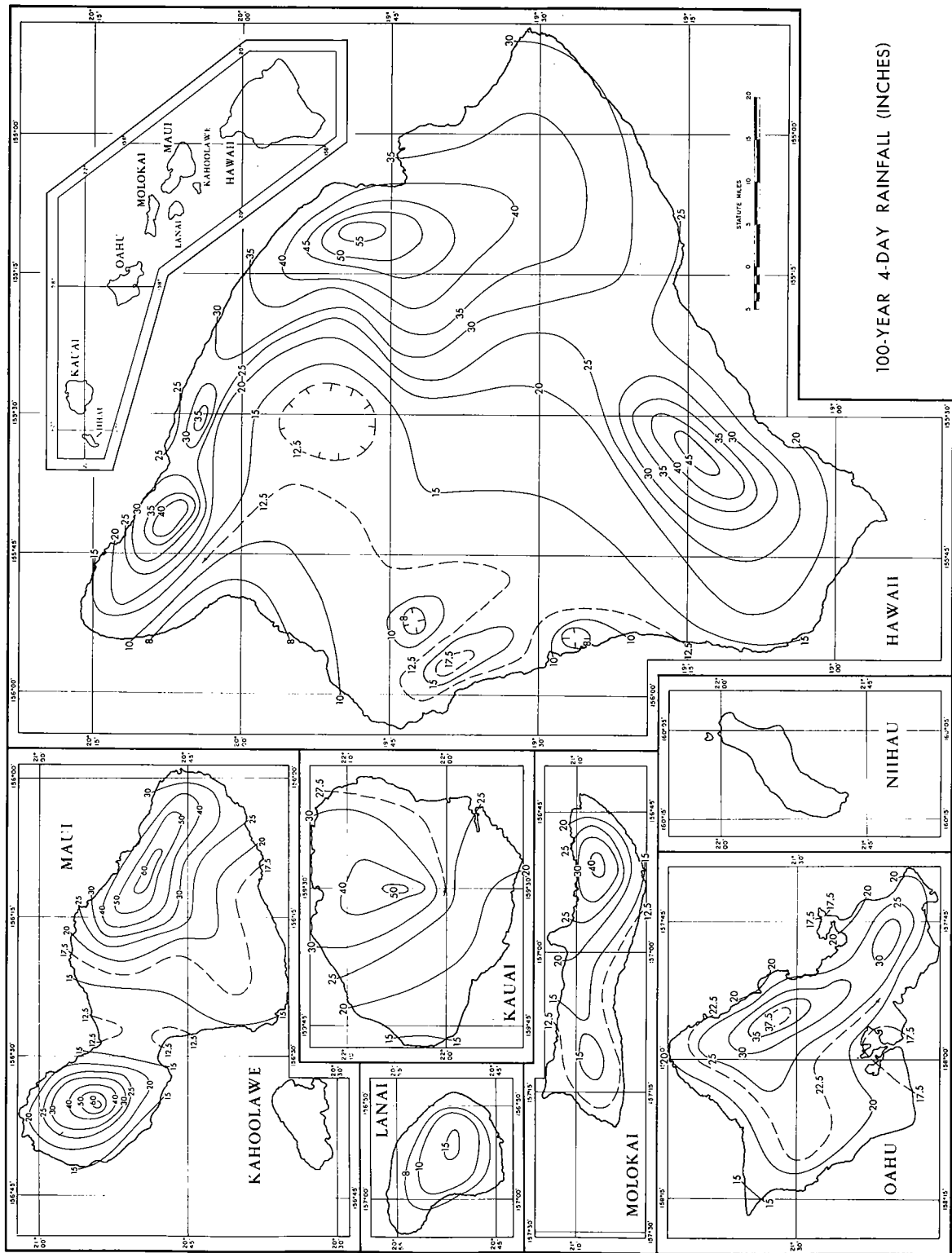
Figure 22.—100-year 4-day rainfall (in.).
