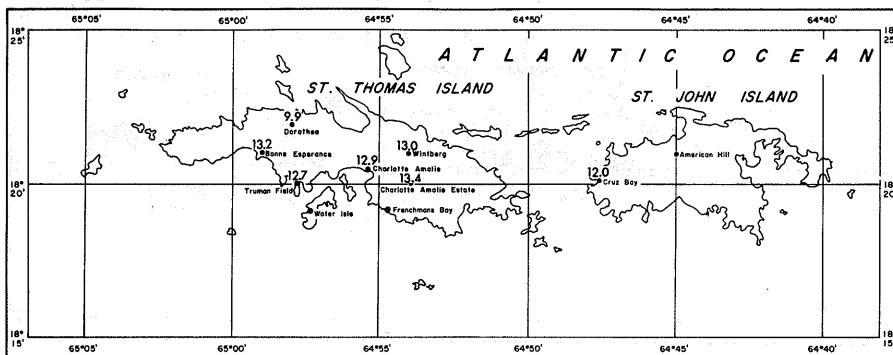
100-YEAR 2-DAY RAINFALL (INCHES)
