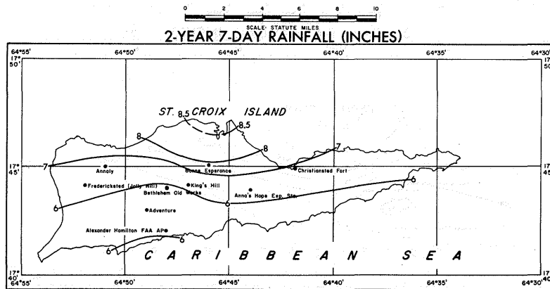
FIGURE 47.—2-year 7-day rainfall (in.) for Virgin Islands.
