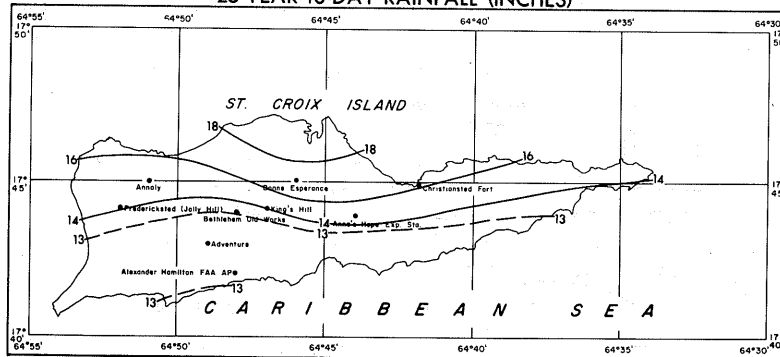
FIGURE 56.—25-year 10-day rainfall (in.) for Virgin Islands.
