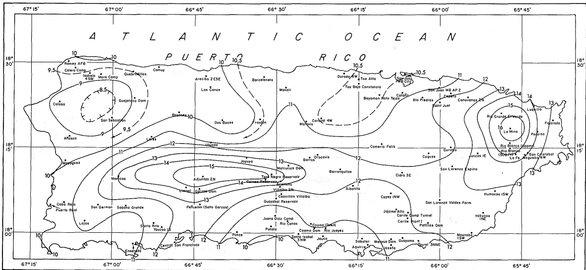
10-YEAR 4-DAY RAINFALL (INCHES)
