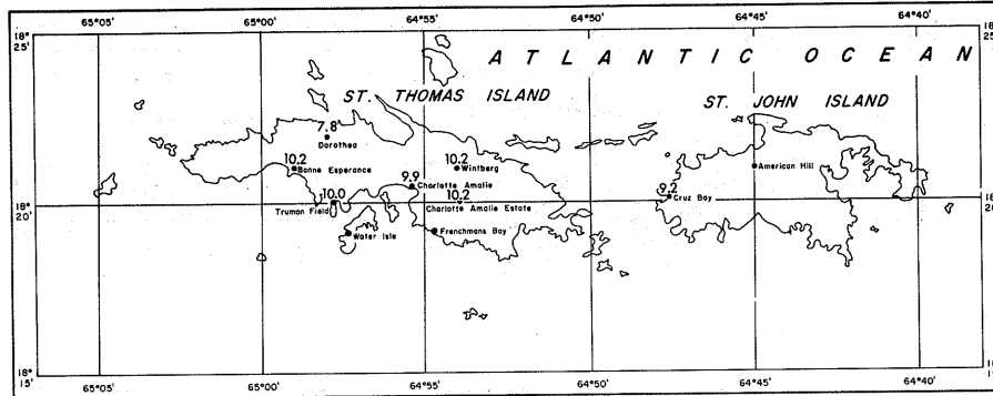
SCALE: STATUTE MILES 25-YEAR 2-DAY RAINFALL (INCHES)
