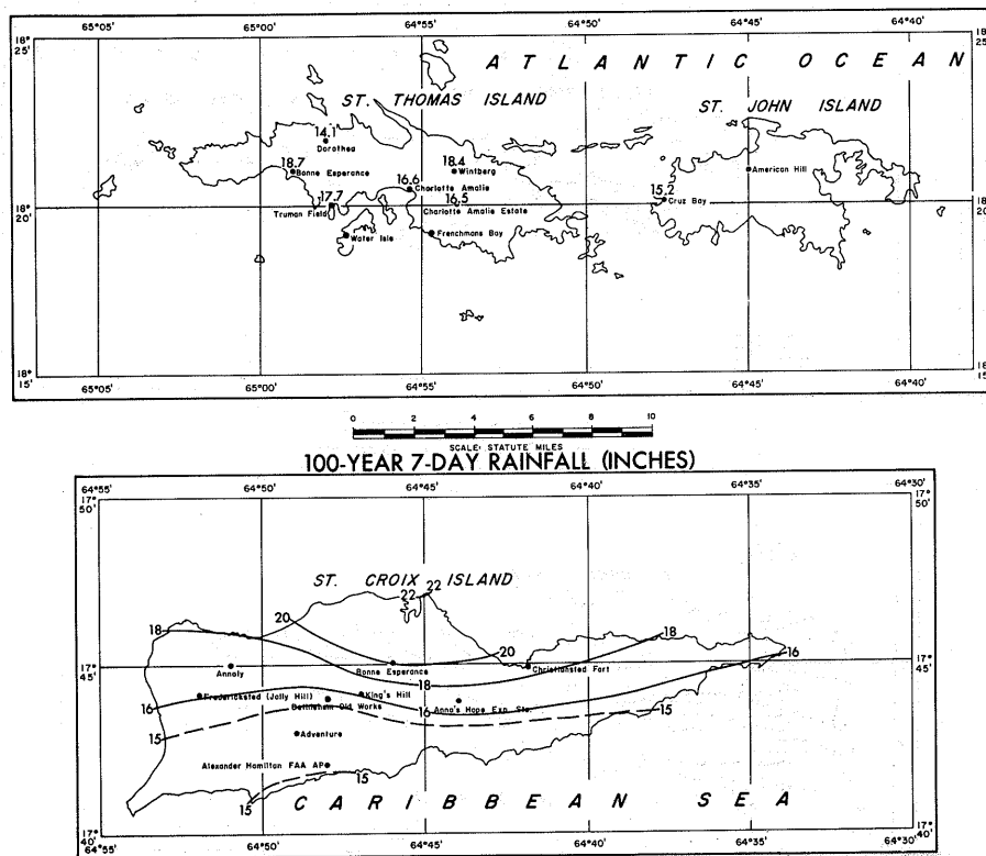
FIGURE 52.—100-year 7-day rainfall (in.) for Virgin Islands.
