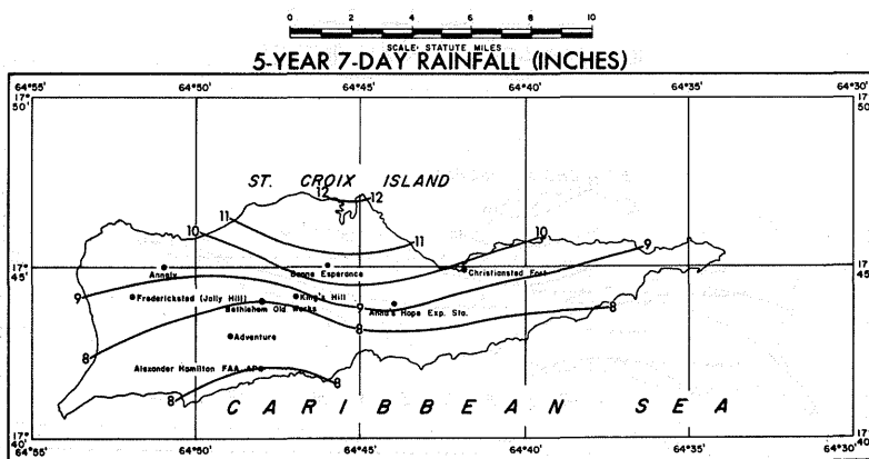
FIGURE 48.—5-year 7-day rainfall (in.) for Virgin Islands.
