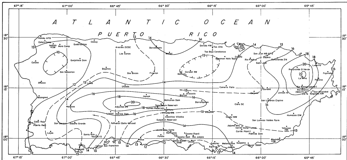
10-YEAR 10-DAY RAINFALL (INCHES)
