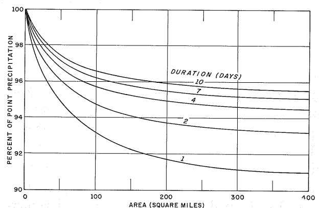
FIGURE 10.—Depth-area curves.
