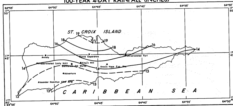
FIGURE 46.—100-year 4-day rainfall (in.) for Virgin Islands.
