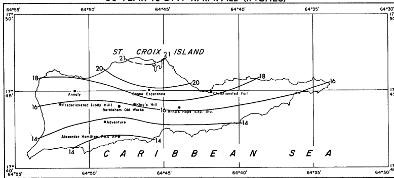
FIGURE 57.—50-year 10-day rainfall (in.) for Virgin Islands.
