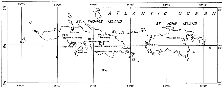
FIGURE 57.—50-year 10-day rainfall (in.) for Virgin Islands.
