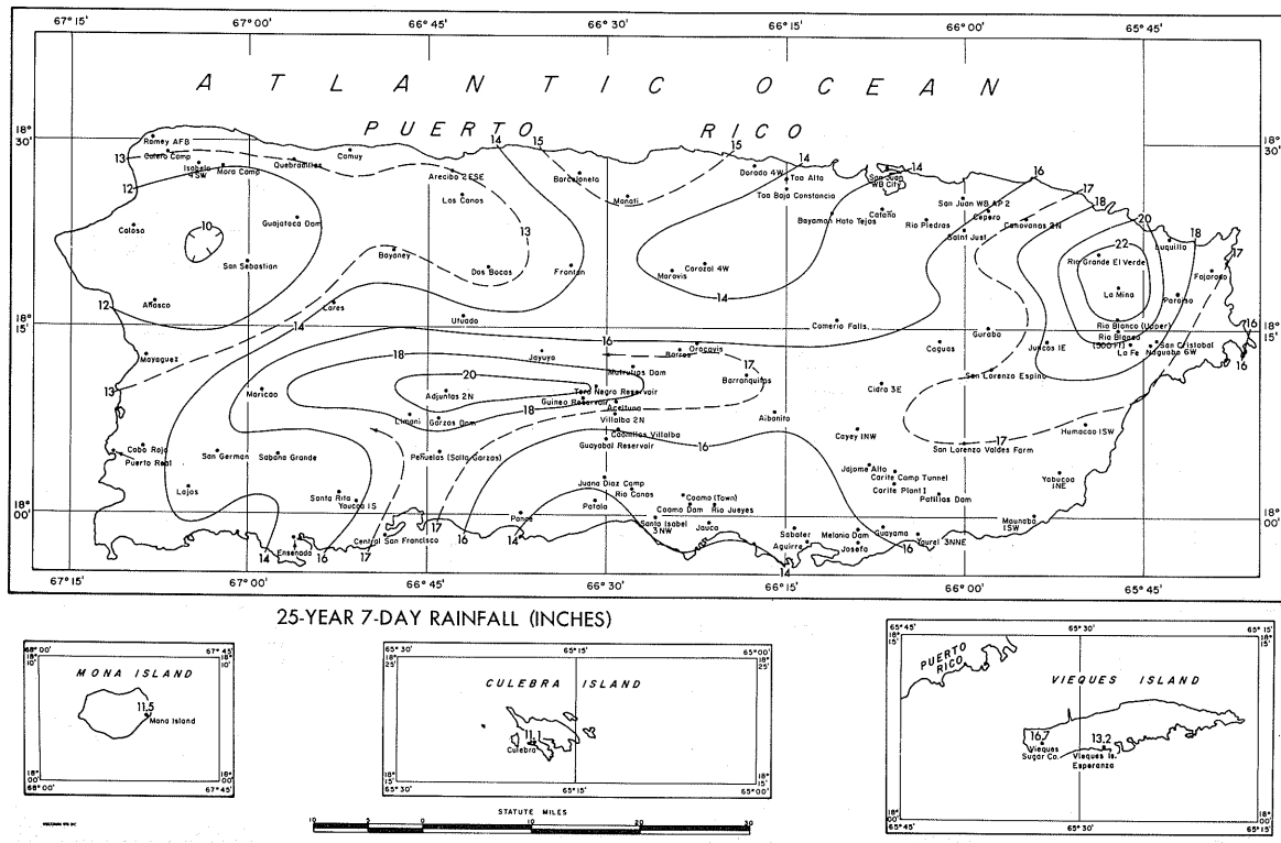
FIGURE 26.—25-year 7-day rainfall (in.) for Puerto Rico.
