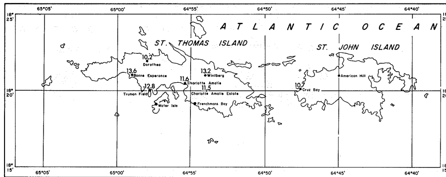
10-YEAR 10-DAY RAINFALL (INCHES)
