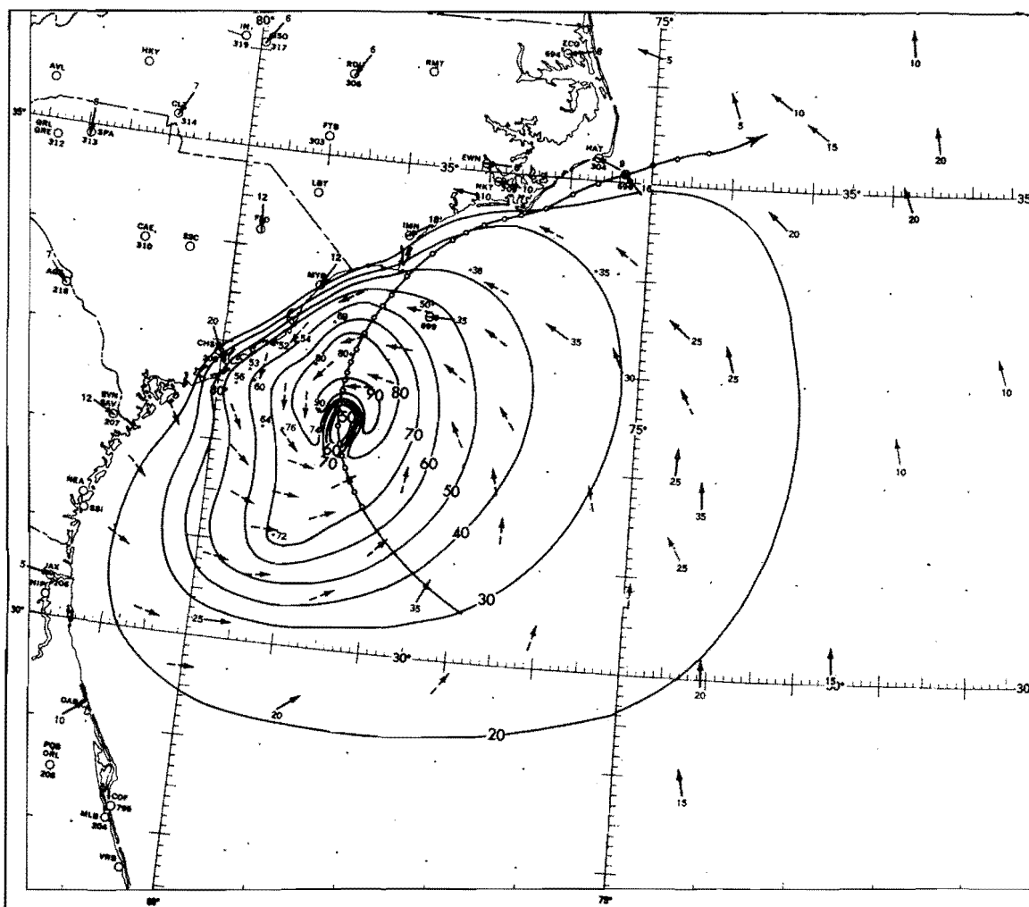
Figure 10.--Wind field (kt) of Hurricane Helene, 1100 EST, Sept. 27, 1958, from Schauss (1962, fig. 12a).
