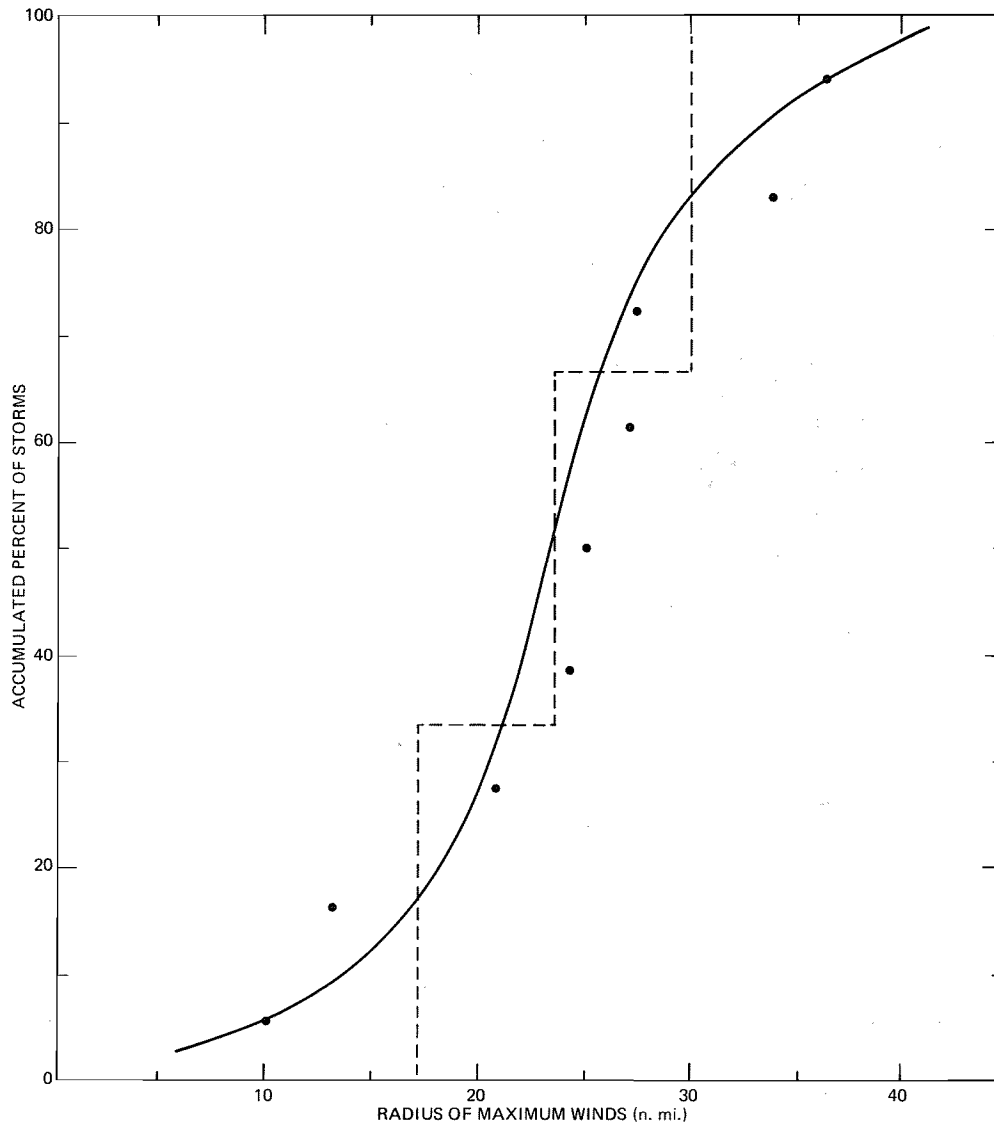
Figure 11.--Probability distribution of radius of maximum winds of hurricanes, Charleston, S.C., zone, 1900-1973.
