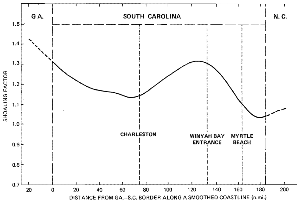
Figure 19.--Shoaling factor, South Carolina coast, Adapted from Barrientos and Jelesnianski (unpublished).
