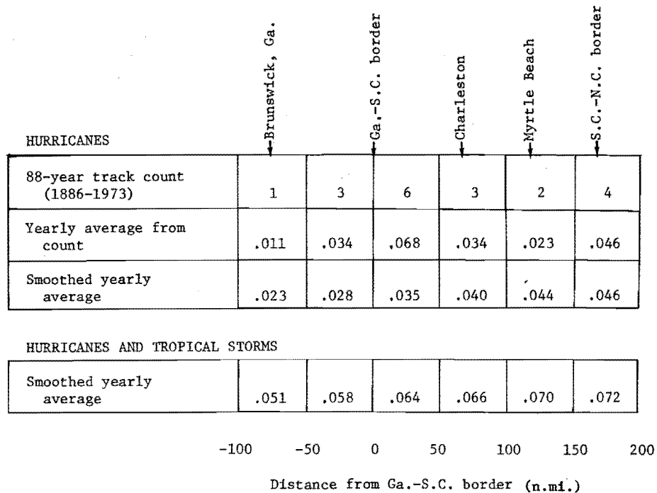
Figure 6.--Landfalling frequency of hurricanes and tropical storms per 50 n.mi. of coast. Track count from track maps by Cry (1965) and the Monthly Weather Review. Smoothed averages from graphs by Ho et al. (1975).
