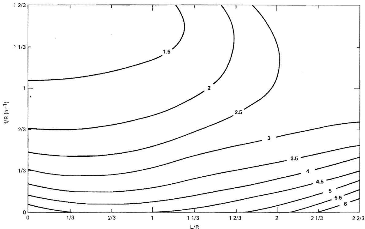
Figure 22.--Time scale factor ( t_{2/3} in hr) for storm surge, alongshore hurricanes, as function of storm surge speed, and distance of path from coast.
