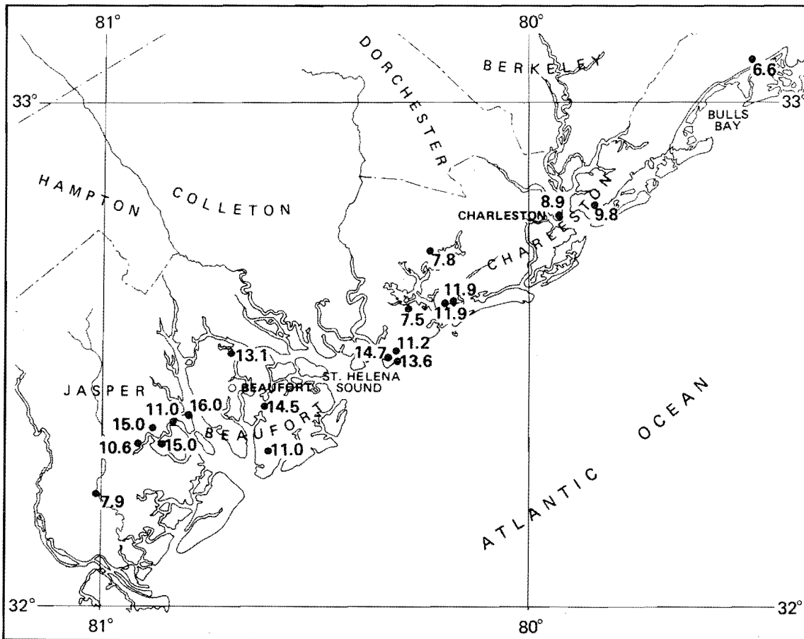
Figure 5.--High-water marks, hurricane of Aug. 11, 1940, obtained by National Ocean Survey field party in 1971 (ft above National Geodetic Vertical Datum of 1929).
