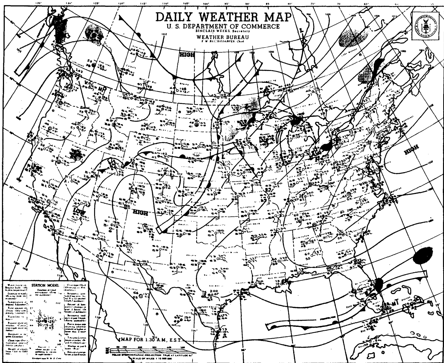
Figure 7-5a.--Surface weather analysis 0030 CST, October 9, 1954.
